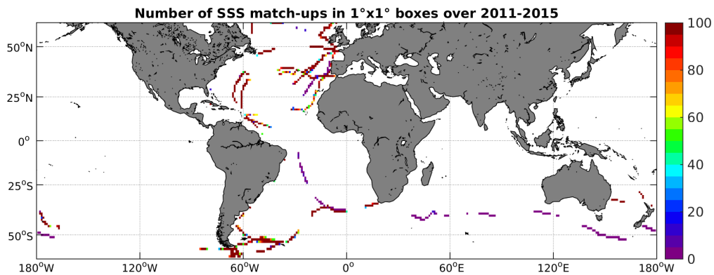
Figure 4: Number of SSS match-ups between TSG-GOSUD-Sailing-ship SSS and the Aquarius-L3-JPL-V4-7DAY-RUNNING SSS product for the SMOS coastal zone ( \pm 800\text{km} ) 60N-60S Pi-MEP region over 1^\circ \times 1^\circ boxes and for the full satellite product period.
