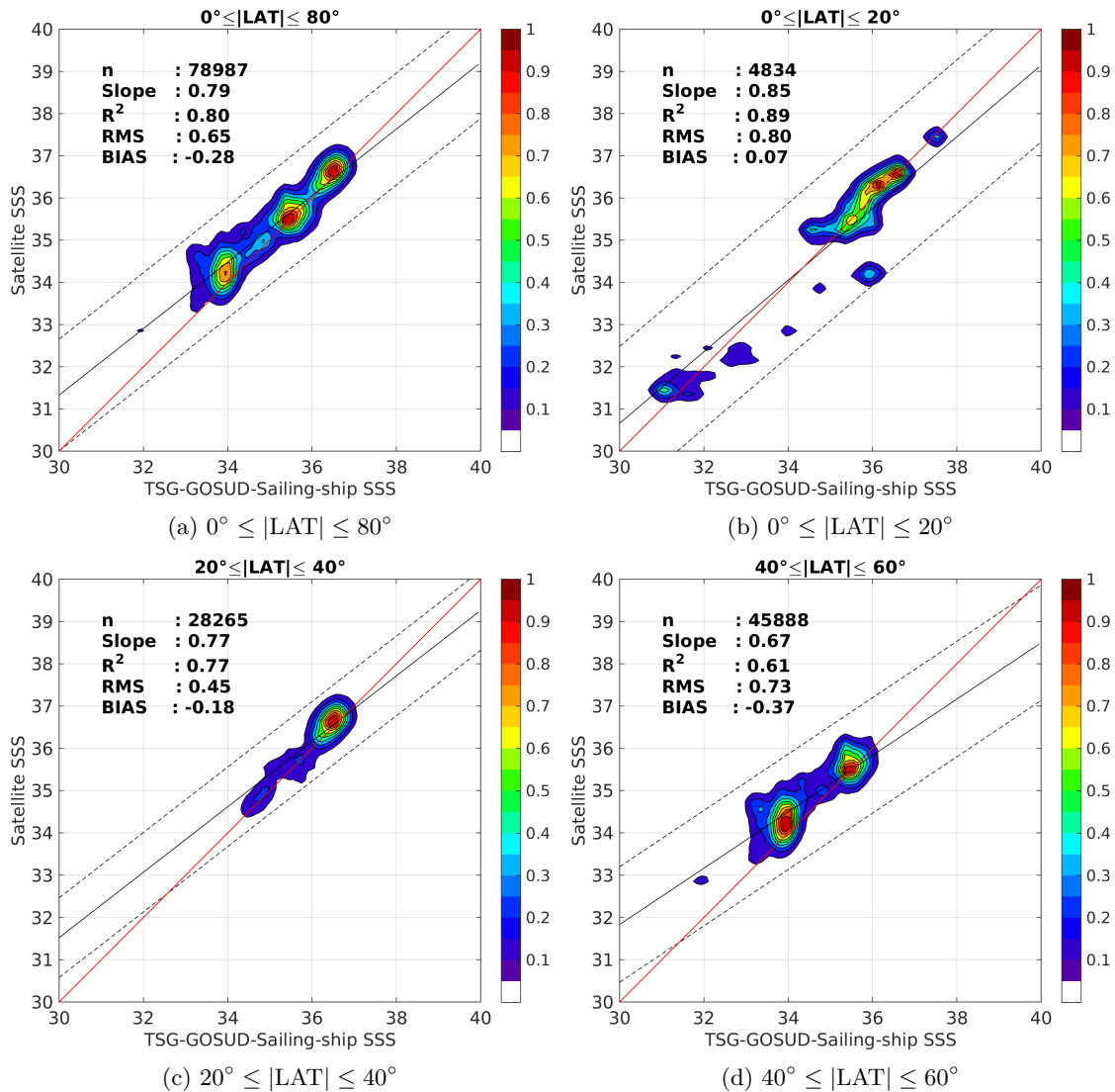
Figure 9: Contour maps of the concentration of Aquarius-L3-JPL-V4-7DAY-RUNNING SSS (y-axis) versus TSG-GOSUD-Sailing-ship SSS (x-axis) at match-up pairs for different latitude bands. For each plot, the red line shows x=y . The black thin and dashed lines indicate a linear fit through the data cloud and the \pm 95\% confidence levels, respectively. The number match-up pairs n , the slope and R^2 coefficient of the linear fit, the root mean square (RMS) and the mean bias between satellite and in situ data are indicated for each latitude band in each plots.
