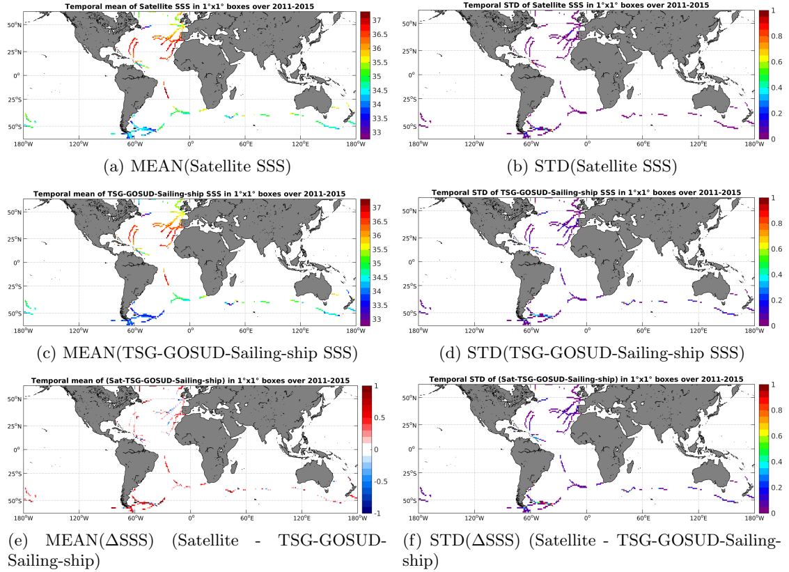
Figure 6: Temporal mean (left) and STD (right) of SSS from Aquarius-L3-JPL-V4-7DAY-RUNNING (top), TSG-GOSUD-Sailing-ship (middle), and of \Delta SSS (Satellite - TSG-GOSUD-Sailing-ship). Only match-up pairs are used to generate these maps.
