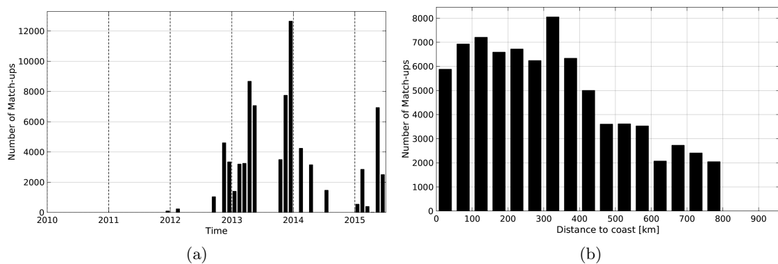
Figure 1: Number of match-ups between TSG-GOSUD-Sailing-ship and Aquarius-L3-JPL-V4-7DAY-RUNNING SSS as a function of time (a) and as function of the distance to coast (b) over the SMOS coastal zone ( \pm 800\text{km} ) 60N-60S Pi-MEP region and for the full satellite product period.
