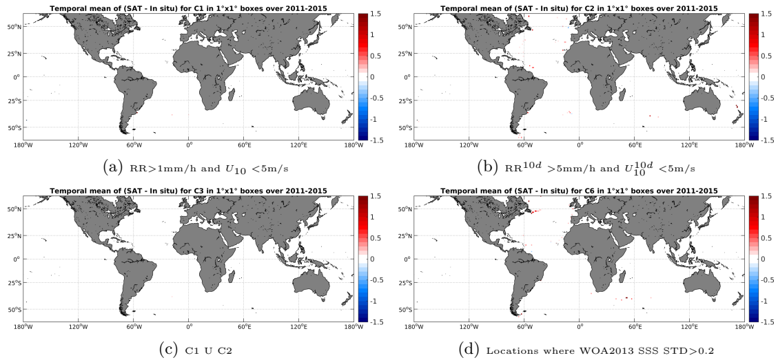
Figure 12: Temporal mean gridded over spatial boxes of size 1^\circ \times 1^\circ of \Delta SSS (Aquarius-L3-JPL-V4-7DAY-RUNNING - TSG-GOSUD-Sailing-ship) for 4 different subdatasets corresponding to: RR > 1\text{mm/h} and U_{10} < 5\text{m/s} (a), RR^{10d} > 5\text{mm/h} and U_{10}^{10d} < 5\text{m/s} (b), C1 U C2 (c), Locations where WOA2013 SSS STD > 0.2 (d).
