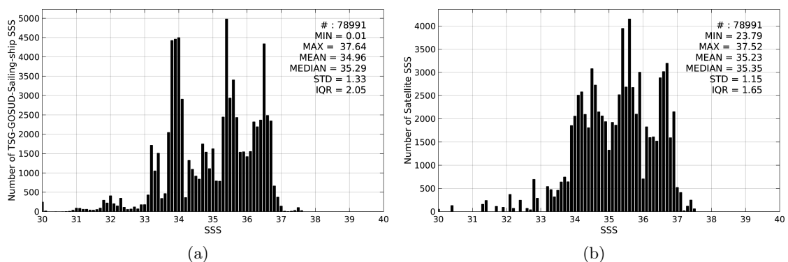
Figure 2: Histograms of SSS from TSG-GOSUD-Sailing-ship (a) and Aquarius-L3-JPL-V4-7DAY-RUNNING (b) considering all match-up pairs per bins of 0.1 over the SMOS coastal zone ( \pm 800\text{km} ) 60N-60S Pi-MEP region and for the full satellite product period.
