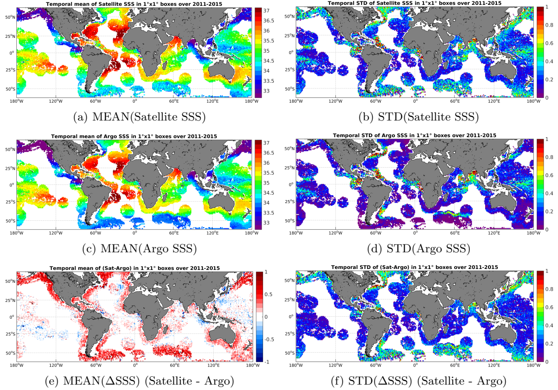
Figure 6: Temporal mean (left) and STD (right) of SSS from Aquarius-L3-JPL-V4-7DAY-RUNNING (top), Argo (middle), and of \Delta SSS (Satellite - Argo). Only match-up pairs are used to generate these maps.
