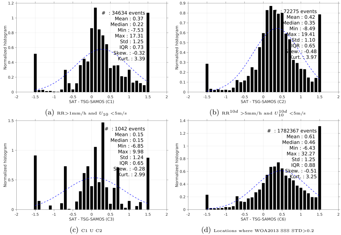
Figure 13: Normalized histogram of \Delta\text{SSS} (Aquarius-L3-JPL-V4-MONTHLY - TSG-SAMOS) for 6 different subdatasets corresponding to: RR > 1mm/h and U_{10} < 5\text{m/s} (a), RR^{10d} > 5\text{mm/h} and U_{10}^{10d} < 5\text{m/s} (b), C1 U C2 (c), Locations where WOA2013 SSS STD > 0.2 (d).
