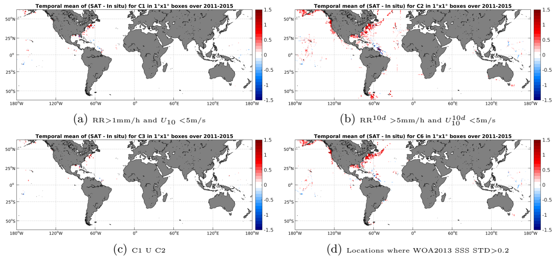
Figure 12: Temporal mean gridded over spatial boxes of size 1^\circ \times 1^\circ of \Delta SSS (Aquarius-L3-JPL-V4-MONTHLY - TSG-SAMOS) for 4 different subdatasets corresponding to: RR > 1\text{mm/h} and U_{10} < 5\text{m/s} (a), RR^{10d} > 5\text{mm/h} and U_{10}^{10d} < 5\text{m/s} (b), C1 U C2 (c), Locations where WOA2013 SSS STD > 0.2 (d).
