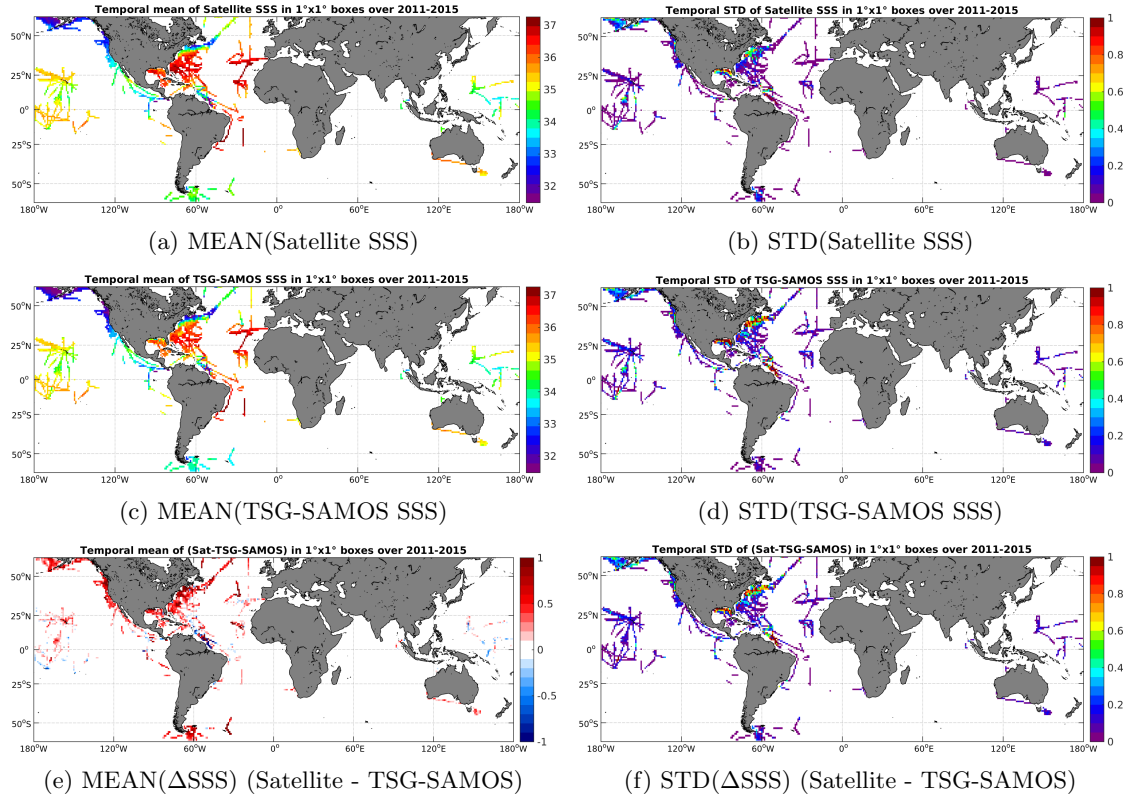
Figure 6: Temporal mean (left) and STD (right) of SSS from Aquarius-L3-JPL-V4-MONTHLY (top), TSG-SAMOS (middle), and of \Delta SSS (Satellite - TSG-SAMOS). Only match-up pairs are used to generate these maps.
