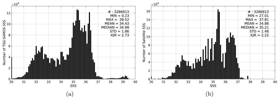
Figure 2: Histograms of SSS from TSG-SAMOS (a) and Aquarius-L3-JPL-V4-MONTHLY (b) considering all match-up pairs per bins of 0.1 over the SMOS coastal zone ( \geq 800 km) 60N-60S Pi-MEP region and for the full satellite product period.
