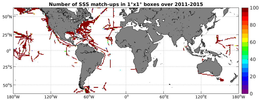
Figure 4: Number of SSS match-ups between TSG-SAMOS SSS and the Aquarius-L3-JPL-V4-MONTHLY SSS product for the SMOS coastal zone ( \approx 800\text{km} ) 60N-60S Pi-MEP region over 1^\circ \times 1^\circ boxes and for the full satellite product period.
