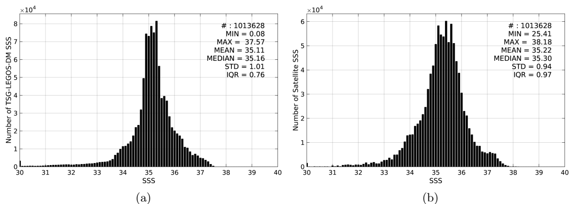
Figure 2: Histograms of SSS from TSG-LEGOS-DM (a) and Aquarius-L3-JPL-V4-MONTHLY (b) considering all match-up pairs per bins of 0.1 over the SMOS coastal zone ( \approx 800 km) 60N-60S Pi-MEP region and for the full satellite product period.
