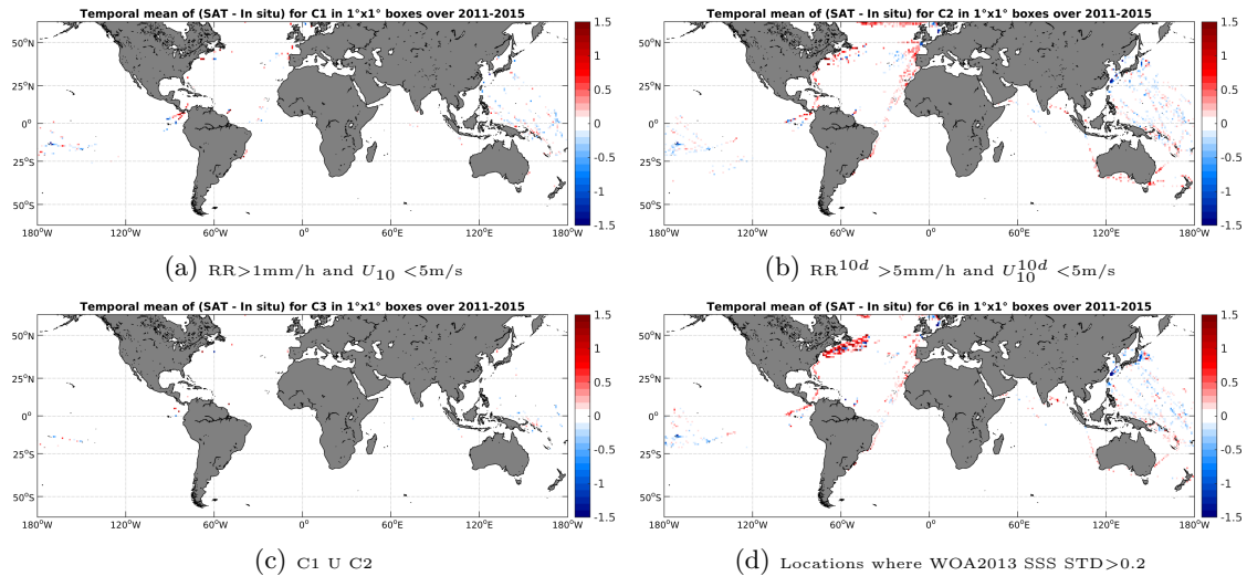
Figure 12: Temporal mean gridded over spatial boxes of size 1^\circ \times 1^\circ of \Delta SSS (Aquarius-L3-JPL-V4-MONTHLY - TSG-LEGOS-DM) for 4 different subdatasets corresponding to: RR > 1\text{mm/h} and U_{10} < 5\text{m/s} (a), RR^{10d} > 5\text{mm/h} and U_{10}^{10d} < 5\text{m/s} (b), C1 U C2 (c), Locations where WOA2013 SSS STD > 0.2 (d).
