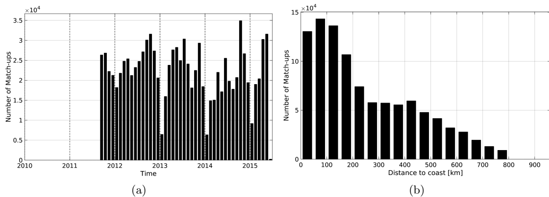
Figure 1: Number of match-ups between TSG-LEGOS-DM and Aquarius-L3-JPL-V4-MONTHLY SSS as a function of time (a) and as function of the distance to coast (b) over the SMOS coastal zone ( \approx 800 km) 60N-60S Pi-MEP region and for the full satellite product period.
