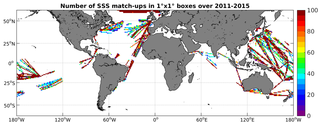
Figure 4: Number of SSS match-ups between TSG-LEGOS-DM SSS and the Aquarius-L3-JPL-V4-MONTHLY SSS product for the SMOS coastal zone ( \pm 800\text{km} ) 60N-60S Pi-MEP region over 1^\circ \times 1^\circ boxes and for the full satellite product period.
