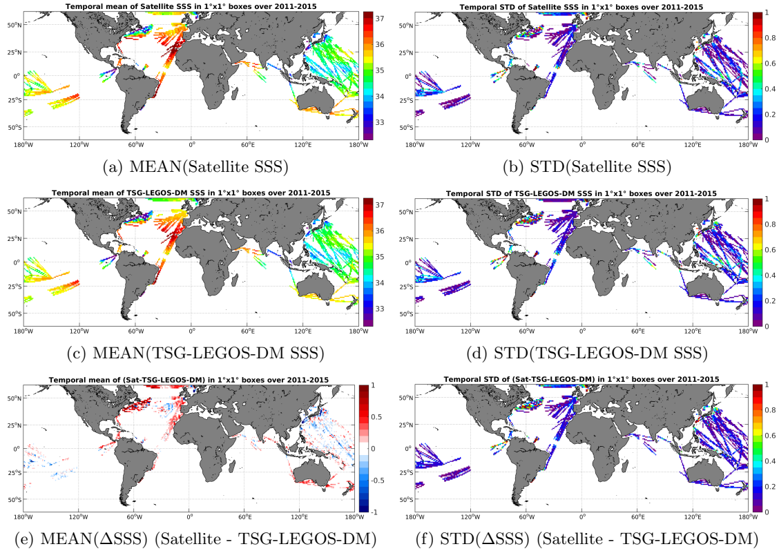
Figure 6: Temporal mean (left) and STD (right) of SSS from Aquarius-L3-JPL-V4-MONTHLY (top), TSG-LEGOS-DM (middle), and of \Delta SSS (Satellite - TSG-LEGOS-DM). Only match-up pairs are used to generate these maps.
