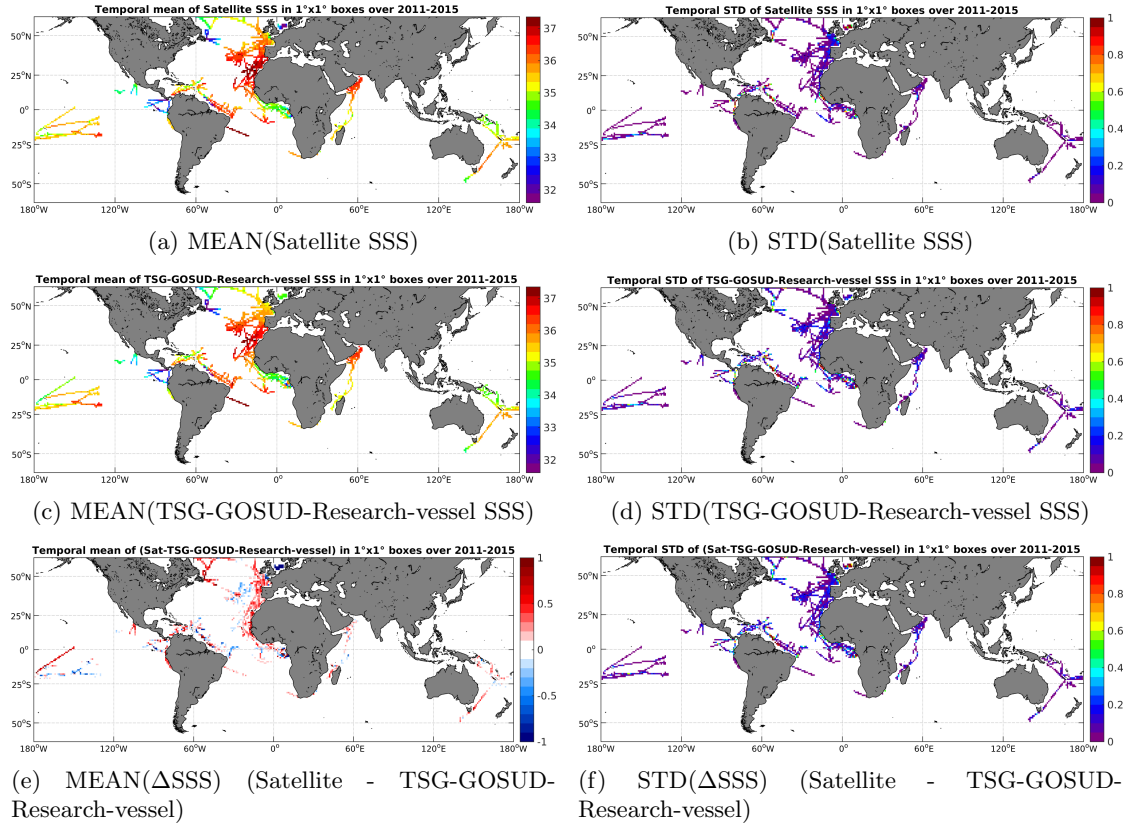
Figure 6: Temporal mean (left) and STD (right) of SSS from Aquarius-L3-JPL-V4-MONTHLY (top), TSG-GOSUD-Research-vessel (middle), and of \Delta SSS (Satellite - TSG-GOSUD-Research-vessel). Only match-up pairs are used to generate these maps.
