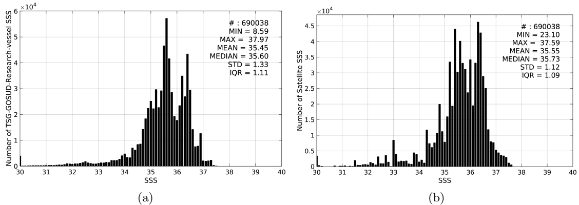
Figure 2: Histograms of SSS from TSG-GOSUD-Research-vessel (a) and Aquarius-L3-JPL-V4-MONTHLY (b) considering all match-up pairs per bins of 0.1 over the SMOS coastal zone ( \pm 800\text{km} ) 60N-60S Pi-MEP region and for the full satellite product period.
