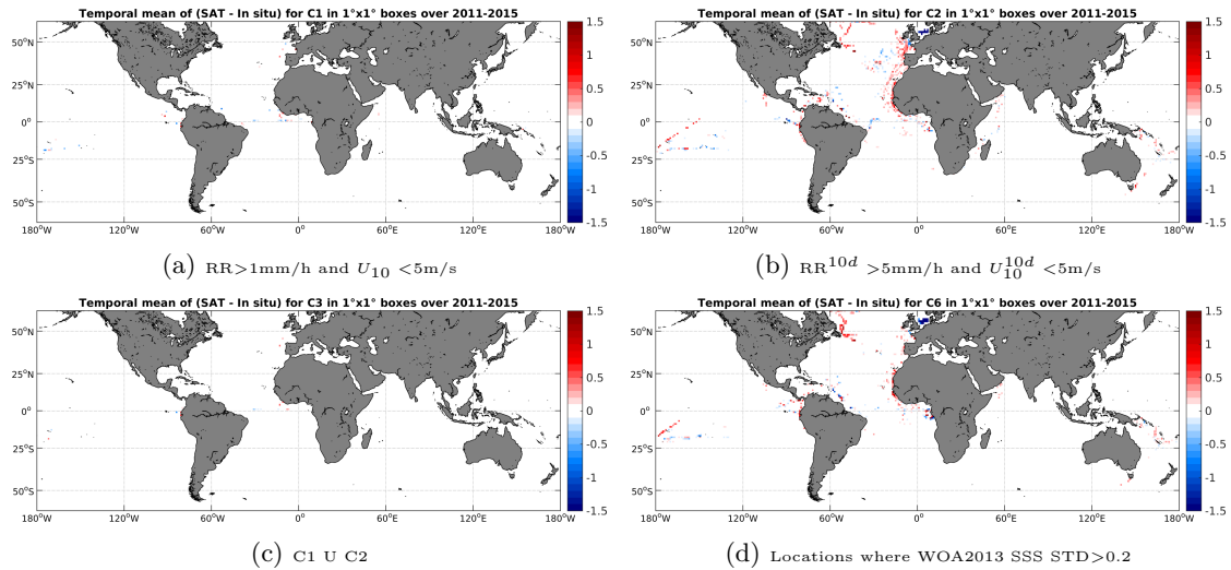
Figure 12: Temporal mean gridded over spatial boxes of size 1^\circ \times 1^\circ of \Delta SSS (Aquarius-L3-JPL-V4-MONTHLY - TSG-GOSUD-Research-vessel) for 4 different subdatasets corresponding to: RR > 1\text{mm/h} and U_{10} < 5\text{m/s} (a), RR^{10d} > 5\text{mm/h} and U_{10}^{10d} < 5\text{m/s} (b), C1 U C2 (c), Locations where WOA2013 SSS STD > 0.2 (d).
