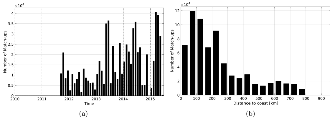
Figure 1: Number of match-ups between TSG-GOSUD-Research-vessel and Aquarius-L3-JPL-V4-MONTHLY SSS as a function of time (a) and as function of the distance to coast (b) over the SMOS coastal zone ( \pm 800 km) 60N-60S Pi-MEP region and for the full satellite product period.
