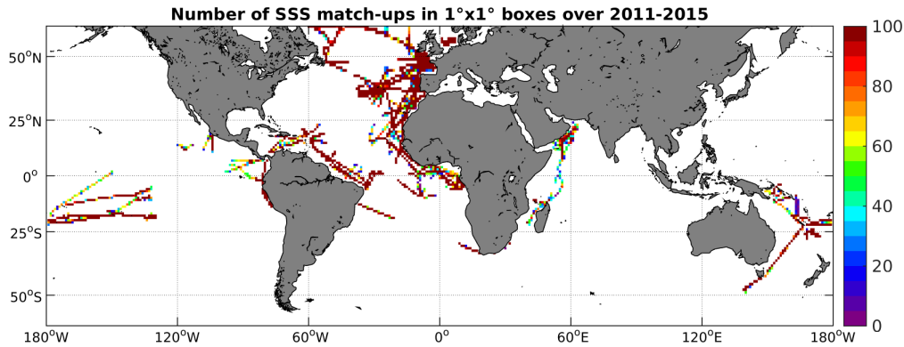
Figure 4: Number of SSS match-ups between TSG-GOSUD-Research-vessel SSS and the Aquarius-L3-JPL-V4-MONTHLY SSS product for the SMOS coastal zone ( \approx 800\text{km} ) 60N-60S Pi-MEP region over 1^\circ \times 1^\circ boxes and for the full satellite product period.
