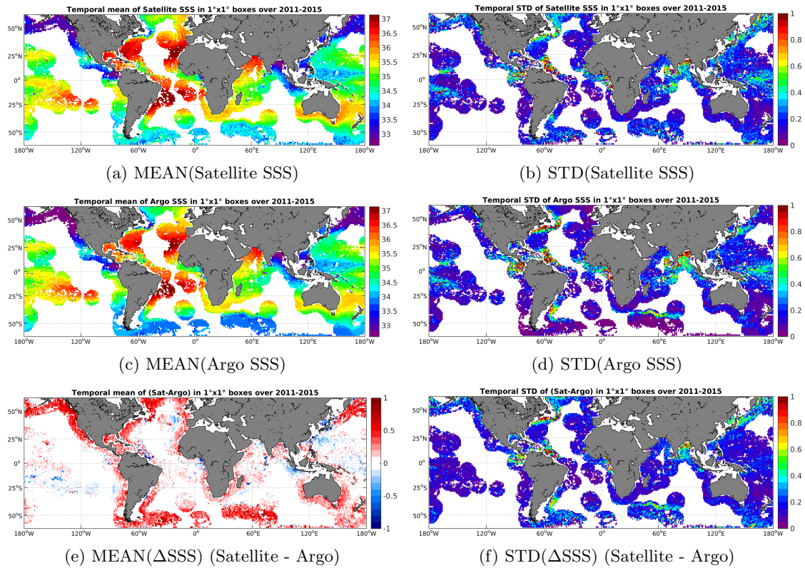
Figure 6: Temporal mean (left) and STD (right) of SSS from Aquarius-L3-JPL-V4-MONTHLY (top), Argo (middle), and of \Delta SSS (Satellite - Argo). Only match-up pairs are used to generate these maps.
