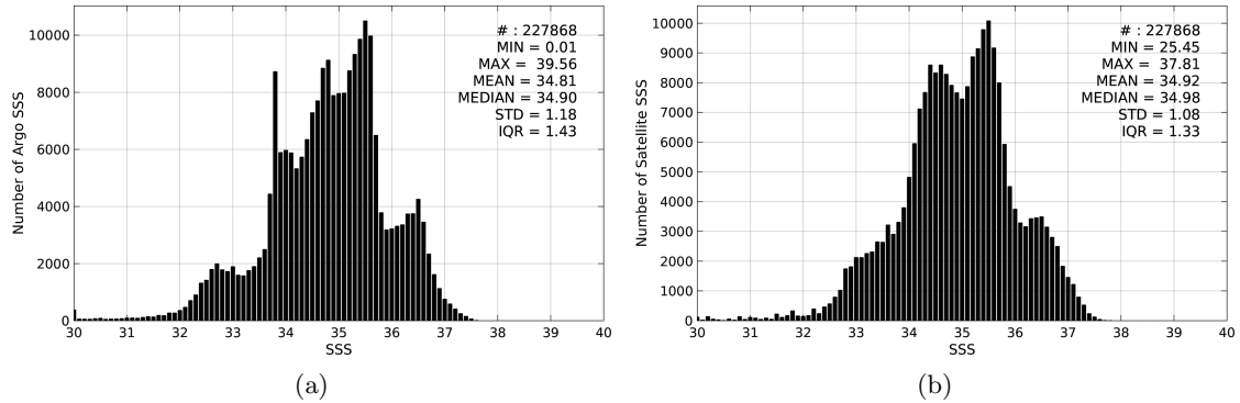
Figure 2: Histograms of SSS from Argo (a) and Aquarius-L3-JPL-V4-MONTHLY (b) considering all match-up pairs per bins of 0.1 over the SMOS coastal zone ( \pm 800\text{km} ) 60N-60S Pi-MEP region and for the full satellite product period.
