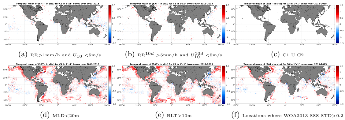
Figure 12: Temporal mean gridded over spatial boxes of size 1^\circ \times 1^\circ of \Delta SSS (Aquarius-L3-JPL-V4-MONTHLY - Argo) for 6 different subdatasets corresponding to:RR > 1 mm/h and U_{10} < 5 m/s (a), RR ^{10d} > 5 mm/h and U_{10}^{10d} < 5 m/s (b), C1 U C2 (c),MLD < 20 m (d),BLT > 10 m (e),Locations where WOA2013 SSS STD > 0.2 (f).
