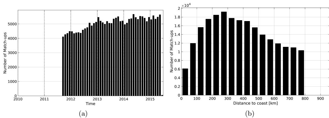
Figure 1: Number of match-ups between Argo and Aquarius-L3-JPL-V4-MONTHLY SSS as a function of time (a) and as function of the distance to coast (b) over the SMOS coastal zone ( \pm 800 km) 60N-60S Pi-MEP region and for the full satellite product period.
