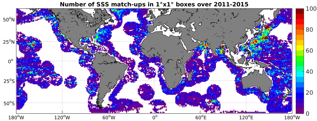
Figure 4: Number of SSS match-ups between Argo SSS and the Aquarius-L3-JPL-V4-MONTHLY SSS product for the SMOS coastal zone ( \approx 800\text{km} ) 60N-60S Pi-MEP region over 1^\circ \times 1^\circ boxes and for the full satellite product period.
