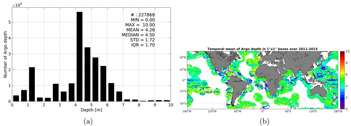
Figure 3: Histograms of the depth of the upper level SSS measurements from Argo in the Match-up DataBase for the SMOS coastal zone ( \pm 800\text{km} ) 60N-60S Pi-MEP region (a) and temporal mean spatial distribution of pressure of the in situ SSS data over 1^\circ \times 1^\circ boxes and for the full satellite product period (b).
