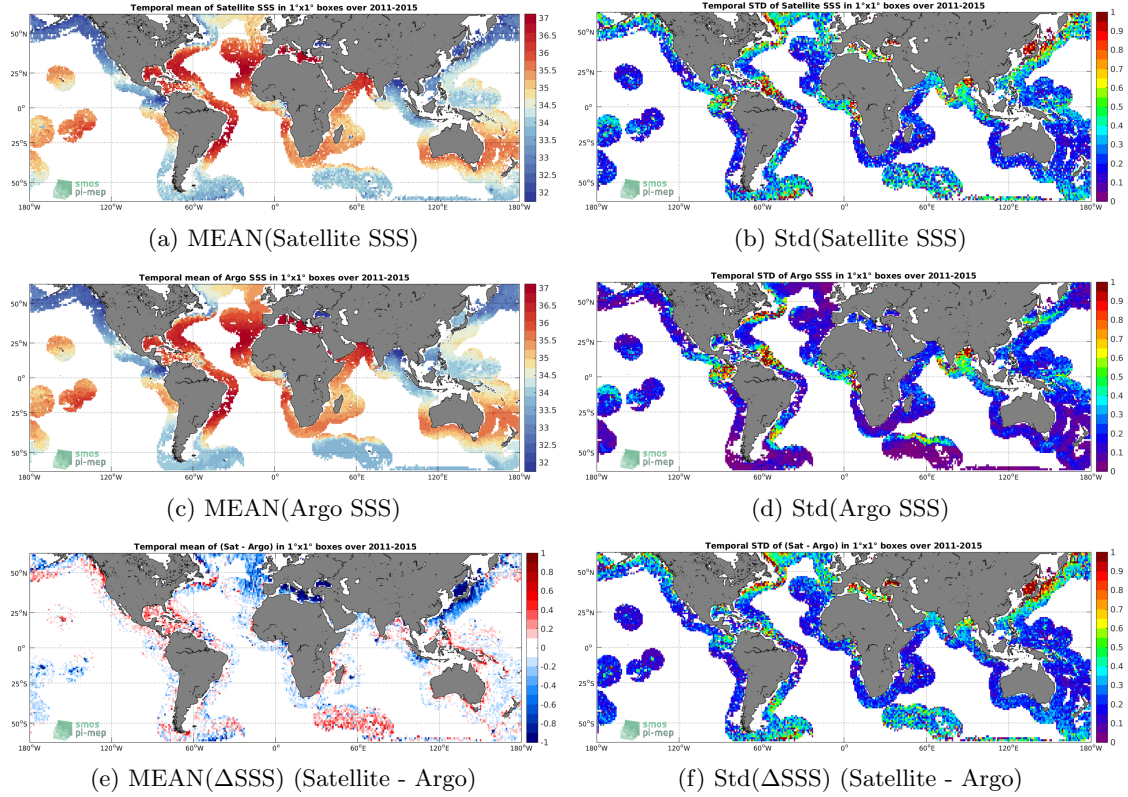
Figure 6: Temporal mean (left) and Std (right) of SSS from Aquarius SSS L2-AVERAGED OR v5 (NASA-GSFC) (top), Argo (middle), and of \Delta SSS (Satellite - Argo). Only match-up pairs are used to generate these maps.
