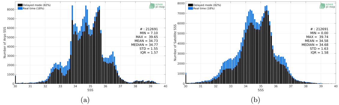
Figure 2: Histograms of SSS from Argo (a) and Aquarius SSS L2-AVERAGED OR v5 (NASA-GSFC) (b) considering all match-up pairs per bins of 0.1 over the SMOS coastal zone (<800km) 60N-60S Pi-MEP region and for the full satellite product period.
