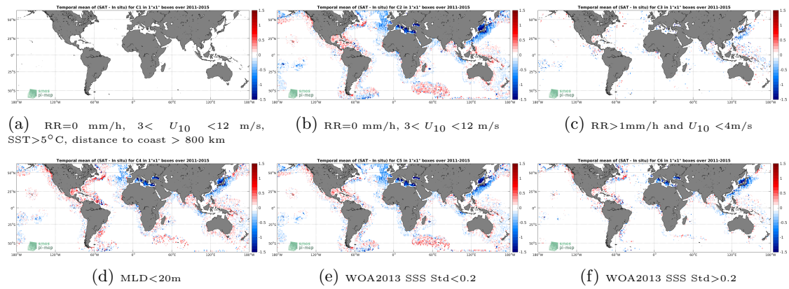
Figure 12: Temporal mean gridded over spatial boxes of size 1^\circ \times 1^\circ of \Delta SSS (Aquarius SSS L2-AVERAGED OR v5 (NASA-GSFC) - Argo) for 6 different subdatasets corresponding to:RR=0 mm/h, 3 < U_{10} < 12 m/s, SST >5^\circ C, distance to coast > 800 km (a), RR=0 mm/h, 3 < U_{10} < 12 m/s (b), RR >1 mm/h and U_{10} < 4 m/s (c),MLD <20 m (d),WOA2013 SSS Std <0.2 (e),WOA2013 SSS Std >0.2 (f).
