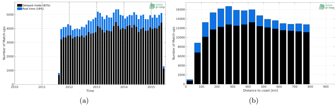
Figure 1: Number of match-ups between Argo and Aquarius SSS L2-AVERAGED OR v5 (NASA-GSFC) SSS as a function of time (a) and as function of the distance to coast (b) over the SMOS coastal zone (<800km) 60N-60S Pi-MEP region and for the full satellite product period.
