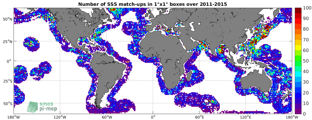
Figure 4: Number of SSS match-ups between Argo SSS and the Aquarius SSS L2-AVERAGED OR v5 (NASA-GSFC) SSS product for the SMOS coastal zone (<800km) 60N-60S Pi-MEP region over 1^{\circ} \times 1^{\circ} boxes and for the full satellite product period.
