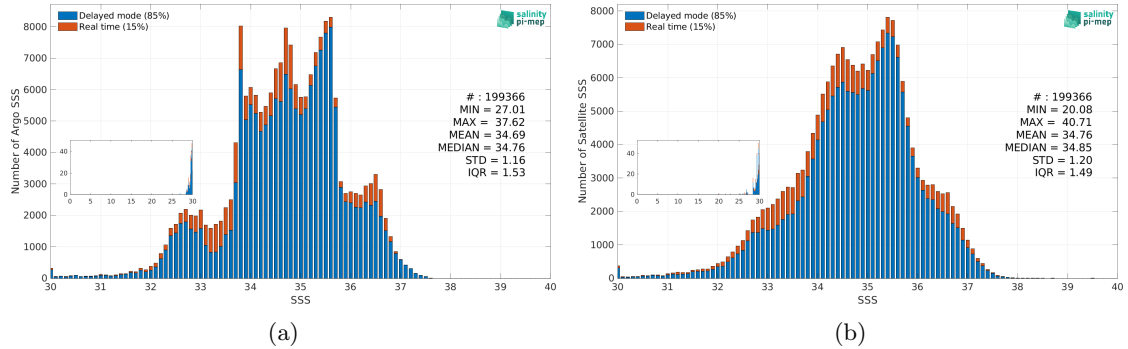
Figure 3: Histograms of SSS from Argo (a) and Aquarius SSS L2-AVERAGED CAP v5 (JPL) (b) considering all match-up pairs per bins of 0.1 over the SMOS coastal zone (<800km) 60N-60S Pi-MEP region and for the full satellite product period.
