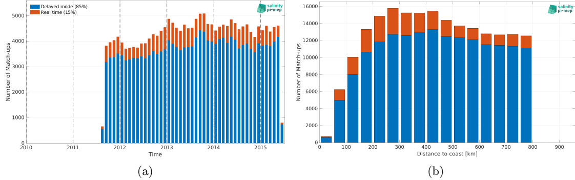
Figure 2: Number of match-ups between Argo and Aquarius SSS L2-AVERAGED CAP v5 (JPL) SSS as a function of time (a) and as function of the distance to coast (b) over the SMOS coastal zone (<800km) 60N-60S Pi-MEP region and for the full satellite product period.
