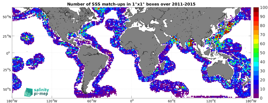
Figure 5: Number of SSS match-ups between Argo SSS and the Aquarius SSS L2-AVERAGED CAP v5 (JPL) SSS product for the SMOS coastal zone (<800km) 60N-60S Pi-MEP region over 1^\circ \times 1^\circ boxes and for the full satellite product period.
