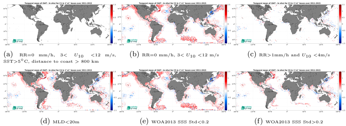
Figure 14: Temporal mean gridded over spatial boxes of size 1^\circ \times 1^\circ of \Delta SSS (Aquarius SSS L2-AVERAGED CAP v5 (JPL) - Argo) for 6 different subdatasets corresponding to:RR=0 mm/h, 3 < U_{10} < 12 m/s, SST >5^\circ C, distance to coast > 800 km (a), RR=0 mm/h, 3 < U_{10} < 12 m/s (b), RR >1 mm/h and U_{10} < 4 m/s (c),MLD <20 m (d),WOA2013 SSS Std <0.2 (e),WOA2013 SSS Std >0.2 (f).
