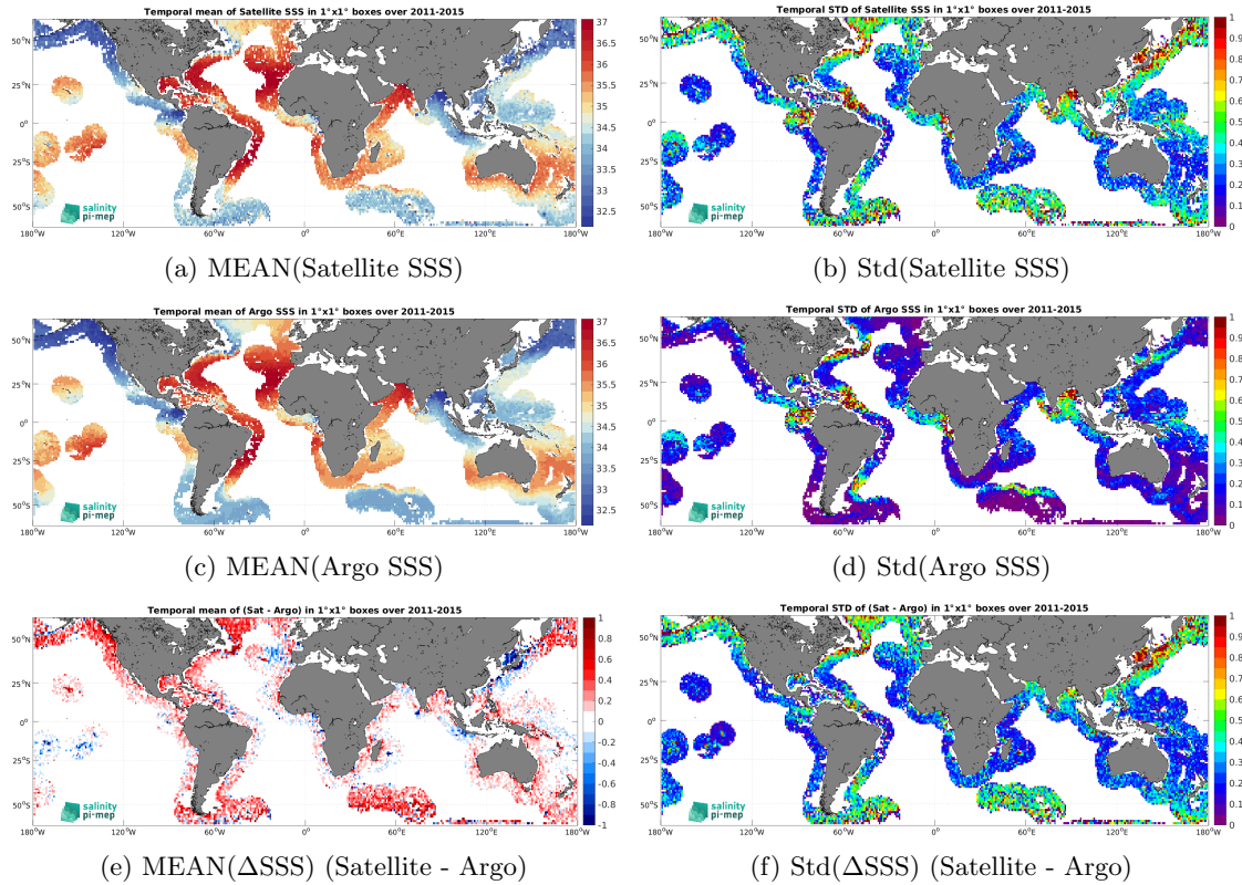
Figure 7: Temporal mean (left) and Std (right) of SSS from Aquarius SSS L2-AVERAGED CAP v5 (JPL) (top), Argo (middle), and of \Delta SSS (Satellite - Argo). Only match-up pairs are used to generate these maps.
