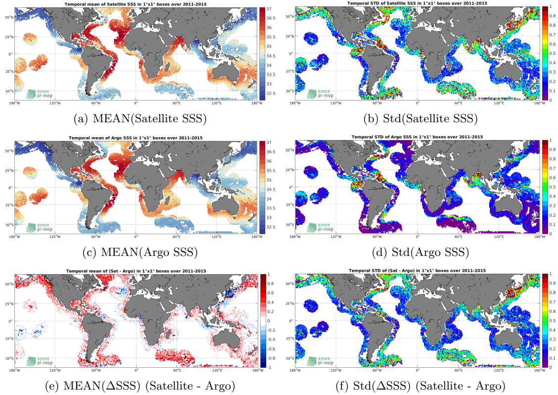
Figure 6: Temporal mean (left) and Std (right) of SSS from Aquarius SSS L2-AVERAGED CAP v5 (JPL) (top), Argo (middle), and of \Delta SSS (Satellite - Argo). Only match-up pairs are used to generate these maps.
