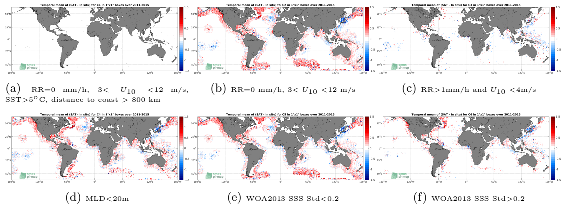
Figure 12: Temporal mean gridded over spatial boxes of size 1^\circ \times 1^\circ of \Delta SSS (Aquarius SSS L2-AVERAGED CAP v5 (JPL) - Argo) for 6 different subdatasets corresponding to:RR=0 mm/h, 3 < U_{10} < 12 m/s, SST >5^\circ C, distance to coast > 800 km (a), RR=0 mm/h, 3 < U_{10} < 12 m/s (b), RR >1 mm/h and U_{10} < 4 m/s (c),MLD <20 m (d),WOA2013 SSS Std <0.2 (e),WOA2013 SSS Std >0.2 (f).
