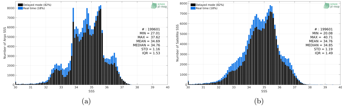
Figure 2: Histograms of SSS from Argo (a) and Aquarius SSS L2-AVERAGED CAP v5 (JPL) (b) considering all match-up pairs per bins of 0.1 over the SMOS coastal zone (<800km) 60N-60S Pi-MEP region and for the full satellite product period.
