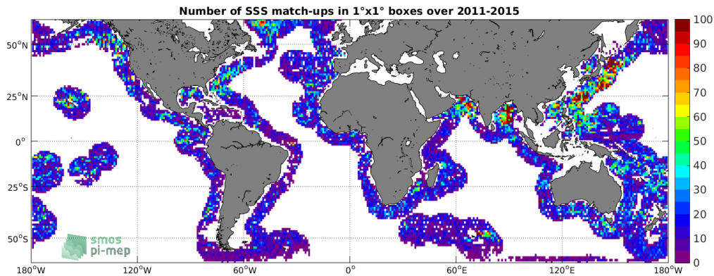
Figure 4: Number of SSS match-ups between Argo SSS and the Aquarius SSS L2-AVERAGED CAP v5 (JPL) SSS product for the SMOS coastal zone (<800km) 60N-60S Pi-MEP region over 1^\circ \times 1^\circ boxes and for the full satellite product period.
