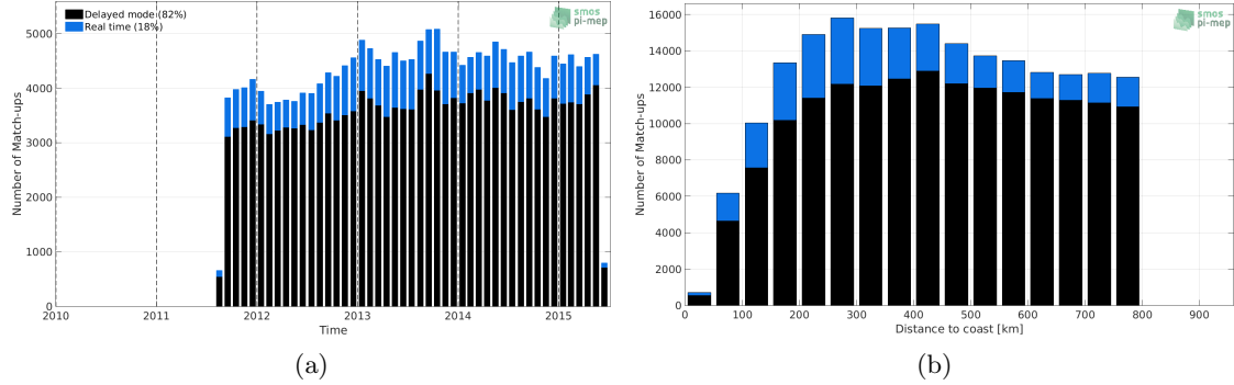
Figure 1: Number of match-ups between Argo and Aquarius SSS L2-AVERAGED CAP v5 (JPL) SSS as a function of time (a) and as function of the distance to coast (b) over the SMOS coastal zone (<800km) 60N-60S Pi-MEP region and for the full satellite product period.
