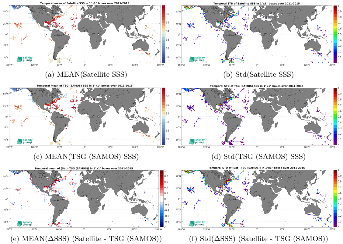
Figure 6: Temporal mean (left) and Std (right) of SSS from Aquarius SSS L2 OR v5 (NASA-GSFC) (top), TSG (SAMOS) (middle), and of \Delta SSS (Satellite - TSG (SAMOS)). Only match-up pairs are used to generate these maps.
