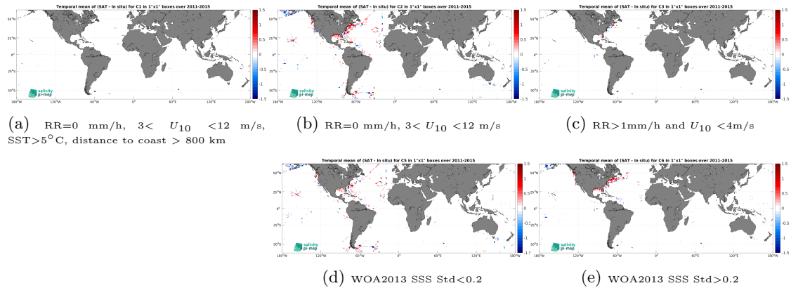
Figure 12: Temporal mean gridded over spatial boxes of size 1^\circ \times 1^\circ of \Delta\text{SSS} (Aquarius SSS L2 OR v5 (NASA-GSFC) - TSG (SAMOS)) for 5 different subdatasets corresponding to:RR=0 mm/h, 3 < U_{10} < 12 m/s, SST >5^\circ\text{C} , distance to coast > 800 km (a), RR=0 mm/h, 3 < U_{10} < 12 m/s (b), RR >1 mm/h and U_{10} < 4 m/s (c), WOA2013 SSS Std <0.2 (d), WOA2013 SSS Std >0.2 (e).
