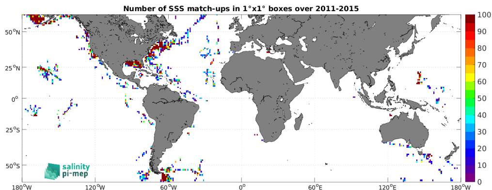
Figure 4: Number of SSS match-ups between TSG (SAMOS) SSS and the Aquarius SSS L2 OR v5 (NASA-GSFC) SSS product for the SMOS coastal zone (<800km) 60N-60S Pi-MEP region over 1^\circ \times 1^\circ boxes and for the full satellite product period.
