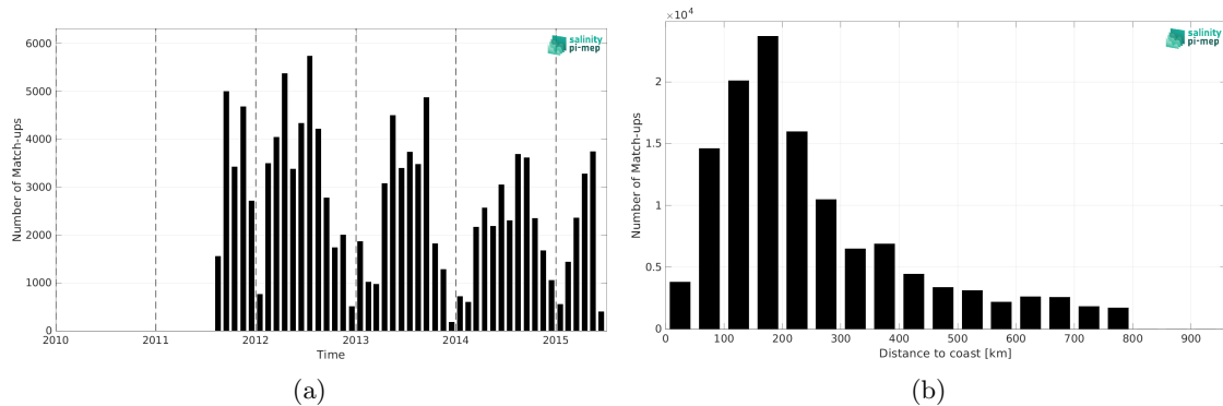
Figure 1: Number of match-ups between TSG (SAMOS) and Aquarius SSS L2 OR v5 (NASA-GSFC) SSS as a function of time (a) and as function of the distance to coast (b) over the SMOS coastal zone (<800km) 60N-60S Pi-MEP region and for the full satellite product period.
