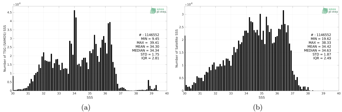
Figure 2: Histograms of SSS from TSG (SAMOS) (a) and Aquarius SSS L2 OR v5 (NASA-GSFC) (b) considering all match-up pairs per bins of 0.1 over the SMOS coastal zone (<800km) 60N-60S Pi-MEP region and for the full satellite product period.
