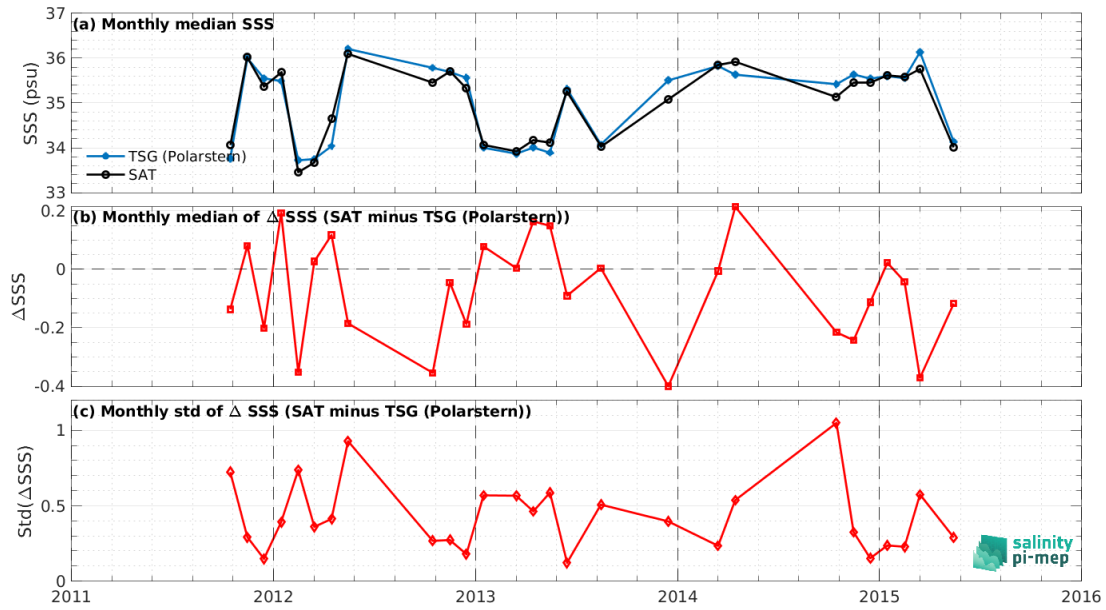
Figure 8: Time series of the monthly median SSS (top), median of \Delta SSS (Satellite - TSG (Polarstern)) and Std of \Delta SSS (Satellite - TSG (Polarstern)) over the SMOS coastal zone ( <800\text{km} ) 60\text{N} - 60\text{S} Pi-MEP region considering all match-ups collected by the Pi-MEP.
