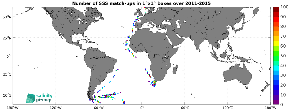
Figure 5: Number of SSS match-ups between TSG (Polarstern) SSS and the Aquarius SSS L2 OR v5 (NASA-GSFC) SSS product for the SMOS coastal zone (<800km) 60N-60S Pi-MEP region over 1^\circ \times 1^\circ boxes and for the full satellite product period.
