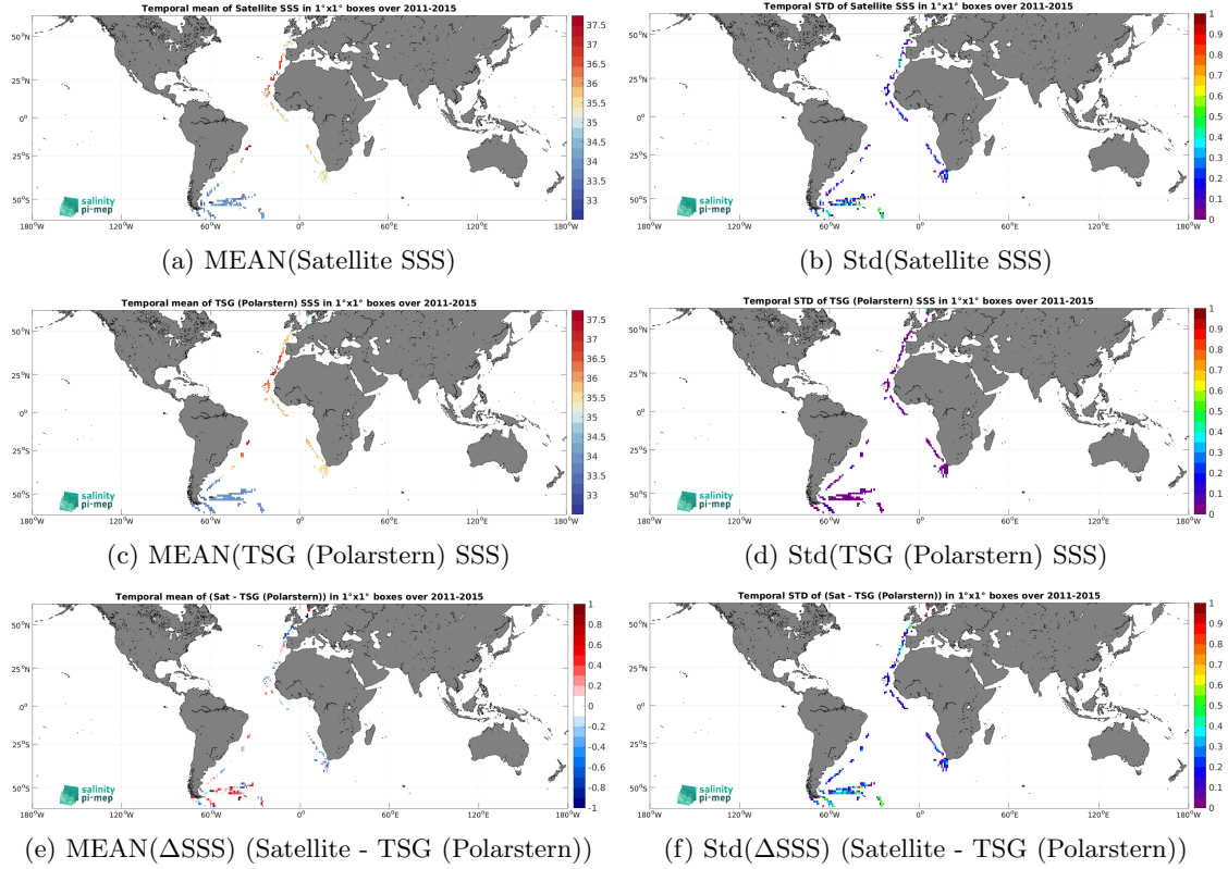
Figure 7: Temporal mean (left) and Std (right) of SSS from Aquarius SSS L2 OR v5 (NASA-GSFC) (top), TSG (Polarstern) (middle), and of \Delta SSS (Satellite - TSG (Polarstern)). Only match-up pairs are used to generate these maps.
