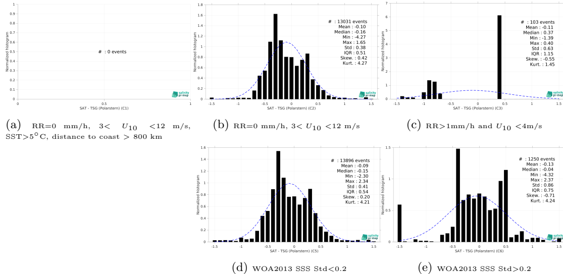
Figure 15: Normalized histogram of \Delta\text{SSS} (Aquarius SSS L2 OR v5 (NASA-GSFC) - TSG (Polarstern)) for 5 different subdatasets corresponding to: RR=0 mm/h, 3 < U_{10} < 12 m/s, SST > 5^{\circ}\text{C} , distance to coast > 800 km (a), RR=0 mm/h, 3 < U_{10} < 12 m/s (b), RR > 1\text{mm/h} and U_{10} < 4\text{m/s} (c), WOA2013 SSS Std < 0.2 (d), WOA2013 SSS Std > 0.2 (e).
