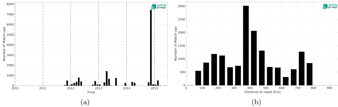
Figure 2: Number of match-ups between TSG (Polarstern) and Aquarius SSS L2 OR v5 (NASA-GSFC) SSS as a function of time (a) and as function of the distance to coast (b) over the SMOS coastal zone (<800km) 60N-60S Pi-MEP region and for the full satellite product period.
