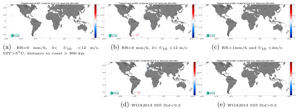
Figure 14: Temporal mean gridded over spatial boxes of size 1^\circ \times 1^\circ of \Delta SSS (Aquarius SSS L2 OR v5 (NASA-GSFC) - TSG (Polarstern)) for 5 different subdatasets corresponding to: RR=0 mm/h, 3 < U_{10} < 12 m/s, SST > 5^\circ\text{C} , distance to coast > 800 km (a), RR=0 mm/h, 3 < U_{10} < 12 m/s (b), RR > 1 mm/h and U_{10} < 4 m/s (c), WOA2013 SSS Std < 0.2 (d), WOA2013 SSS Std > 0.2 (e).
