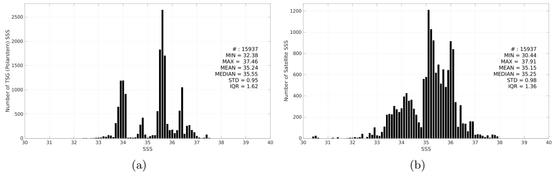
Figure 3: Histograms of SSS from TSG (Polarstern) (a) and Aquarius SSS L2 OR v5 (NASA-GSFC) (b) considering all match-up pairs per bins of 0.1 over the SMOS coastal zone (<800km) 60N-60S Pi-MEP region and for the full satellite product period.
