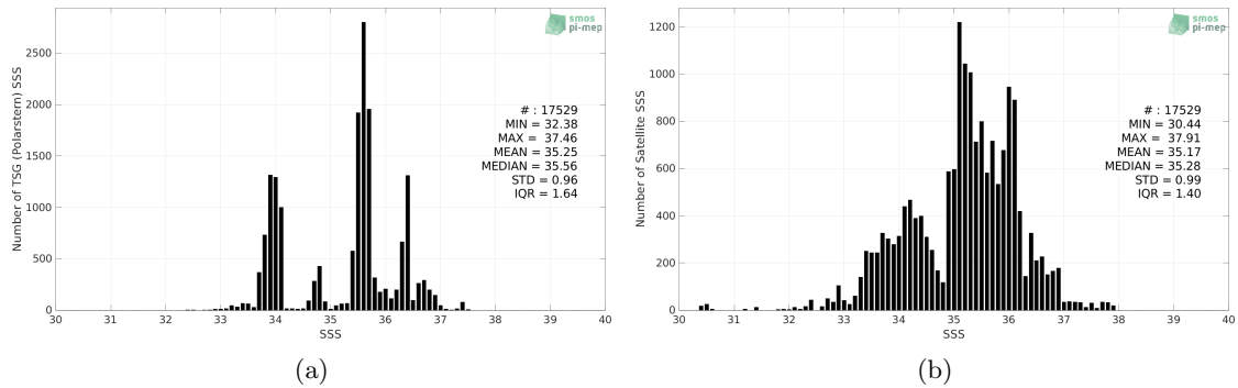
Figure 2: Histograms of SSS from TSG (Polarstern) (a) and Aquarius SSS L2 OR v5 (NASA-GSFC) (b) considering all match-up pairs per bins of 0.1 over the SMOS coastal zone (<800km) 60N-60S Pi-MEP region and for the full satellite product period.
