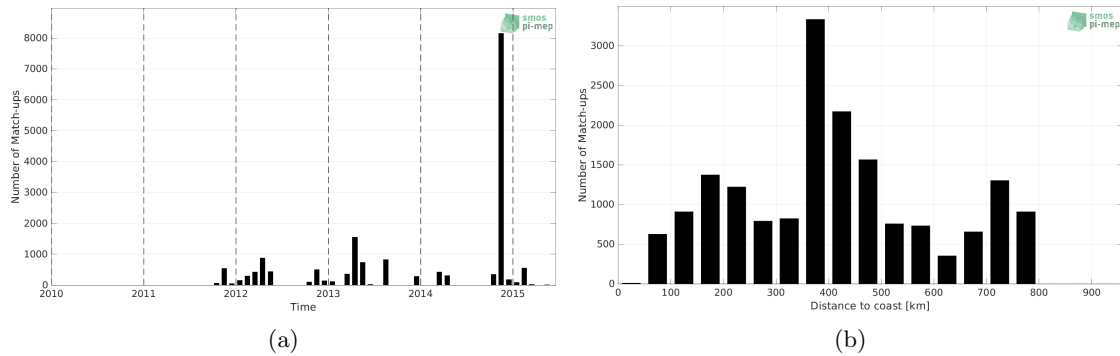
Figure 1: Number of match-ups between TSG (Polarstern) and Aquarius SSS L2 OR v5 (NASA-GSFC) SSS as a function of time (a) and as function of the distance to coast (b) over the SMOS coastal zone (<800km) 60N-60S Pi-MEP region and for the full satellite product period.
