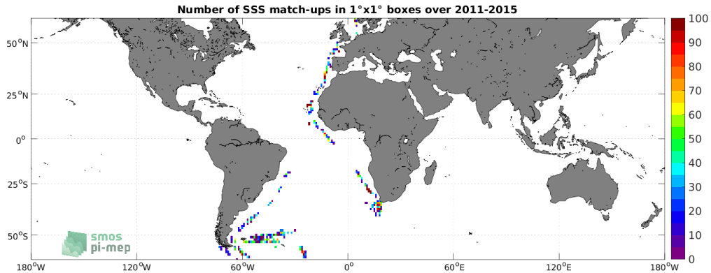
Figure 4: Number of SSS match-ups between TSG (Polarstern) SSS and the Aquarius SSS L2 OR v5 (NASA-GSFC) SSS product for the SMOS coastal zone (<800km) 60N-60S Pi-MEP region over 1^\circ \times 1^\circ boxes and for the full satellite product period.
