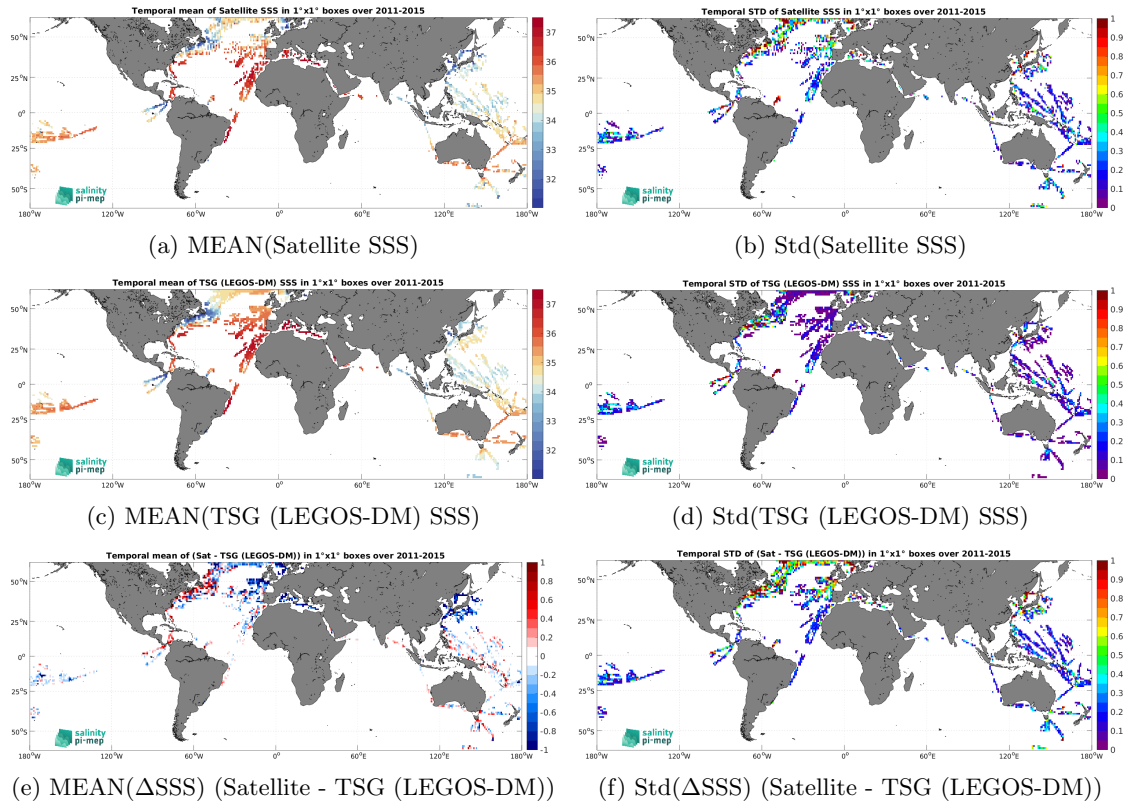
Figure 7: Temporal mean (left) and Std (right) of SSS from Aquarius SSS L2 OR v5 (NASA-GSFC) (top), TSG (LEGOS-DM) (middle), and of \Delta SSS (Satellite - TSG (LEGOS-DM)). Only match-up pairs are used to generate these maps.
