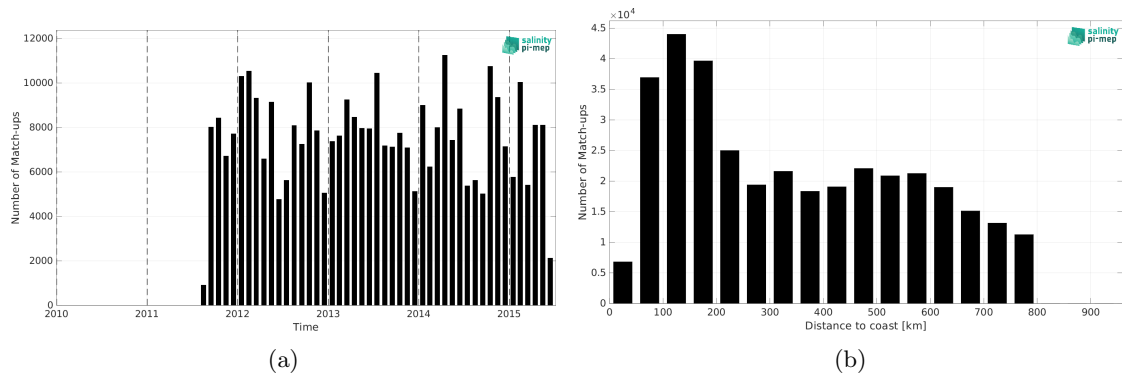
Figure 2: Number of match-ups between TSG (LEGOS-DM) and Aquarius SSS L2 OR v5 (NASA-GSFC) SSS as a function of time (a) and as function of the distance to coast (b) over the SMOS coastal zone (<800km) 60N-60S Pi-MEP region and for the full satellite product period.
