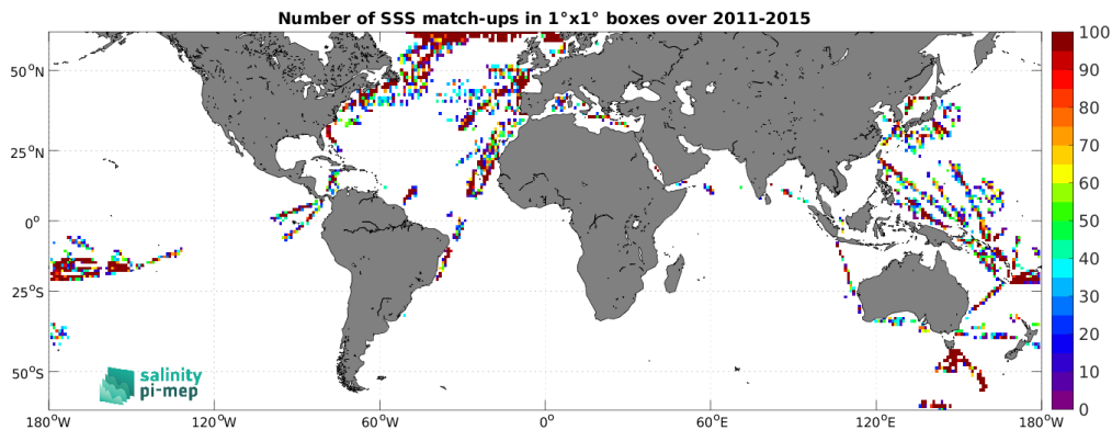
Figure 5: Number of SSS match-ups between TSG (LEGOS-DM) SSS and the Aquarius SSS L2 OR v5 (NASA-GSFC) SSS product for the SMOS coastal zone (<800km) 60N-60S Pi-MEP region over 1^\circ \times 1^\circ boxes and for the full satellite product period.
