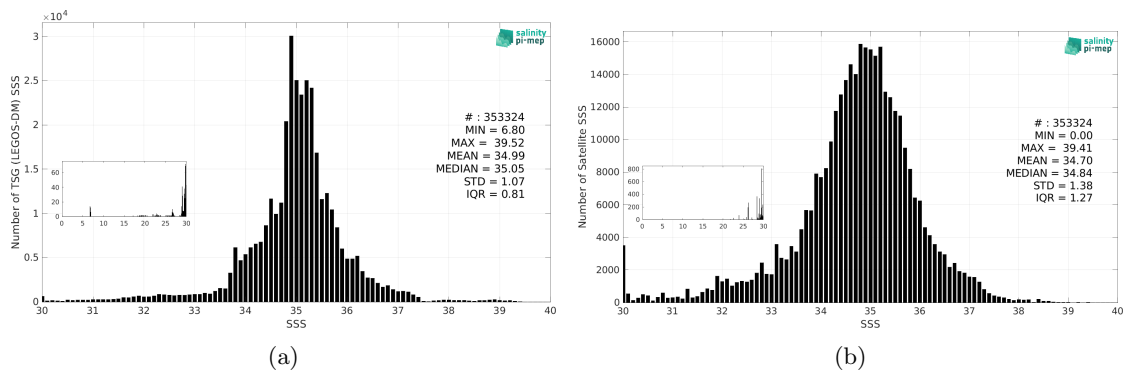
Figure 3: Histograms of SSS from TSG (LEGOS-DM) (a) and Aquarius SSS L2 OR v5 (NASA-GSFC) (b) considering all match-up pairs per bins of 0.1 over the SMOS coastal zone (<800km) 60N-60S Pi-MEP region and for the full satellite product period.
