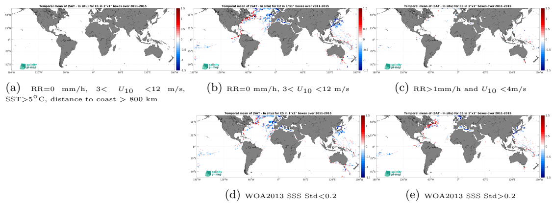
Figure 14: Temporal mean gridded over spatial boxes of size 1^\circ \times 1^\circ of \Delta SSS (Aquarius SSS L2 OR v5 (NASA-GSFC) - TSG (LEGOS-DM)) for 5 different subdatasets corresponding to:RR=0 mm/h, 3 < U_{10} < 12 m/s, SST > 5^\circ\text{C} , distance to coast > 800 km (a), RR=0 mm/h, 3 < U_{10} < 12 m/s (b), RR > 1 mm/h and U_{10} < 4 m/s (c), WOA2013 SSS Std < 0.2 (d), WOA2013 SSS Std > 0.2 (e).
