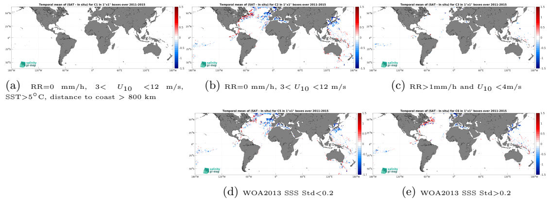
Figure 12: Temporal mean gridded over spatial boxes of size 1^\circ \times 1^\circ of \Delta SSS (Aquarius SSS L2 OR v5 (NASA-GSFC) - TSG (LEGOS-DM)) for 5 different subdatasets corresponding to:RR=0 mm/h, 3 < U_{10} < 12 m/s, SST >5^\circ\text{C} , distance to coast > 800 km (a), RR=0 mm/h, 3 < U_{10} < 12 m/s (b), RR >1 mm/h and U_{10} < 4 m/s (c), WOA2013 SSS Std <0.2 (d), WOA2013 SSS Std >0.2 (e).
