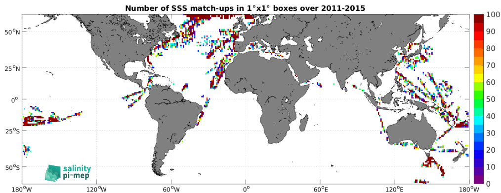
Figure 4: Number of SSS match-ups between TSG (LEGOS-DM) SSS and the Aquarius SSS L2 OR v5 (NASA-GSFC) SSS product for the SMOS coastal zone (<800km) 60N-60S Pi-MEP region over 1^\circ \times 1^\circ boxes and for the full satellite product period.
