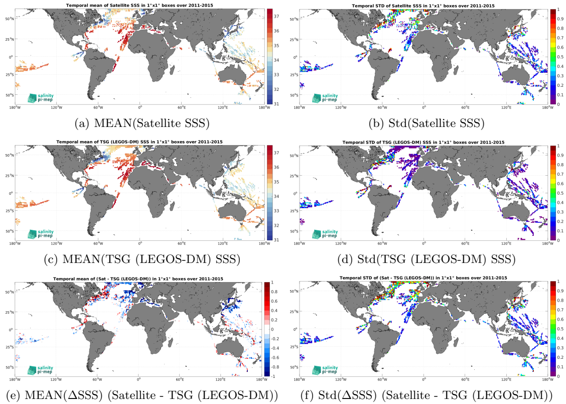
Figure 6: Temporal mean (left) and Std (right) of SSS from Aquarius SSS L2 OR v5 (NASA-GSFC) (top), TSG (LEGOS-DM) (middle), and of \Delta SSS (Satellite - TSG (LEGOS-DM)). Only match-up pairs are used to generate these maps.
