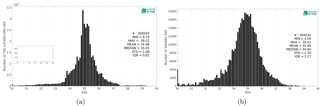
Figure 2: Histograms of SSS from TSG (LEGOS-DM) (a) and Aquarius SSS L2 OR v5 (NASA-GSFC) (b) considering all match-up pairs per bins of 0.1 over the SMOS coastal zone (<800km) 60N-60S Pi-MEP region and for the full satellite product period.
