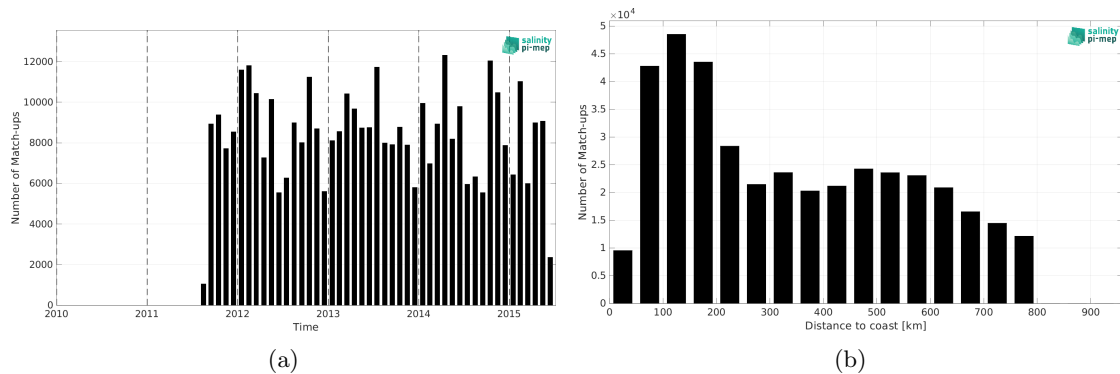
Figure 1: Number of match-ups between TSG (LEGOS-DM) and Aquarius SSS L2 OR v5 (NASA-GSFC) SSS as a function of time (a) and as function of the distance to coast (b) over the SMOS coastal zone (<800km) 60N-60S Pi-MEP region and for the full satellite product period.
