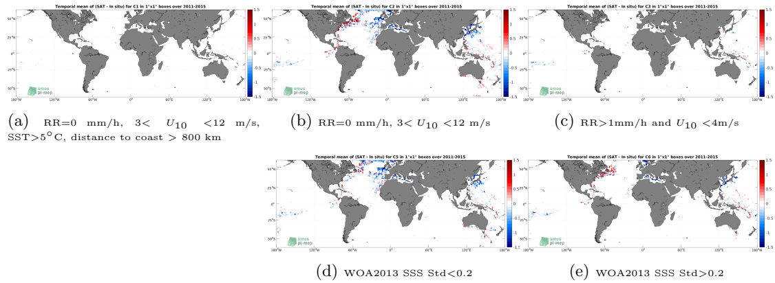
Figure 12: Temporal mean gridded over spatial boxes of size 1^\circ \times 1^\circ of \Delta\text{SSS} (Aquarius SSS L2 OR v5 (NASA-GSFC) - TSG (LEGOS-DM)) for 5 different subdatasets corresponding to:RR=0 mm/h, 3 < U_{10} < 12 m/s, SST >5^\circ\text{C} , distance to coast > 800 km (a), RR=0 mm/h, 3 < U_{10} < 12 m/s (b), RR >1 mm/h and U_{10} < 4 m/s (c), WOA2013 SSS Std <0.2 (d), WOA2013 SSS Std >0.2 (e).
