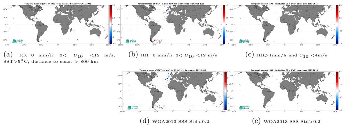
Figure 14: Temporal mean gridded over spatial boxes of size 1^\circ \times 1^\circ of \Delta SSS (Aquarius SSS L2 OR v5 (NASA-GSFC) - TSG (GOSUD-Sailing-ship)) for 5 different subdatasets corresponding to:RR=0 mm/h, 3 < U_{10} < 12 m/s, SST >5^\circ\text{C} , distance to coast > 800 km (a), RR=0 mm/h, 3 < U_{10} < 12 m/s (b), RR >1 mm/h and U_{10} < 4 m/s (c), WOA2013 SSS Std <0.2 (d), WOA2013 SSS Std >0.2 (e).
