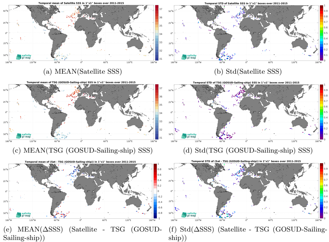
Figure 7: Temporal mean (left) and Std (right) of SSS from Aquarius SSS L2 OR v5 (NASA-GSFC) (top), TSG (GOSUD-Sailing-ship) (middle), and of \Delta SSS (Satellite - TSG (GOSUD-Sailing-ship)). Only match-up pairs are used to generate these maps.
