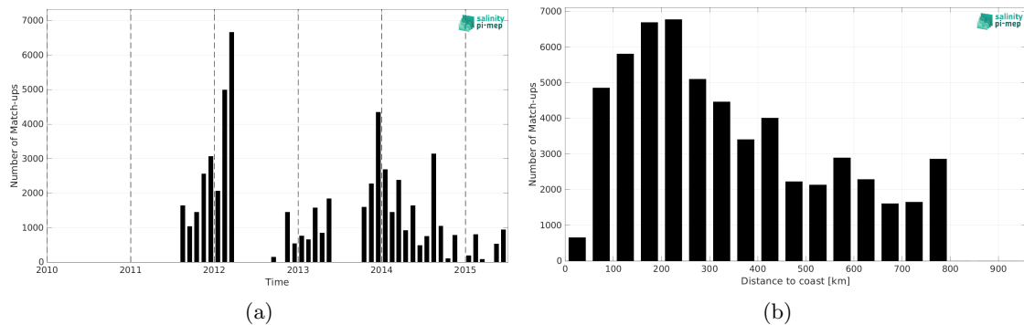
Figure 2: Number of match-ups between TSG (GOSUD-Sailing-ship) and Aquarius SSS L2 OR v5 (NASA-GSFC) SSS as a function of time (a) and as function of the distance to coast (b) over the SMOS coastal zone (<800km) 60N-60S Pi-MEP region and for the full satellite product period.
