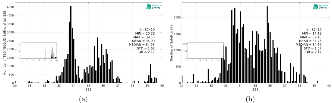
Figure 3: Histograms of SSS from TSG (GOSUD-Sailing-ship) (a) and Aquarius SSS L2 OR v5 (NASA-GSFC) (b) considering all match-up pairs per bins of 0.1 over the SMOS coastal zone (<800km) 60N-60S Pi-MEP region and for the full satellite product period.
