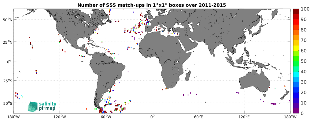
Figure 5: Number of SSS match-ups between TSG (GOSUD-Sailing-ship) SSS and the Aquarius SSS L2 OR v5 (NASA-GSFC) SSS product for the SMOS coastal zone (<800km) 60N-60S Pi-MEP region over 1^\circ \times 1^\circ boxes and for the full satellite product period.
