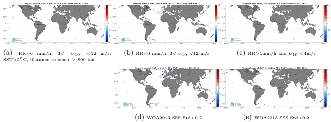
Figure 12: Temporal mean gridded over spatial boxes of size 1^\circ \times 1^\circ of \Delta SSS (Aquarius SSS L2 OR v5 (NASA-GSFC) - TSG (GOSUD-Sailing-ship)) for 5 different subdatasets corresponding to:RR=0 mm/h, 3 < U_{10} < 12 m/s, SST > 5^\circ\text{C} , distance to coast > 800 km (a), RR=0 mm/h, 3 < U_{10} < 12 m/s (b), RR > 1 mm/h and U_{10} < 4 m/s (c), WOA2013 SSS Std < 0.2 (d), WOA2013 SSS Std > 0.2 (e).
