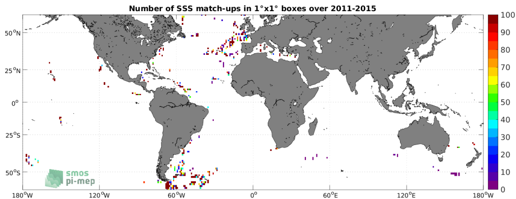
Figure 4: Number of SSS match-ups between TSG (GOSUD-Sailing-ship) SSS and the Aquarius SSS L2 OR v5 (NASA-GSFC) SSS product for the SMOS coastal zone (<800km) 60N-60S Pi-MEP region over 1^\circ \times 1^\circ boxes and for the full satellite product period.
