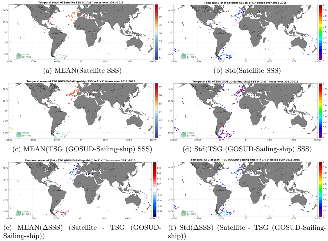
Figure 6: Temporal mean (left) and Std (right) of SSS from Aquarius SSS L2 OR v5 (NASA-GSFC) (top), TSG (GOSUD-Sailing-ship) (middle), and of \Delta SSS (Satellite - TSG (GOSUD-Sailing-ship)). Only match-up pairs are used to generate these maps.
