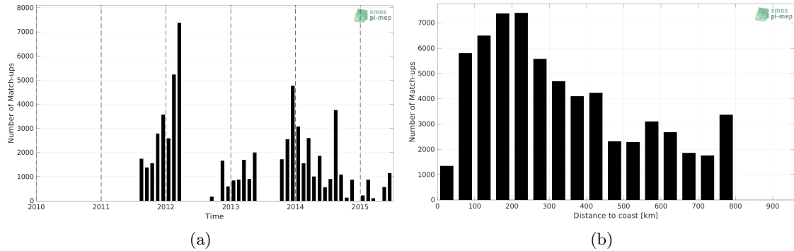
Figure 1: Number of match-ups between TSG (GOSUD-Sailing-ship) and Aquarius SSS L2 OR v5 (NASA-GSFC) SSS as a function of time (a) and as function of the distance to coast (b) over the SMOS coastal zone (<800km) 60N-60S Pi-MEP region and for the full satellite product period.
