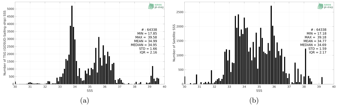
Figure 2: Histograms of SSS from TSG (GOSUD-Sailing-ship) (a) and Aquarius SSS L2 OR v5 (NASA-GSFC) (b) considering all match-up pairs per bins of 0.1 over the SMOS coastal zone (<800km) 60N-60S Pi-MEP region and for the full satellite product period.
