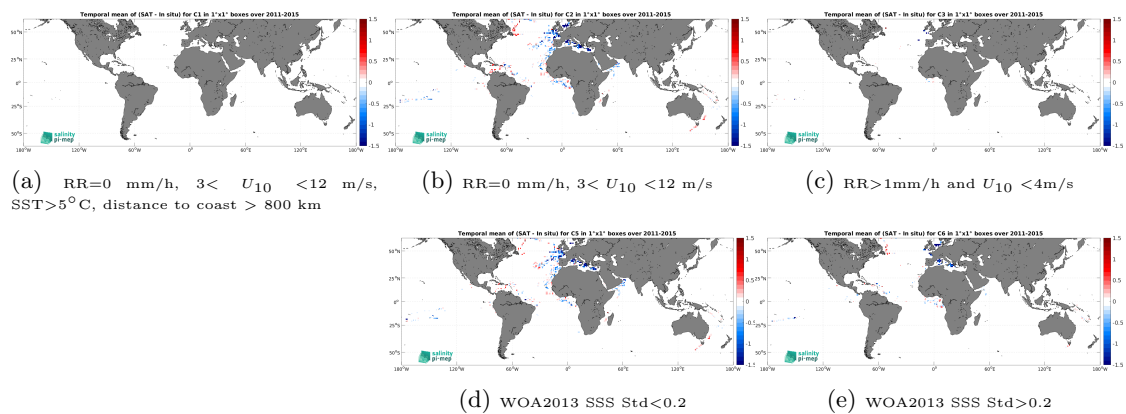
Figure 14: Temporal mean gridded over spatial boxes of size 1^\circ \times 1^\circ of \Delta\text{SSS} (Aquarius SSS L2 OR v5 (NASA-GSFC) - TSG (GOSUD-Research-vessel)) for 5 different subdatasets corresponding to: RR=0 mm/h, 3 < U_{10} < 12 m/s, SST > 5°C, distance to coast > 800 km (a), RR=0 mm/h, 3 < U_{10} < 12 m/s (b), RR > 1mm/h and U_{10} < 4 m/s (c), WOA2013 SSS Std < 0.2 (d), WOA2013 SSS Std > 0.2 (e).
