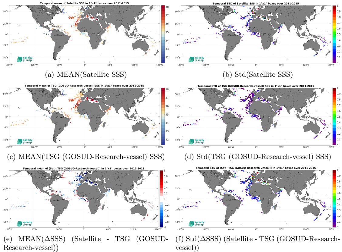
Figure 7: Temporal mean (left) and Std (right) of SSS from Aquarius SSS L2 OR v5 (NASA-GSFC) (top), TSG (GOSUD-Research-vessel) (middle), and of \Delta SSS (Satellite - TSG (GOSUD-Research-vessel)). Only match-up pairs are used to generate these maps.
