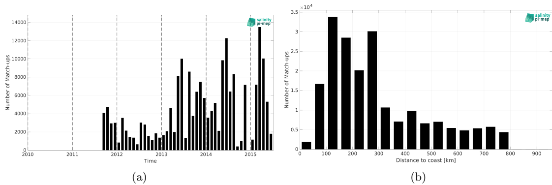
Figure 2: Number of match-ups between TSG (GOSUD-Research-vessel) and Aquarius SSS L2 OR v5 (NASA-GSFC) SSS as a function of time (a) and as function of the distance to coast (b) over the SMOS coastal zone (<800km) 60N-60S Pi-MEP region and for the full satellite product period.
