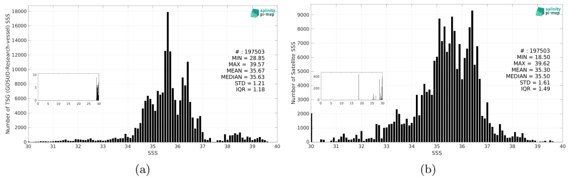
Figure 3: Histograms of SSS from TSG (GOSUD-Research-vessel) (a) and Aquarius SSS L2 OR v5 (NASA-GSFC) (b) considering all match-up pairs per bins of 0.1 over the SMOS coastal zone (<800km) 60N-60S Pi-MEP region and for the full satellite product period.
