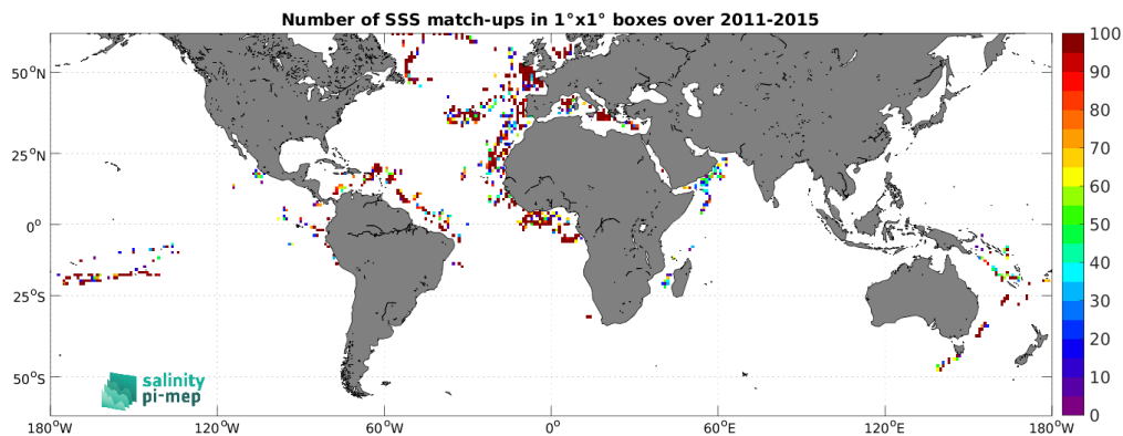
Figure 5: Number of SSS match-ups between TSG (GOSUD-Research-vessel) SSS and the Aquarius SSS L2 OR v5 (NASA-GSFC) SSS product for the SMOS coastal zone (<800km) 60N-60S Pi-MEP region over 1^\circ \times 1^\circ boxes and for the full satellite product period.
