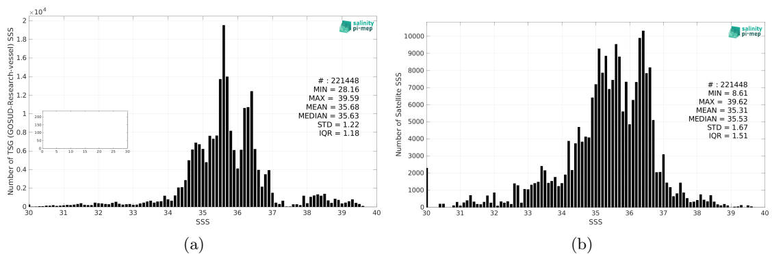
Figure 2: Histograms of SSS from TSG (GOSUD-Research-vessel) (a) and Aquarius SSS L2 OR v5 (NASA-GSFC) (b) considering all match-up pairs per bins of 0.1 over the SMOS coastal zone (<800km) 60N-60S Pi-MEP region and for the full satellite product period.
