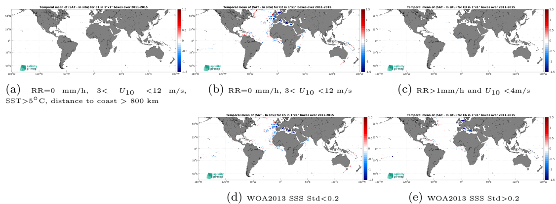
Figure 12: Temporal mean gridded over spatial boxes of size 1^\circ \times 1^\circ of \Delta\text{SSS} (Aquarius SSS L2 OR v5 (NASA-GSFC) - TSG (GOSUD-Research-vessel)) for 5 different subdatasets corresponding to:RR=0 mm/h, 3 < U_{10} < 12 m/s, SST >5^\circ\text{C} , distance to coast > 800 km (a), RR=0 mm/h, 3 < U_{10} < 12 m/s (b), RR >1 mm/h and U_{10} < 4 m/s (c), WOA2013 SSS Std <0.2 (d), WOA2013 SSS Std >0.2 (e).
