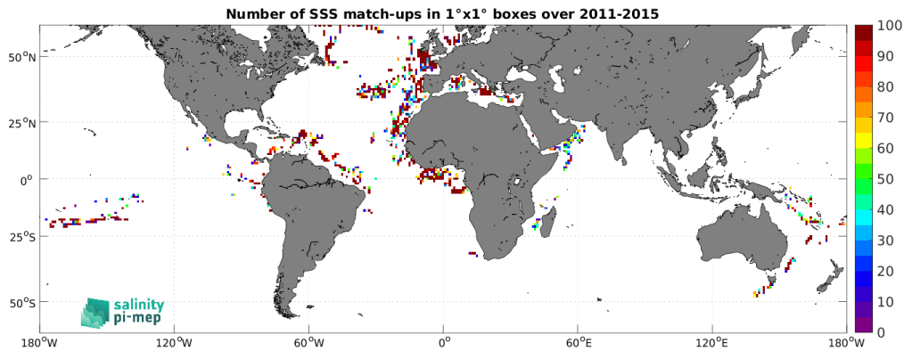
Figure 4: Number of SSS match-ups between TSG (GOSUD-Research-vessel) SSS and the Aquarius SSS L2 OR v5 (NASA-GSFC) SSS product for the SMOS coastal zone (<800km) 60N-60S Pi-MEP region over 1^\circ \times 1^\circ boxes and for the full satellite product period.
