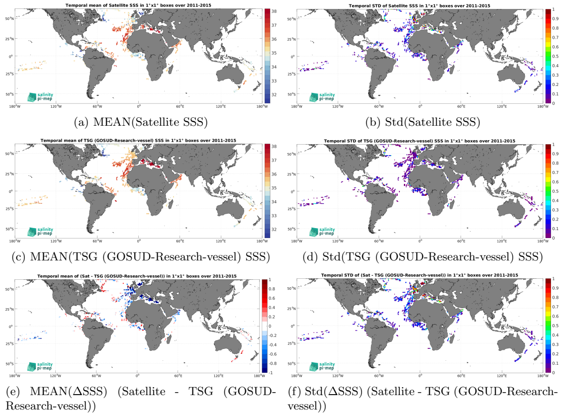
Figure 6: Temporal mean (left) and Std (right) of SSS from Aquarius SSS L2 OR v5 (NASA-GSFC) (top), TSG (GOSUD-Research-vessel) (middle), and of \Delta SSS (Satellite - TSG (GOSUD-Research-vessel)). Only match-up pairs are used to generate these maps.
