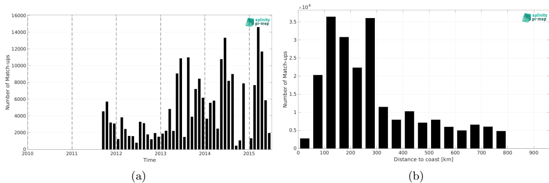
Figure 1: Number of match-ups between TSG (GOSUD-Research-vessel) and Aquarius SSS L2 OR v5 (NASA-GSFC) SSS as a function of time (a) and as function of the distance to coast (b) over the SMOS coastal zone (<800km) 60N-60S Pi-MEP region and for the full satellite product period.
