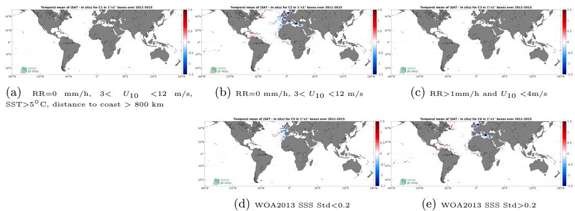
Figure 12: Temporal mean gridded over spatial boxes of size 1^\circ \times 1^\circ of \Delta SSS (Aquarius SSS L2 OR v5 (NASA-GSFC) - TSG (GOSUD-Research-vessel)) for 5 different subdatasets corresponding to:RR=0 mm/h, 3 < U_{10} < 12 m/s, SST >5^\circ\text{C} , distance to coast > 800 km (a), RR=0 mm/h, 3 < U_{10} < 12 m/s (b), RR >1 mm/h and U_{10} < 4 m/s (c), WOA2013 SSS Std <0.2 (d), WOA2013 SSS Std >0.2 (e).
