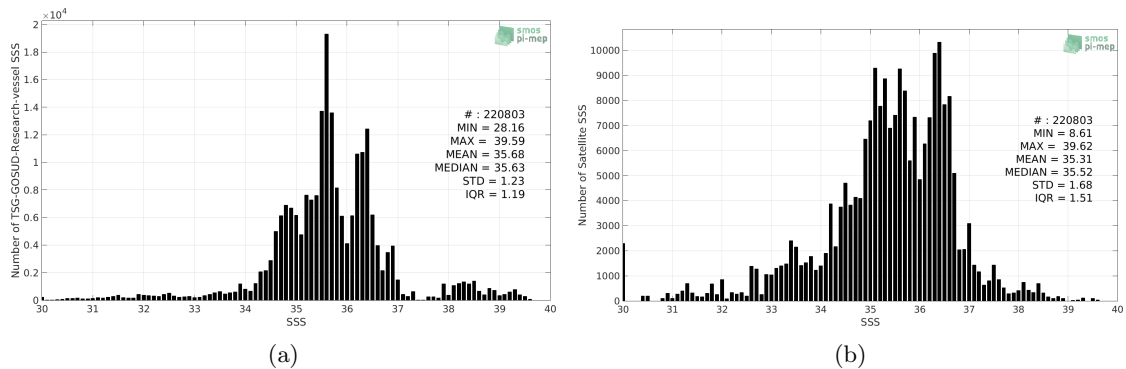
Figure 2: Histograms of SSS from TSG-GOSUD-Research-vessel (a) and Aquarius-L2-OR-V5 (b) considering all match-up pairs per bins of 0.1 over the SMOS coastal zone ( \approx 800 km) 60N-60S Pi-MEP region and for the full satellite product period.
