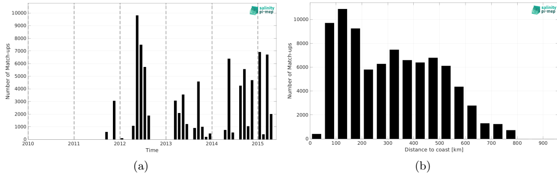
Figure 2: Number of match-ups between TSG (CSIC-UTM) and Aquarius SSS L2 OR v5 (NASA-GSFC) SSS as a function of time (a) and as function of the distance to coast (b) over the SMOS coastal zone (<800km) 60N-60S Pi-MEP region and for the full satellite product period.
