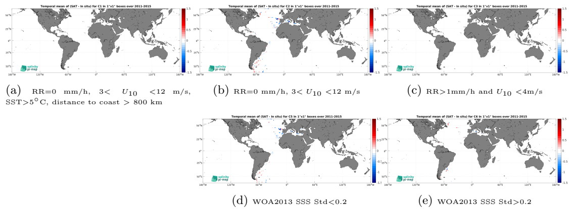
Figure 14: Temporal mean gridded over spatial boxes of size 1^\circ \times 1^\circ of \Delta SSS (Aquarius SSS L2 OR v5 (NASA-GSFC) - TSG (CSIC-UTM)) for 5 different subdatasets corresponding to: RR=0 mm/h, 3 < U_{10} < 12 m/s, SST > 5^\circ\text{C} , distance to coast > 800 km (a), RR=0 mm/h, 3 < U_{10} < 12 m/s (b), RR > 1 mm/h and U_{10} < 4 m/s (c), WOA2013 SSS Std < 0.2 (d), WOA2013 SSS Std > 0.2 (e).
