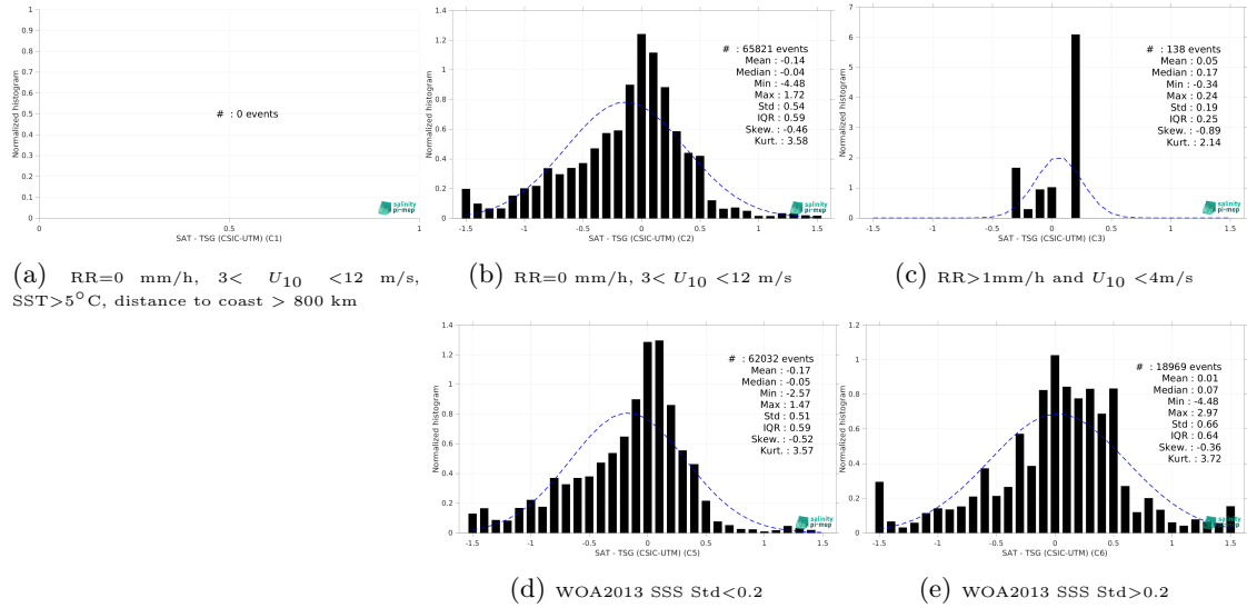
Figure 15: Normalized histogram of \Delta\text{SSS} (Aquarius SSS L2 OR v5 (NASA-GSFC) - TSG (CSIC-UTM)) for 5 different subdatasets corresponding to: RR=0 mm/h, 3 < U_{10} < 12 m/s, SST > 5^{\circ}\text{C} , distance to coast > 800 km (a), RR=0 mm/h, 3 < U_{10} < 12 m/s (b), RR > 1\text{mm/h} and U_{10} < 4\text{m/s} (c), WOA2013 SSS Std < 0.2 (d), WOA2013 SSS Std > 0.2 (e).
