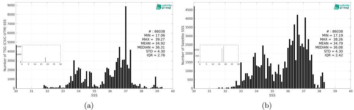
Figure 3: Histograms of SSS from TSG (CSIC-UTM) (a) and Aquarius SSS L2 OR v5 (NASA-GSFC) (b) considering all match-up pairs per bins of 0.1 over the SMOS coastal zone (<800km) 60N-60S Pi-MEP region and for the full satellite product period.
