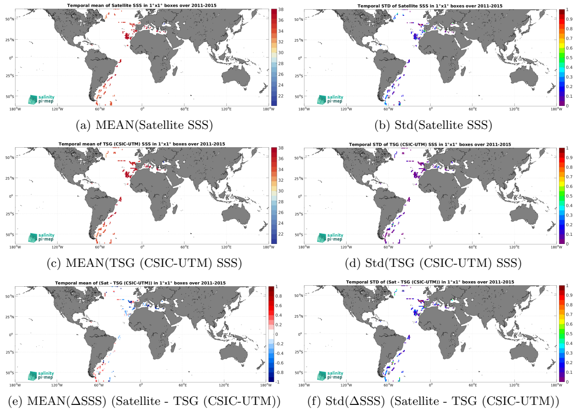
Figure 7: Temporal mean (left) and Std (right) of SSS from Aquarius SSS L2 OR v5 (NASA-GSFC) (top), TSG (CSIC-UTM) (middle), and of \Delta SSS (Satellite - TSG (CSIC-UTM)). Only match-up pairs are used to generate these maps.
