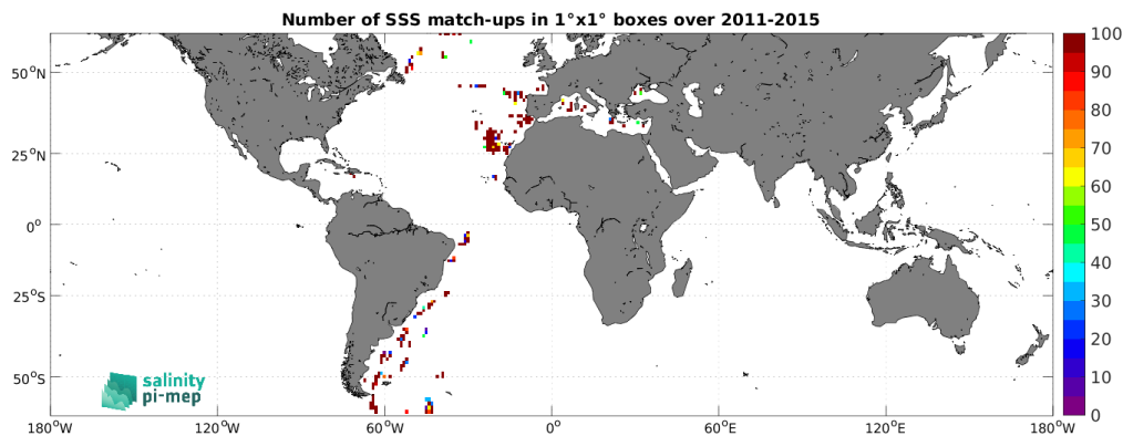
Figure 5: Number of SSS match-ups between TSG (CSIC-UTM) SSS and the Aquarius SSS L2 OR v5 (NASA-GSFC) SSS product for the SMOS coastal zone (<800km) 60N-60S Pi-MEP region over 1^\circ \times 1^\circ boxes and for the full satellite product period.
