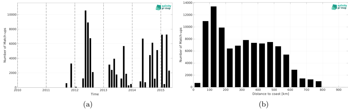
Figure 1: Number of match-ups between TSG (CSIC-UTM) and Aquarius SSS L2 OR v5 (NASA-GSFC) SSS as a function of time (a) and as function of the distance to coast (b) over the SMOS coastal zone (<800km) 60N-60S Pi-MEP region and for the full satellite product period.
