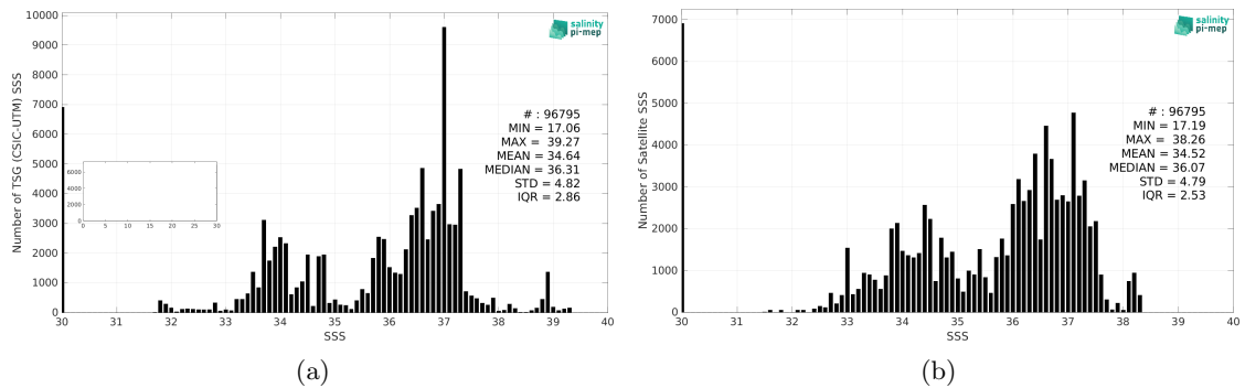
Figure 2: Histograms of SSS from TSG (CSIC-UTM) (a) and Aquarius SSS L2 OR v5 (NASA-GSFC) (b) considering all match-up pairs per bins of 0.1 over the SMOS coastal zone (<800km) 60N-60S Pi-MEP region and for the full satellite product period.
