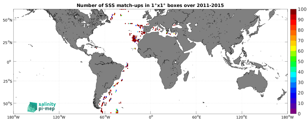
Figure 4: Number of SSS match-ups between TSG (CSIC-UTM) SSS and the Aquarius SSS L2 OR v5 (NASA-GSFC) SSS product for the SMOS coastal zone (<800km) 60N-60S Pi-MEP region over 1^\circ \times 1^\circ boxes and for the full satellite product period.
