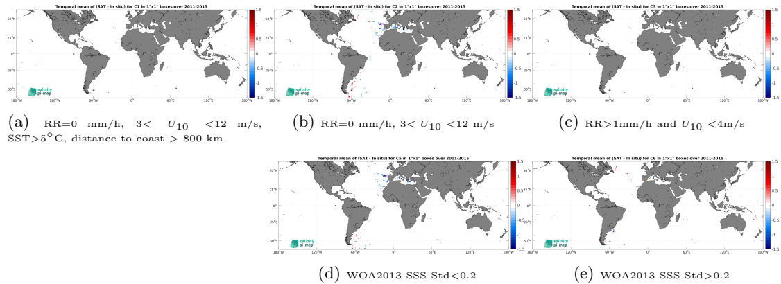
Figure 12: Temporal mean gridded over spatial boxes of size 1^\circ \times 1^\circ of \Delta SSS (Aquarius SSS L2 OR v5 (NASA-GSFC) - TSG (CSIC-UTM)) for 5 different subdatasets corresponding to:RR=0 mm/h, 3 < U_{10} < 12 m/s, SST >5^\circ\text{C} , distance to coast > 800 km (a), RR=0 mm/h, 3 < U_{10} < 12 m/s (b), RR >1 mm/h and U_{10} < 4 m/s (c), WOA2013 SSS Std <0.2 (d), WOA2013 SSS Std >0.2 (e).
