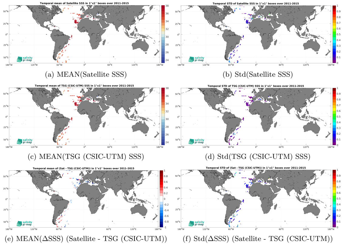
Figure 6: Temporal mean (left) and Std (right) of SSS from Aquarius SSS L2 OR v5 (NASA-GSFC) (top), TSG (CSIC-UTM) (middle), and of \Delta SSS (Satellite - TSG (CSIC-UTM)). Only match-up pairs are used to generate these maps.
