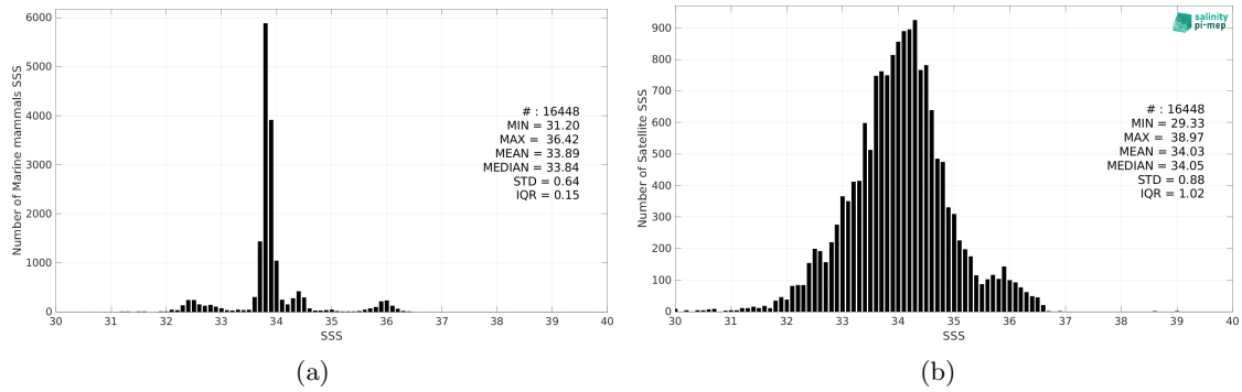
Figure 2: Histograms of SSS from Marine mammals (a) and Aquarius SSS L2 OR v5 (NASA-GSFC) (b) considering all match-up pairs per bins of 0.1 over the SMOS coastal zone (<800km) 60N-60S Pi-MEP region and for the full satellite product period.
