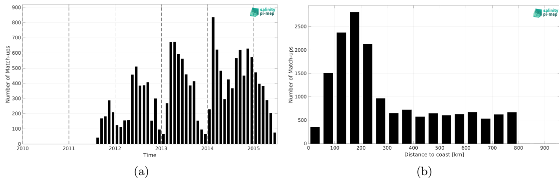
Figure 1: Number of match-ups between Marine mammals and Aquarius SSS L2 OR v5 (NASA-GSFC) SSS as a function of time (a) and as function of the distance to coast (b) over the SMOS coastal zone (<800km) 60N-60S Pi-MEP region and for the full satellite product period.
