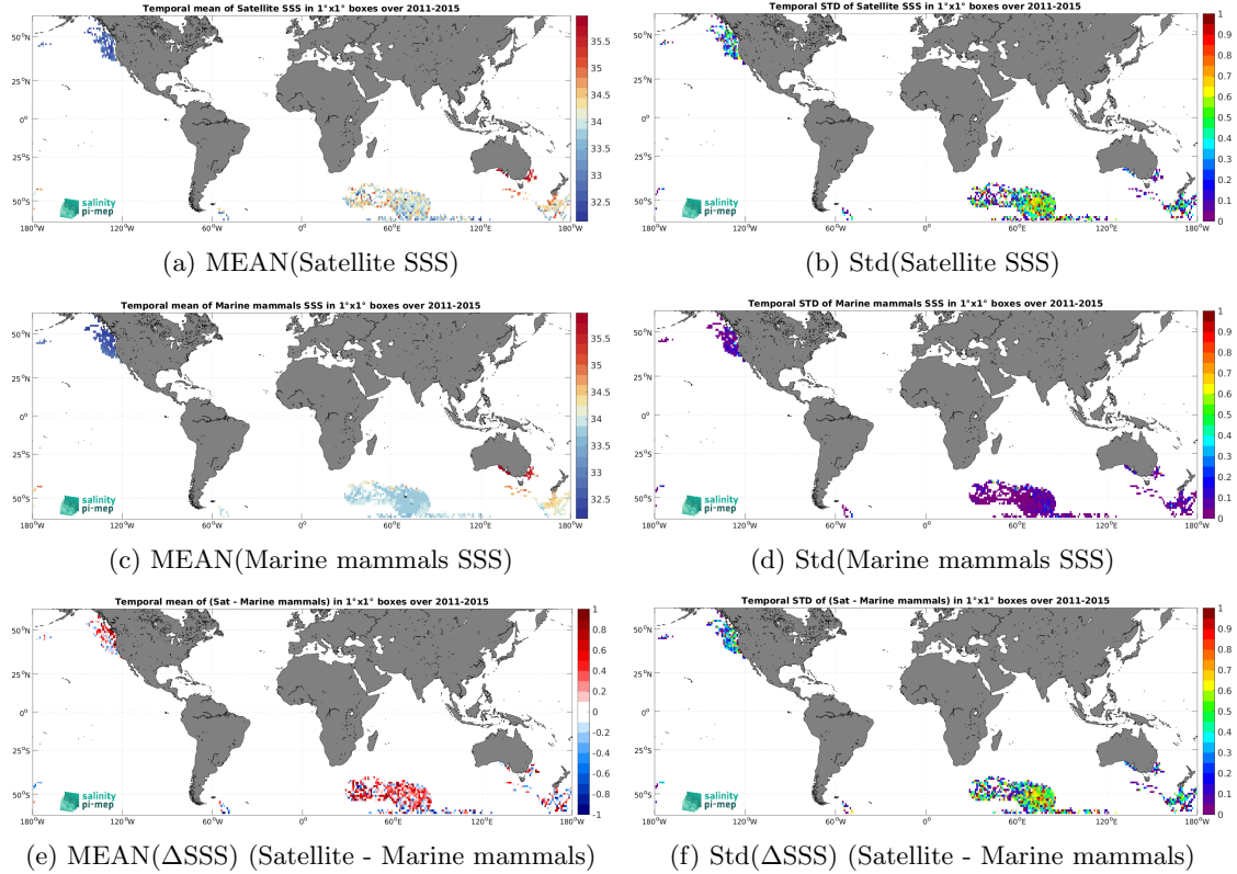
Figure 6: Temporal mean (left) and Std (right) of SSS from Aquarius SSS L2 OR v5 (NASA-GSFC) (top), Marine mammals (middle), and of \Delta SSS (Satellite - Marine mammals). Only match-up pairs are used to generate these maps.
