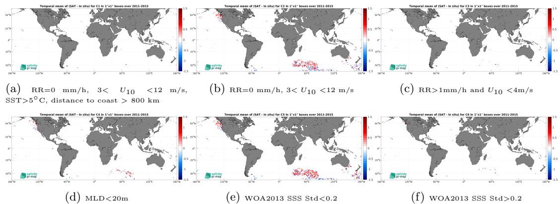
Figure 12: Temporal mean gridded over spatial boxes of size 1^\circ \times 1^\circ of \Delta SSS (Aquarius SSS L2 OR v5 (NASA-GSFC) - Marine mammals) for 6 different subdatasets corresponding to:RR=0 mm/h, 3 < U_{10} < 12 m/s, SST >5^\circ C, distance to coast > 800 km (a), RR=0 mm/h, 3 < U_{10} < 12 m/s (b), RR >1 mm/h and U_{10} < 4 m/s (c),MLD <20 m (d),WOA2013 SSS Std <0.2 (e),WOA2013 SSS Std >0.2 (f).
