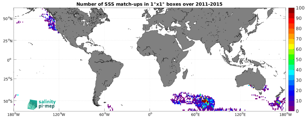
Figure 4: Number of SSS match-ups between Marine mammals SSS and the Aquarius SSS L2 OR v5 (NASA-GSFC) SSS product for the SMOS coastal zone (<800km) 60N-60S Pi-MEP region over 1^{\circ} \times 1^{\circ} boxes and for the full satellite product period.
