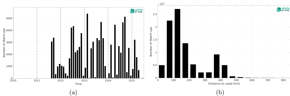
Figure 2: Number of match-ups between ICES and Aquarius SSS L2 OR v5 (NASA-GSFC) SSS as a function of time (a) and as function of the distance to coast (b) over the SMOS coastal zone (<800km) 60N-60S Pi-MEP region and for the full satellite product period.
