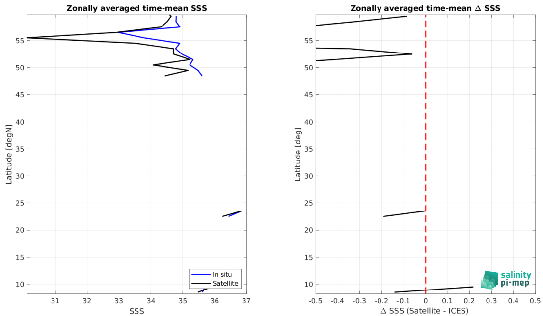
Figure 9: Left panel: Zonal mean SSS from Aquarius SSS L2 OR v5 (NASA-GSFC) satellite product (black) and from ICES (blue). Right panel: Zonal mean of \Delta SSS (Satellite - ICES) for all the collected Pi-MEP match-up pairs estimated over the full satellite product period.
