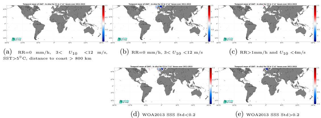
Figure 14: Temporal mean gridded over spatial boxes of size 1^\circ \times 1^\circ of \Delta\text{SSS} (Aquarius SSS L2 OR v5 (NASA-GSFC) - ICES) for 5 different subdatasets corresponding to:RR=0 mm/h, 3 < U_{10} < 12 m/s, SST >5^\circ\text{C} , distance to coast > 800 km (a), RR=0 mm/h, 3 < U_{10} < 12 m/s (b), RR >1 mm/h and U_{10} < 4 m/s (c), WOA2013 SSS Std <0.2 (d), WOA2013 SSS Std >0.2 (e).
