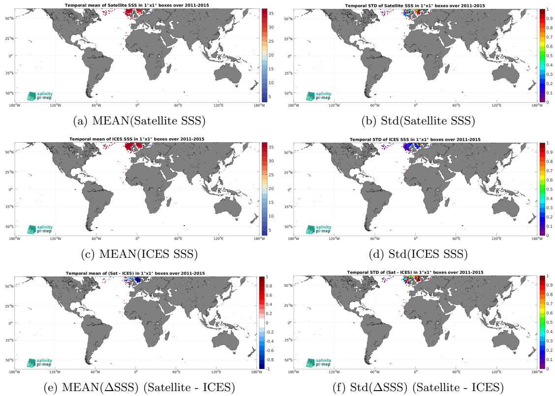
Figure 7: Temporal mean (left) and Std (right) of SSS from Aquarius SSS L2 OR v5 (NASA-GSFC) (top), ICES (middle), and of \Delta SSS (Satellite - ICES). Only match-up pairs are used to generate these maps.
