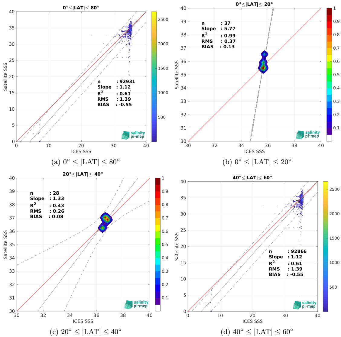
Figure 10: Contour maps of the concentration of Aquarius SSS L2 OR v5 (NASA-GSFC) SSS (y-axis) versus ICES SSS (x-axis) at match-up pairs for different latitude bands. For each plot, the red line shows x=y . The black thin and dashed lines indicate a linear fit through the data cloud and the \pm 95\% confidence levels, respectively. The number match-up pairs n , the slope and R^2 coefficient of the linear fit, the root mean square (RMS) and the mean bias between satellite and in situ data are indicated for each latitude band in each plots.
