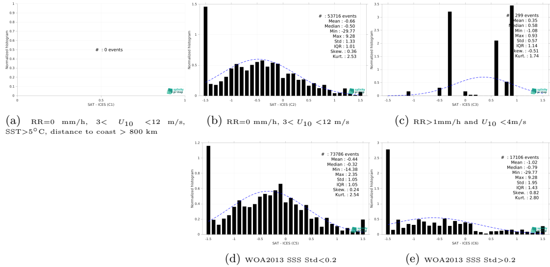
Figure 15: Normalized histogram of \Delta SSS (Aquarius SSS L2 OR v5 (NASA-GSFC) - ICES) for 5 different subdatasets corresponding to: RR=0 mm/h, 3 < U_{10} < 12 m/s, SST > 5°C, distance to coast > 800 km (a), RR=0 mm/h, 3 < U_{10} < 12 m/s (b), RR > 1mm/h and U_{10} < 4 m/s (c), WOA2013 SSS Std < 0.2 (d), WOA2013 SSS Std > 0.2 (e).
