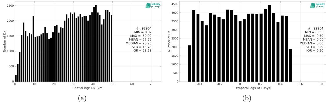
Figure 6: Histograms of the spatial (a) and temporal (b) lags between the location/time of the ICES measurement and the date of the corresponding Aquarius SSS L2 OR v5 (NASA-GSFC) SSS pixel.
