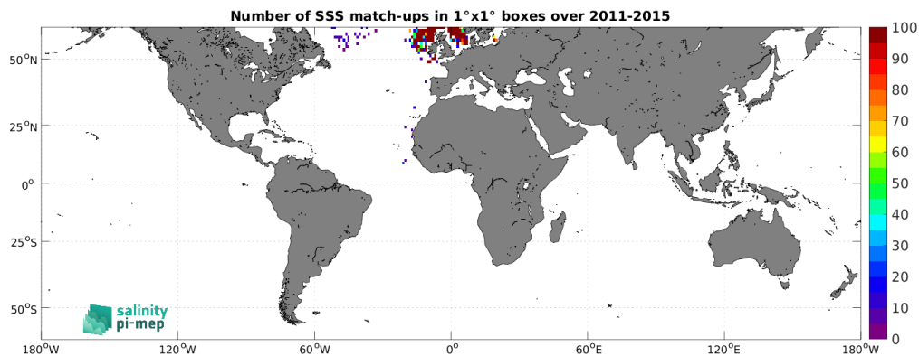
Figure 5: Number of SSS match-ups between ICES SSS and the Aquarius SSS L2 OR v5 (NASA-GSFC) SSS product for the SMOS coastal zone (<800km) 60N-60S Pi-MEP region over 1^\circ \times 1^\circ boxes and for the full satellite product period.
