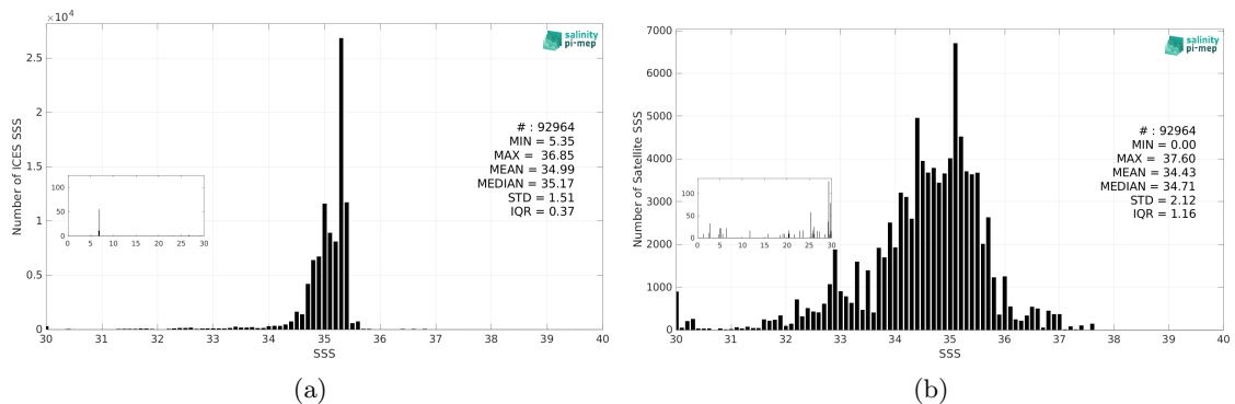
Figure 3: Histograms of SSS from ICES (a) and Aquarius SSS L2 OR v5 (NASA-GSFC) (b) considering all match-up pairs per bins of 0.1 over the SMOS coastal zone (<800km) 60N-60S Pi-MEP region and for the full satellite product period.
