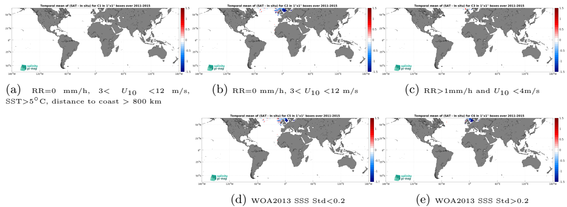
Figure 12: Temporal mean gridded over spatial boxes of size 1^\circ \times 1^\circ of \Delta\text{SSS} (Aquarius SSS L2 OR v5 (NASA-GSFC) - ICES) for 5 different subdatasets corresponding to:RR=0 mm/h, 3 < U_{10} < 12 m/s, SST >5^\circ\text{C} , distance to coast > 800 km (a), RR=0 mm/h, 3 < U_{10} < 12 m/s (b), RR >1 mm/h and U_{10} < 4 m/s (c), WOA2013 SSS Std <0.2 (d), WOA2013 SSS Std >0.2 (e).
