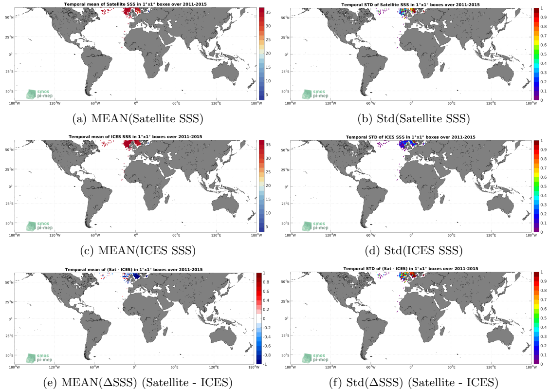
Figure 6: Temporal mean (left) and Std (right) of SSS from Aquarius SSS L2 OR v5 (NASA-GSFC) (top), ICES (middle), and of \Delta SSS (Satellite - ICES). Only match-up pairs are used to generate these maps.
