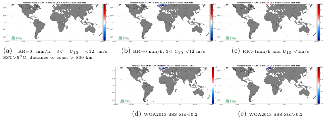
Figure 12: Temporal mean gridded over spatial boxes of size 1^\circ \times 1^\circ of \Delta SSS (Aquarius SSS L2 OR v5 (NASA-GSFC) - ICES) for 5 different subdatasets corresponding to:RR=0 mm/h, 3 < U_{10} < 12 m/s, SST >5^\circ\text{C} , distance to coast > 800 km (a), RR=0 mm/h, 3 < U_{10} < 12 m/s (b), RR >1 mm/h and U_{10} < 4 m/s (c), WOA2013 SSS Std <0.2 (d), WOA2013 SSS Std >0.2 (e).
