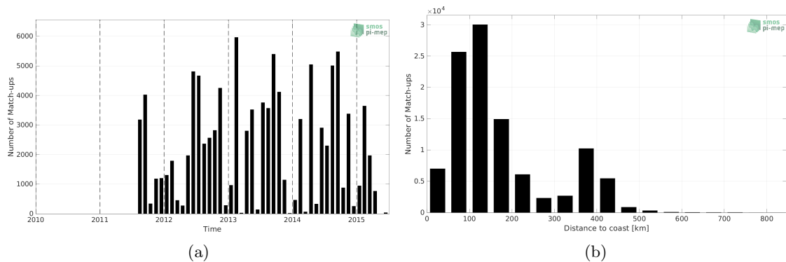
Figure 1: Number of match-ups between ICES and Aquarius SSS L2 OR v5 (NASA-GSFC) SSS as a function of time (a) and as function of the distance to coast (b) over the SMOS coastal zone (<800km) 60N-60S Pi-MEP region and for the full satellite product period.
