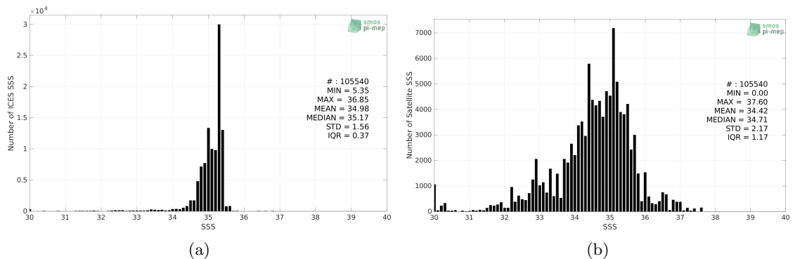
Figure 2: Histograms of SSS from ICES (a) and Aquarius SSS L2 OR v5 (NASA-GSFC) (b) considering all match-up pairs per bins of 0.1 over the SMOS coastal zone (<800km) 60N-60S Pi-MEP region and for the full satellite product period.
