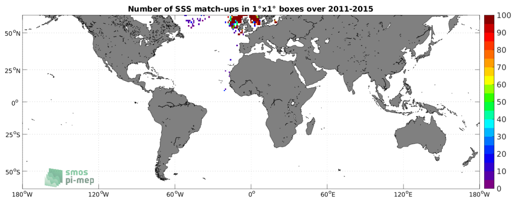
Figure 4: Number of SSS match-ups between ICES SSS and the Aquarius SSS L2 OR v5 (NASA-GSFC) SSS product for the SMOS coastal zone (<800km) 60N-60S Pi-MEP region over 1^\circ \times 1^\circ boxes and for the full satellite product period.
