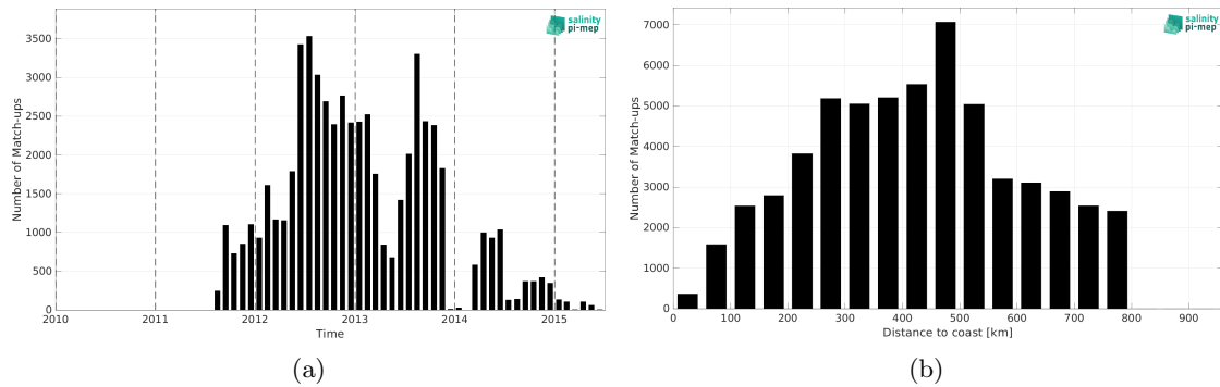
Figure 1: Number of match-ups between Surface drifters and Aquarius SSS L2 OR v5 (NASA-GSFC) SSS as a function of time (a) and as function of the distance to coast (b) over the SMOS coastal zone (<800km) 60N-60S Pi-MEP region and for the full satellite product period.
