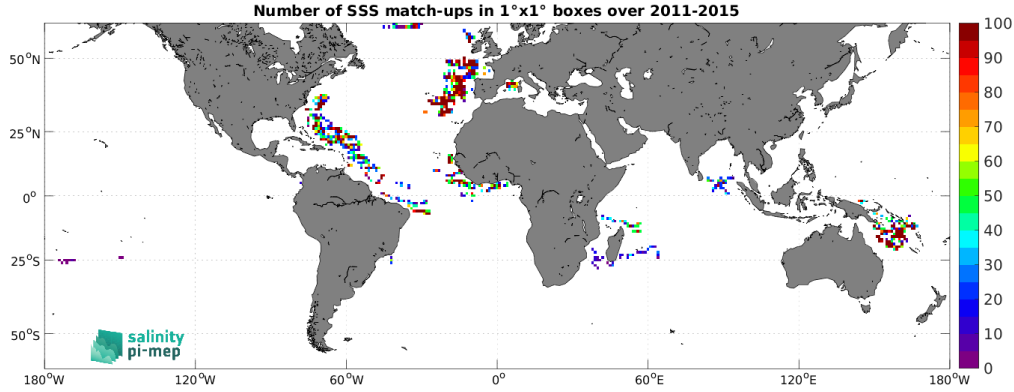
Figure 3: Number of SSS match-ups between Surface drifters SSS and the Aquarius SSS L2 OR v5 (NASA-GSFC) SSS product for the SMOS coastal zone (<800km) 60N-60S Pi-MEP region over 1^\circ \times 1^\circ boxes and for the full satellite product period.
