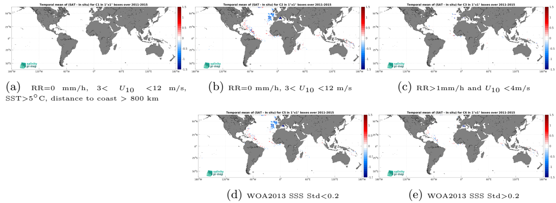
Figure 11: Temporal mean gridded over spatial boxes of size 1^\circ \times 1^\circ of \Delta\text{SSS} (Aquarius SSS L2 OR v5 (NASA-GSFC) - Surface drifters) for 5 different subdatasets corresponding to:RR=0 mm/h, 3 < U_{10} < 12 m/s, SST >5^\circ\text{C} , distance to coast > 800 km (a), RR=0 mm/h, 3 < U_{10} < 12 m/s (b), RR >1 mm/h and U_{10} < 4 m/s (c), WOA2013 SSS Std <0.2 (d), WOA2013 SSS Std >0.2 (e).
