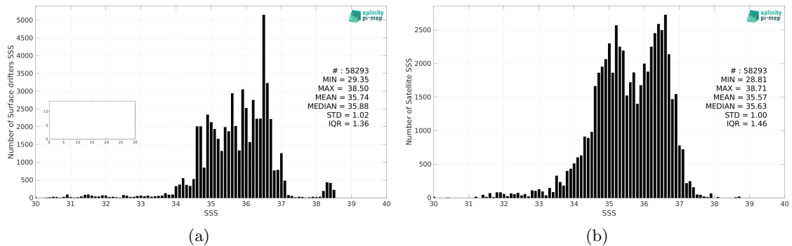
Figure 2: Histograms of SSS from Surface drifters (a) and Aquarius SSS L2 OR v5 (NASA-GSFC) (b) considering all match-up pairs per bins of 0.1 over the SMOS coastal zone (<800km) 60N-60S Pi-MEP region and for the full satellite product period.
