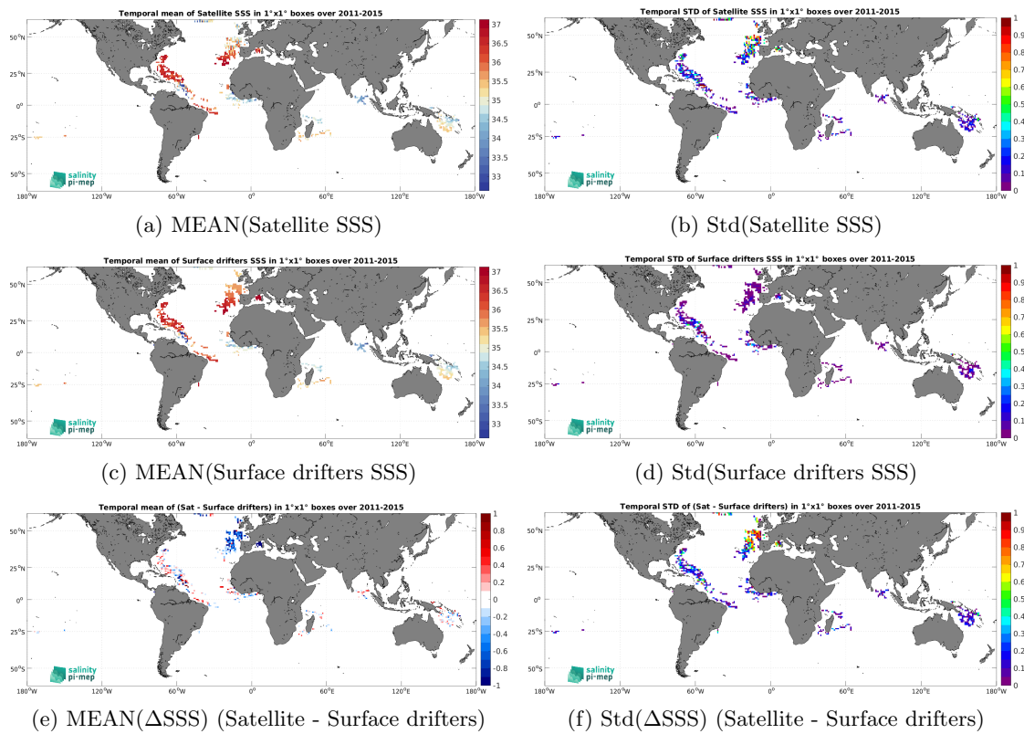
Figure 5: Temporal mean (left) and Std (right) of SSS from Aquarius SSS L2 OR v5 (NASA-GSFC) (top), Surface drifters (middle), and of \Delta SSS (Satellite - Surface drifters). Only match-up pairs are used to generate these maps.
