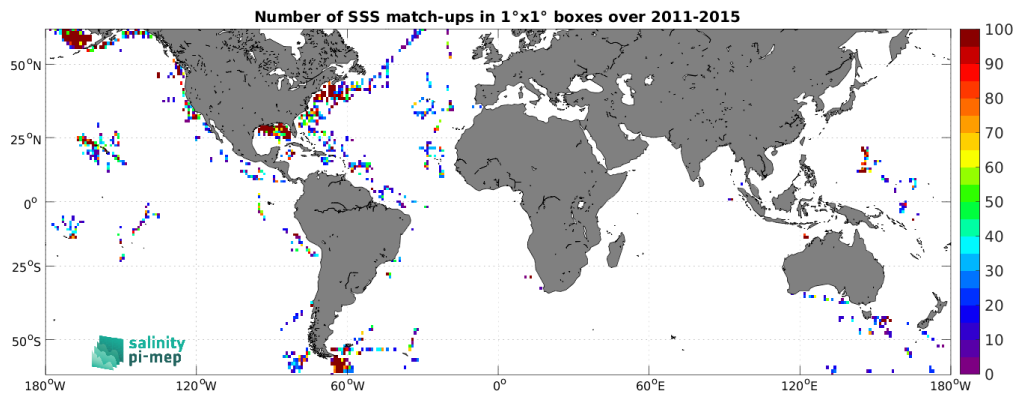
Figure 5: Number of SSS match-ups between TSG (SAMOS) SSS and the Aquarius SSS L2 CAP v5 (JPL) SSS product for the SMOS coastal zone (<800km) 60N-60S Pi-MEP region over 1^\circ \times 1^\circ boxes and for the full satellite product period.
