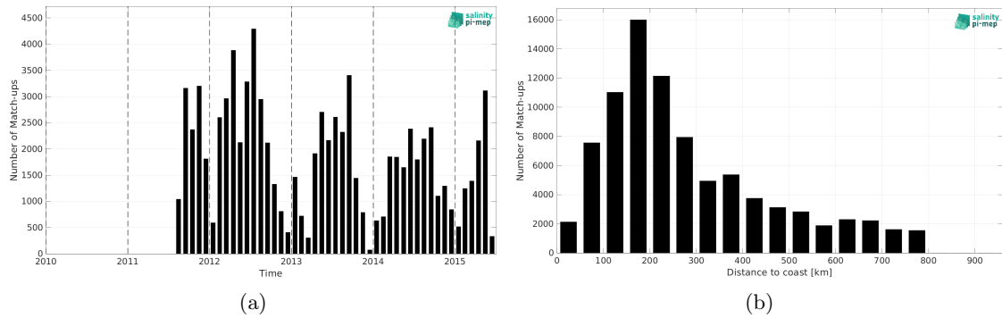
Figure 2: Number of match-ups between TSG (SAMOS) and Aquarius SSS L2 CAP v5 (JPL) SSS as a function of time (a) and as function of the distance to coast (b) over the SMOS coastal zone (<800km) 60N-60S Pi-MEP region and for the full satellite product period.
