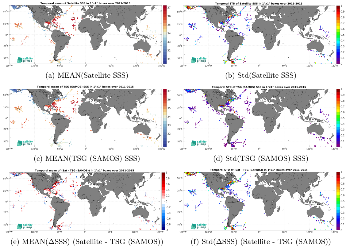
Figure 7: Temporal mean (left) and Std (right) of SSS from Aquarius SSS L2 CAP v5 (JPL) (top), TSG (SAMOS) (middle), and of \Delta SSS (Satellite - TSG (SAMOS)). Only match-up pairs are used to generate these maps.
