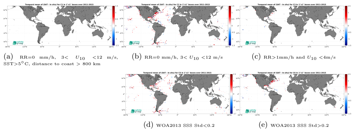
Figure 14: Temporal mean gridded over spatial boxes of size 1^\circ \times 1^\circ of \Delta\text{SSS} (Aquarius SSS L2 CAP v5 (JPL) - TSG (SAMOS)) for 5 different subdatasets corresponding to: RR=0 mm/h, 3 < U_{10} < 12 m/s, SST > 5°C, distance to coast > 800 km (a), RR=0 mm/h, 3 < U_{10} < 12 m/s (b), RR > 1mm/h and U_{10} < 4 m/s (c), WOA2013 SSS Std < 0.2 (d), WOA2013 SSS Std > 0.2 (e).
