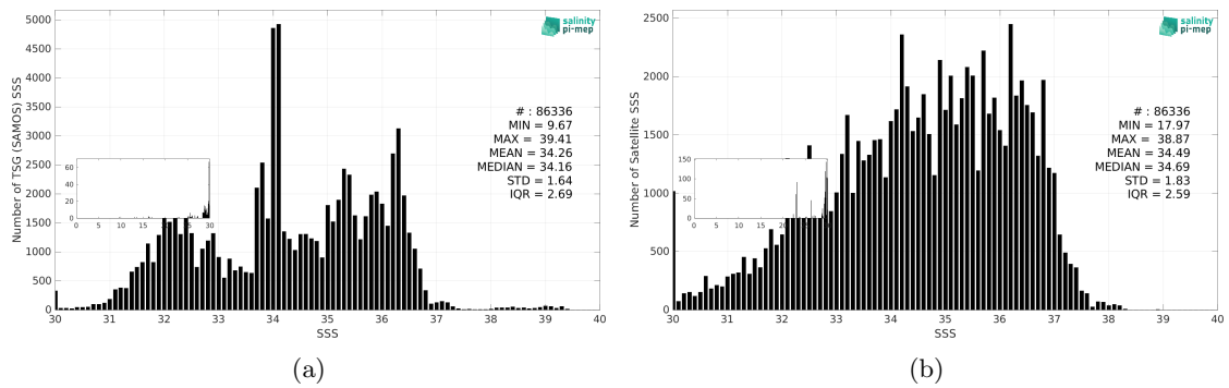
Figure 3: Histograms of SSS from TSG (SAMOS) (a) and Aquarius SSS L2 CAP v5 (JPL) (b) considering all match-up pairs per bins of 0.1 over the SMOS coastal zone (<800km) 60N-60S Pi-MEP region and for the full satellite product period.
