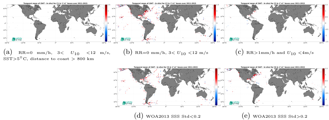
Figure 12: Temporal mean gridded over spatial boxes of size 1^\circ \times 1^\circ of \Delta\text{SSS} (Aquarius SSS L2 CAP v5 (JPL) - TSG (SAMOS)) for 5 different subdatasets corresponding to:RR=0 mm/h, 3 < U_{10} < 12 m/s, SST >5^\circ\text{C} , distance to coast > 800 km (a), RR=0 mm/h, 3 < U_{10} < 12 m/s (b), RR >1 mm/h and U_{10} < 4 m/s (c), WOA2013 SSS Std <0.2 (d), WOA2013 SSS Std >0.2 (e).
