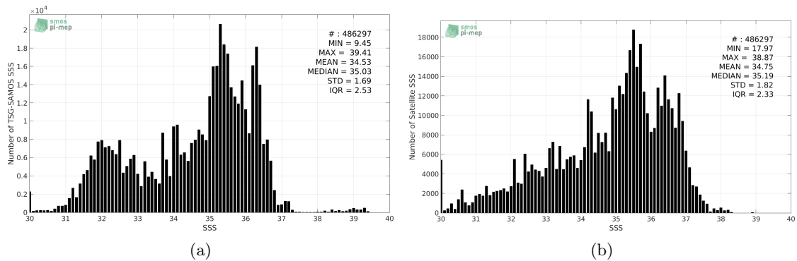
Figure 2: Histograms of SSS from TSG-SAMOS (a) and Aquarius-L2-JPL-V5 (b) considering all match-up pairs per bins of 0.1 over the SMOS coastal zone ( \approx 800\text{km} ) 60N-60S Pi-MEP region and for the full satellite product period.
