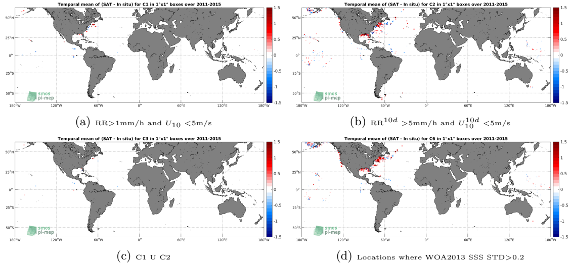
Figure 12: Temporal mean gridded over spatial boxes of size 1^\circ \times 1^\circ of \Delta SSS (Aquarius-L2-JPL-V5 - TSG-SAMOS) for 4 different subdatasets corresponding to: RR > 1\text{mm/h} and U_{10} < 5\text{m/s} (a), RR^{10d} > 5\text{mm/h} and U_{10}^{10d} < 5\text{m/s} (b), C1 U C2 (c), Locations where WOA2013 SSS STD > 0.2 (d).
