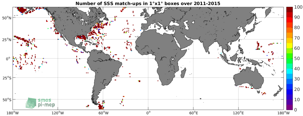
Figure 4: Number of SSS match-ups between TSG-SAMOS SSS and the Aquarius-L2-JPL-V5 SSS product for the SMOS coastal zone ( \geq 800\text{km} ) 60N-60S Pi-MEP region over 1^\circ \times 1^\circ boxes and for the full satellite product period.
