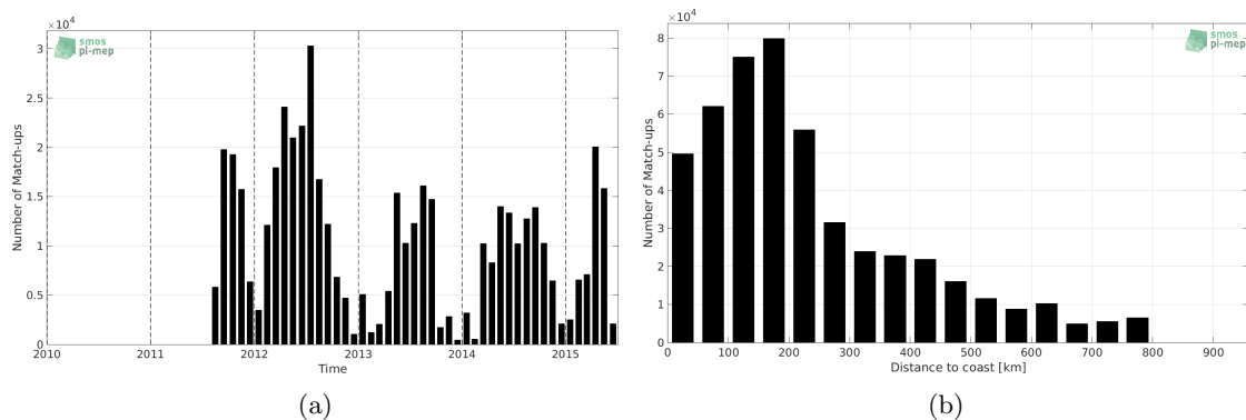
Figure 1: Number of match-ups between TSG-SAMOS and Aquarius-L2-JPL-V5 SSS as a function of time (a) and as function of the distance to coast (b) over the SMOS coastal zone ( \approx 800 km) 60N-60S Pi-MEP region and for the full satellite product period.
