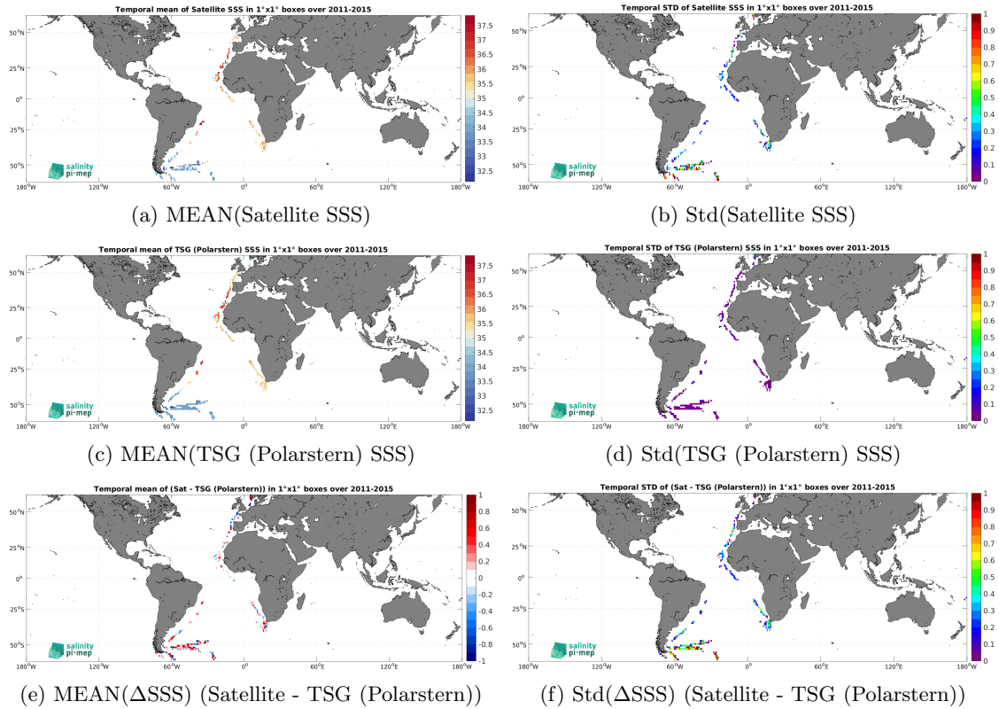
Figure 7: Temporal mean (left) and Std (right) of SSS from Aquarius SSS L2 CAP v5 (JPL) (top), TSG (Polarstern) (middle), and of \Delta SSS (Satellite - TSG (Polarstern)). Only match-up pairs are used to generate these maps.
