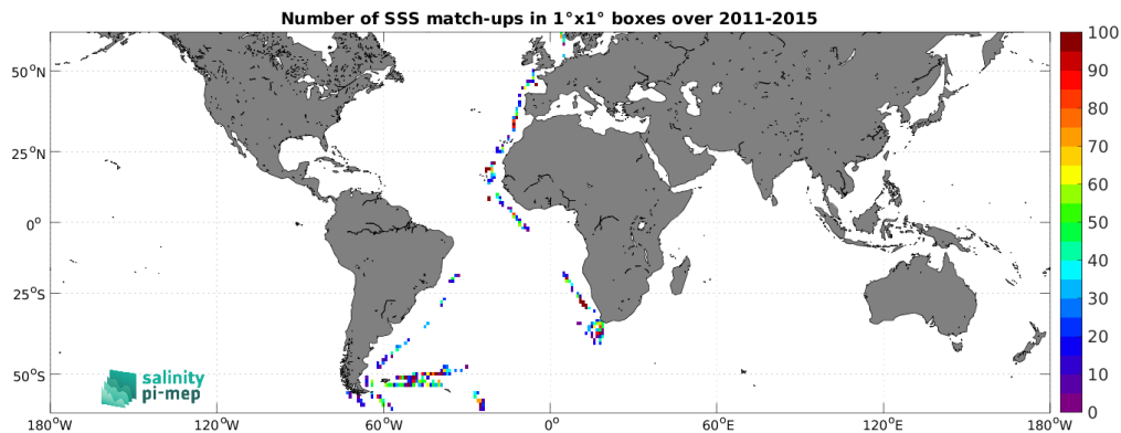
Figure 5: Number of SSS match-ups between TSG (Polarstern) SSS and the Aquarius SSS L2 CAP v5 (JPL) SSS product for the SMOS coastal zone (<800km) 60N-60S Pi-MEP region over 1^\circ \times 1^\circ boxes and for the full satellite product period.
