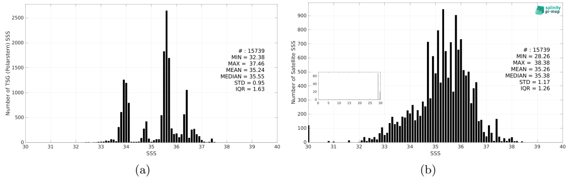
Figure 3: Histograms of SSS from TSG (Polarstern) (a) and Aquarius SSS L2 CAP v5 (JPL) (b) considering all match-up pairs per bins of 0.1 over the SMOS coastal zone (<800km) 60N-60S Pi-MEP region and for the full satellite product period.
