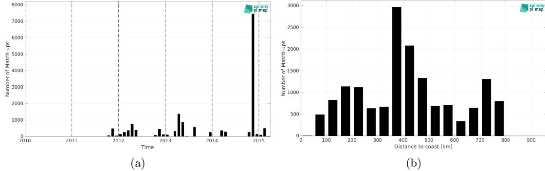
Figure 2: Number of match-ups between TSG (Polarstern) and Aquarius SSS L2 CAP v5 (JPL) SSS as a function of time (a) and as function of the distance to coast (b) over the SMOS coastal zone (<800km) 60N-60S Pi-MEP region and for the full satellite product period.
