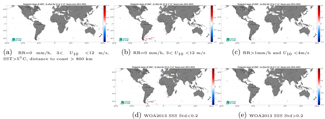
Figure 14: Temporal mean gridded over spatial boxes of size 1^\circ \times 1^\circ of \Delta SSS (Aquarius SSS L2 CAP v5 (JPL) - TSG (Polarstern)) for 5 different subdatasets corresponding to:RR=0 mm/h, 3 < U_{10} < 12 m/s, SST>5°C, distance to coast > 800 km (a), RR=0 mm/h, 3 < U_{10} < 12 m/s (b), RR>1mm/h and U_{10} < 4 m/s (c), WOA2013 SSS Std<0.2 (d), WOA2013 SSS Std>0.2 (e).
