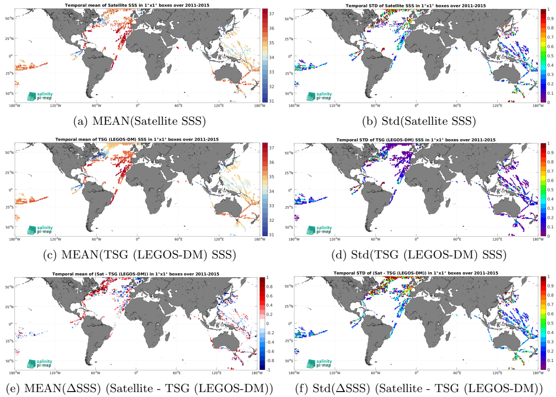
Figure 7: Temporal mean (left) and Std (right) of SSS from Aquarius SSS L2 CAP v5 (JPL) (top), TSG (LEGOS-DM) (middle), and of \Delta SSS (Satellite - TSG (LEGOS-DM)). Only match-up pairs are used to generate these maps.
