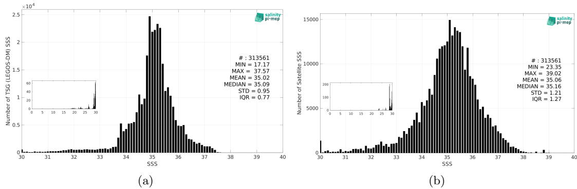
Figure 3: Histograms of SSS from TSG (LEGOS-DM) (a) and Aquarius SSS L2 CAP v5 (JPL) (b) considering all match-up pairs per bins of 0.1 over the SMOS coastal zone (<800km) 60N-60S Pi-MEP region and for the full satellite product period.
