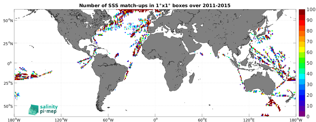
Figure 5: Number of SSS match-ups between TSG (LEGOS-DM) SSS and the Aquarius SSS L2 CAP v5 (JPL) SSS product for the SMOS coastal zone (<800km) 60N-60S Pi-MEP region over 1^\circ \times 1^\circ boxes and for the full satellite product period.
