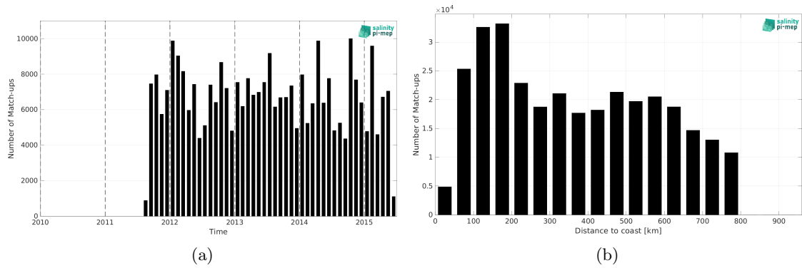
Figure 2: Number of match-ups between TSG (LEGOS-DM) and Aquarius SSS L2 CAP v5 (JPL) SSS as a function of time (a) and as function of the distance to coast (b) over the SMOS coastal zone (<800km) 60N-60S Pi-MEP region and for the full satellite product period.
