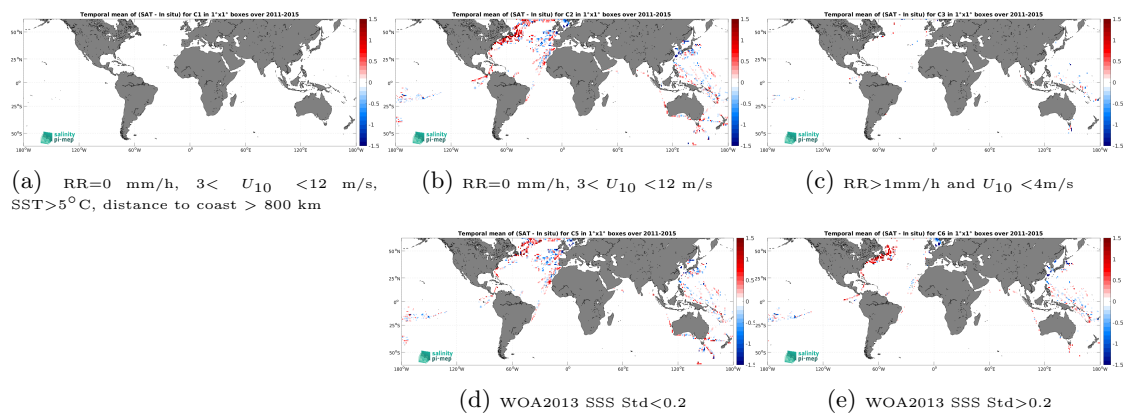
Figure 14: Temporal mean gridded over spatial boxes of size 1^\circ \times 1^\circ of \Delta SSS (Aquarius SSS L2 CAP v5 (JPL) - TSG (LEGOS-DM)) for 5 different subdatasets corresponding to: RR=0 mm/h, 3 < U_{10} < 12 m/s, SST > 5^\circ\text{C} , distance to coast > 800 km (a), RR=0 mm/h, 3 < U_{10} < 12 m/s (b), RR > 1 mm/h and U_{10} < 4 m/s (c), WOA2013 SSS Std < 0.2 (d), WOA2013 SSS Std > 0.2 (e).
