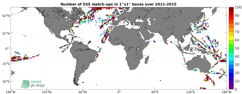
Figure 4: Number of SSS match-ups between TSG (LEGOS-DM) SSS and the Aquarius SSS L2 CAP v5 (JPL) SSS product for the SMOS coastal zone (<800km) 60N-60S Pi-MEP region over 1^\circ \times 1^\circ boxes and for the full satellite product period.
