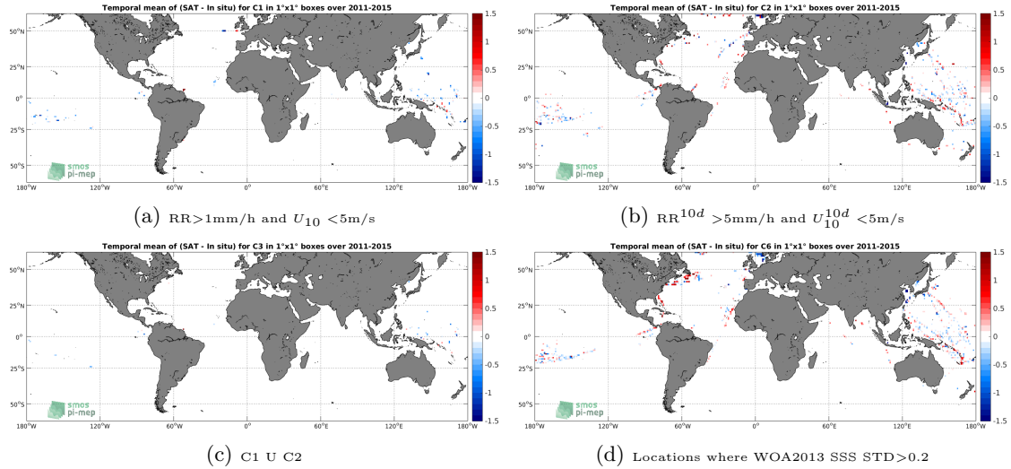
Figure 12: Temporal mean gridded over spatial boxes of size 1^\circ \times 1^\circ of \Delta SSS (Aquarius-L2-JPL-V5 - TSG-LEGOS-DM) for 4 different subdatasets corresponding to: RR > 1\text{mm/h} and U_{10} < 5\text{m/s} (a), RR^{10d} > 5\text{mm/h} and U_{10}^{10d} < 5\text{m/s} (b), C1 U C2 (c), Locations where WOA2013 SSS STD > 0.2 (d).
