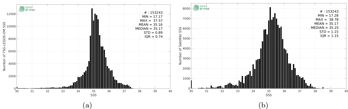
Figure 2: Histograms of SSS from TSG-LEGOS-DM (a) and Aquarius-L2-JPL-V5 (b) considering all match-up pairs per bins of 0.1 over the SMOS coastal zone ( \pm 800\text{km} ) 60N-60S Pi-MEP region and for the full satellite product period.
