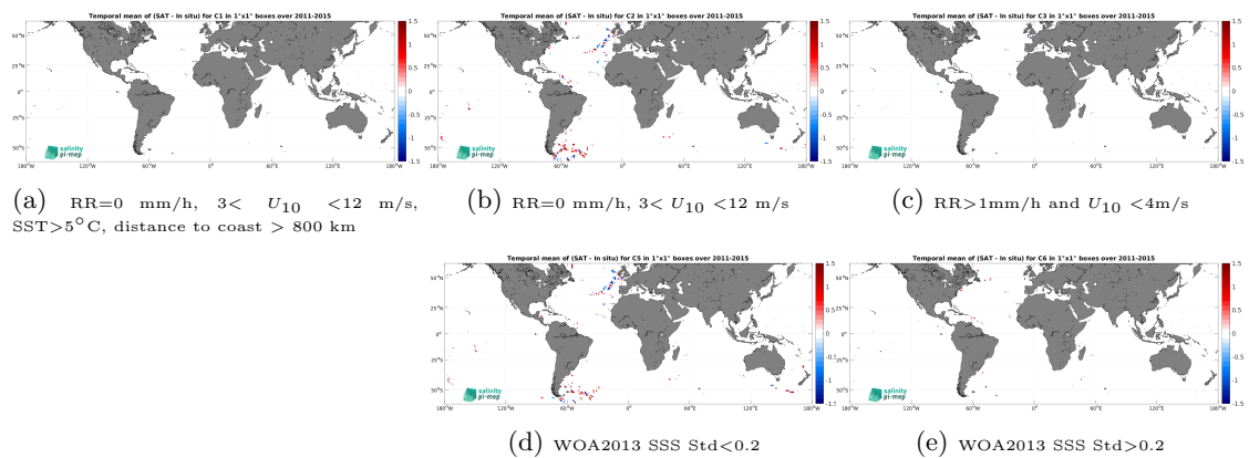
Figure 14: Temporal mean gridded over spatial boxes of size 1^\circ \times 1^\circ of \Delta SSS (Aquarius SSS L2 CAP v5 (JPL) - TSG (GOSUD-Sailing-ship)) for 5 different subdatasets corresponding to:RR=0 mm/h, 3 < U_{10} < 12 m/s, SST >5^\circ\text{C} , distance to coast > 800 km (a), RR=0 mm/h, 3 < U_{10} < 12 m/s (b), RR >1 mm/h and U_{10} < 4 m/s (c), WOA2013 SSS Std <0.2 (d), WOA2013 SSS Std >0.2 (e).
