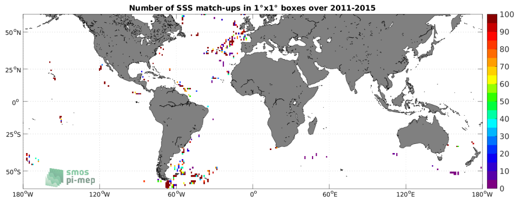
Figure 4: Number of SSS match-ups between TSG (GOSUD-Sailing-ship) SSS and the Aquarius SSS L2 CAP v5 (JPL) SSS product for the SMOS coastal zone (<800km) 60N-60S Pi-MEP region over 1^\circ \times 1^\circ boxes and for the full satellite product period.
