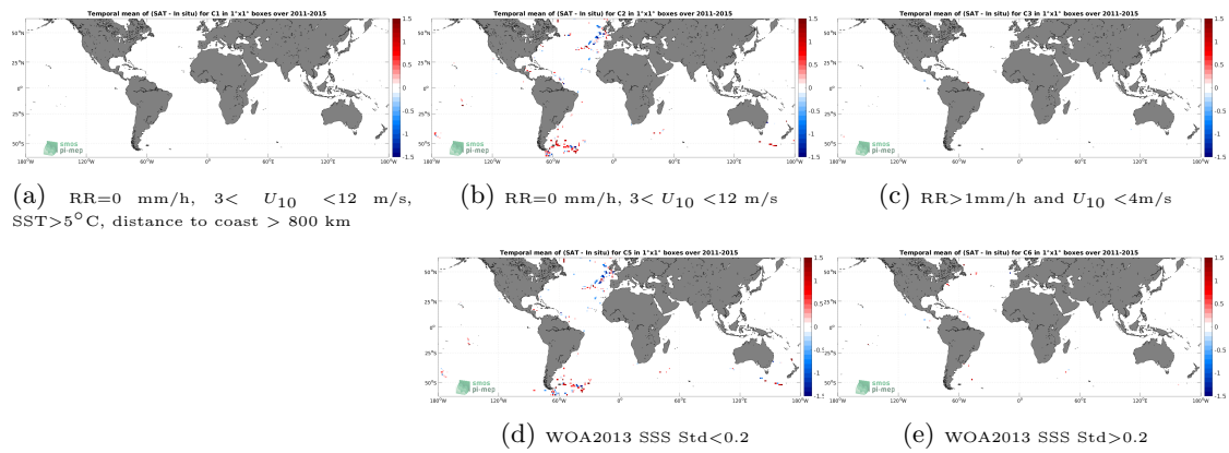
Figure 12: Temporal mean gridded over spatial boxes of size 1^\circ \times 1^\circ of \Delta\text{SSS} (Aquarius SSS L2 CAP v5 (JPL) - TSG (GOSUD-Sailing-ship)) for 5 different subdatasets corresponding to:RR=0 mm/h, 3 < U_{10} < 12 m/s, SST>5°C, distance to coast > 800 km (a), RR=0 mm/h, 3 < U_{10} < 12 m/s (b), RR>1mm/h and U_{10} < 4 m/s (c), WOA2013 SSS Std<0.2 (d), WOA2013 SSS Std>0.2 (e).
