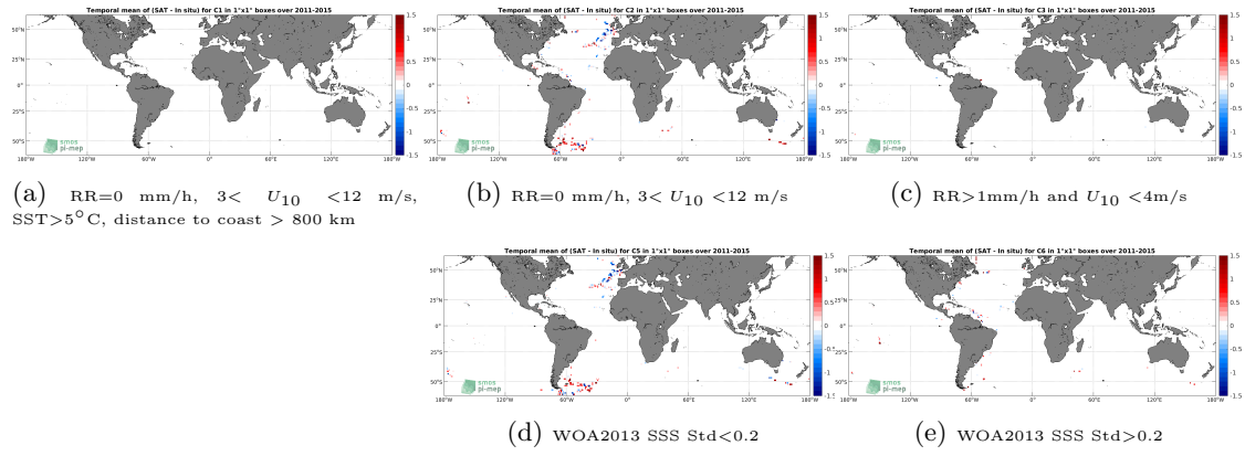
Figure 12: Temporal mean gridded over spatial boxes of size 1^\circ \times 1^\circ of \Delta SSS (Aquarius SSS L2 CAP v5 (JPL) - TSG (GOSUD-Sailing-ship)) for 5 different subdatasets corresponding to: RR=0 mm/h, 3 < U_{10} < 12 m/s, SST >5^\circ C, distance to coast > 800 km (a), RR=0 mm/h, 3 < U_{10} < 12 m/s (b), RR >1 mm/h and U_{10} < 4 m/s (c), WOA2013 SSS Std <0.2 (d), WOA2013 SSS Std >0.2 (e).
