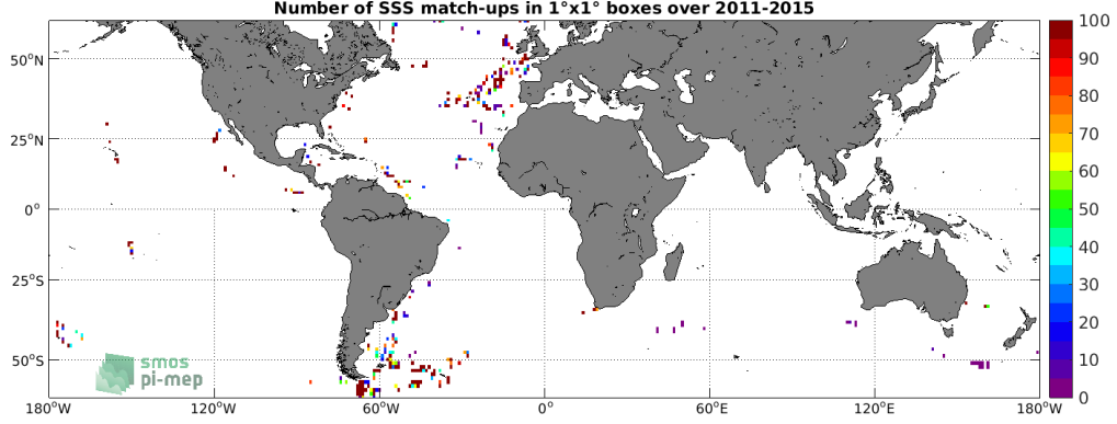
Figure 4: Number of SSS match-ups between TSG (GOSUD-Sailing-ship) SSS and the Aquarius SSS L2 CAP v5 (JPL) SSS product for the SMOS coastal zone (<800km) 60N-60S Pi-MEP region over 1°x1° boxes and for the full satellite product period.
