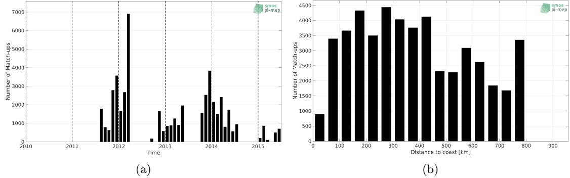
Figure 1: Number of match-ups between TSG (GOSUD-Sailing-ship) and Aquarius SSS L2 CAP v5 (JPL) SSS as a function of time (a) and as function of the distance to coast (b) over the SMOS coastal zone (<800km) 60N-60S Pi-MEP region and for the full satellite product period.
