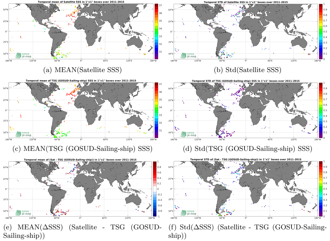
Figure 6: Temporal mean (left) and Std (right) of SSS from Aquarius SSS L2 CAP v5 (JPL) (top), TSG (GOSUD-Sailing-ship) (middle), and of \Delta SSS (Satellite - TSG (GOSUD-Sailing-ship)). Only match-up pairs are used to generate these maps.
