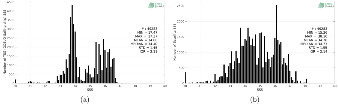
Figure 2: Histograms of SSS from TSG (GOSUD-Sailing-ship) (a) and Aquarius SSS L2 CAP v5 (JPL) (b) considering all match-up pairs per bins of 0.1 over the SMOS coastal zone (<800km) 60N-60S Pi-MEP region and for the full satellite product period.
