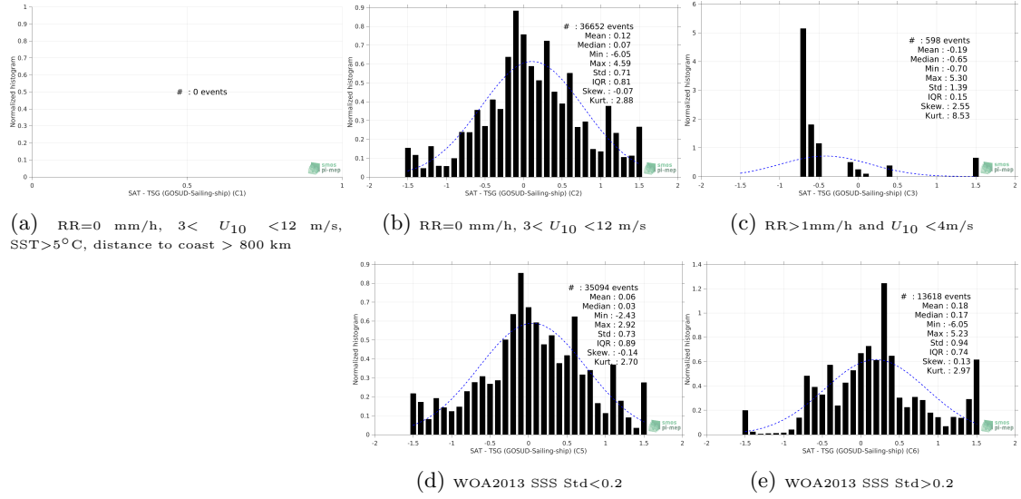
Figure 13: Normalized histogram of \Delta\text{SSS} (Aquarius SSS L2 CAP v5 (JPL) - TSG (GOSUD-Sailing-ship)) for 5 different subdatasets corresponding to: RR=0 mm/h, 3 < U_{10} < 12 m/s, SST > 5^\circ\text{C} , distance to coast > 800 km (a), RR=0 mm/h, 3 < U_{10} < 12 m/s (b), RR > 1 mm/h and U_{10} < 4 m/s (c), WOA2013 SSS Std < 0.2 (d), WOA2013 SSS Std > 0.2 (e).
