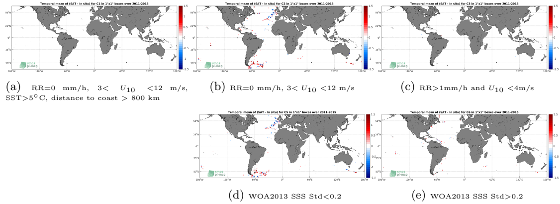
Figure 12: Temporal mean gridded over spatial boxes of size 1^\circ \times 1^\circ of \Delta SSS (Aquarius-L2-JPL-V5 - TSG-GOSUD-Sailing-ship) for 5 different subdatasets corresponding to: RR=0 mm/h, 3 < U_{10} < 12 m/s, SST > 5^\circ\text{C} , distance to coast > 800 km (a), RR=0 mm/h, 3 < U_{10} < 12 m/s (b), RR > 1 mm/h and U_{10} < 4 m/s (c), WOA2013 SSS Std < 0.2 (d), WOA2013 SSS Std > 0.2 (e).
