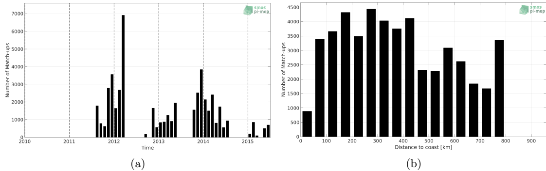
Figure 1: Number of match-ups between TSG-GOSUD-Sailing-ship and Aquarius-L2-JPL-V5 SSS as a function of time (a) and as function of the distance to coast (b) over the SMOS coastal zone (<800km) 60N-60S Pi-MEP region and for the full satellite product period.
