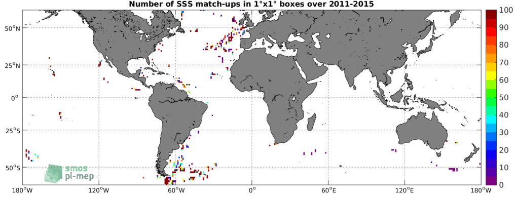
Figure 4: Number of SSS match-ups between TSG-GOSUD-Sailing-ship SSS and the Aquarius-L2-JPL-V5 SSS product for the SMOS coastal zone (<800km) 60N-60S Pi-MEP region over 1°x1° boxes and for the full satellite product period.
