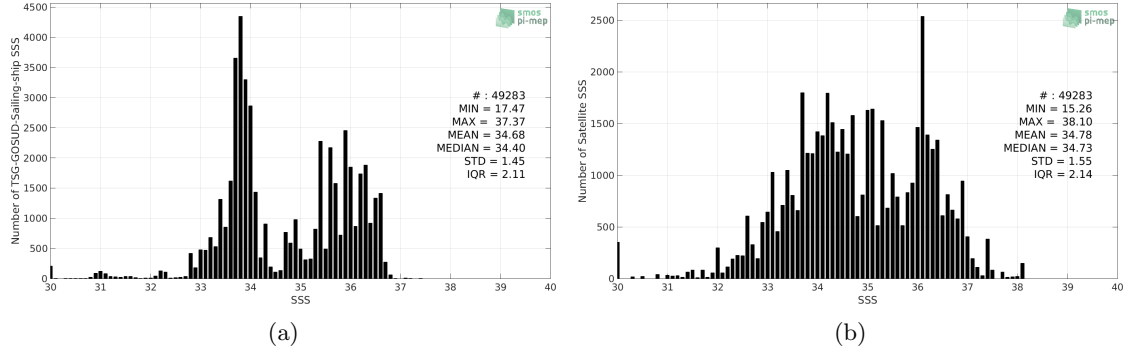
Figure 2: Histograms of SSS from TSG-GOSUD-Sailing-ship (a) and Aquarius-L2-JPL-V5 (b) considering all match-up pairs per bins of 0.1 over the SMOS coastal zone (<800km) 60N-60S Pi-MEP region and for the full satellite product period.
