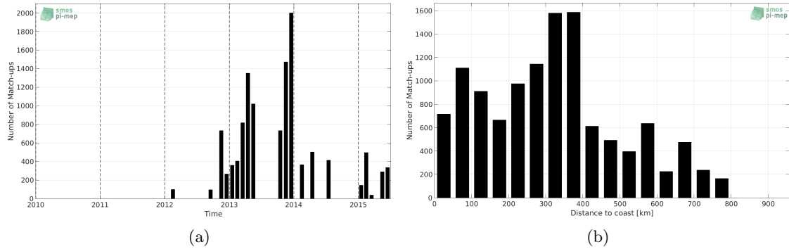
Figure 1: Number of match-ups between TSG-GOSUD-Sailing-ship and Aquarius-L2-JPL-V5 SSS as a function of time (a) and as function of the distance to coast (b) over the SMOS coastal zone (j800km) 60N-60S Pi-MEP region and for the full satellite product period.
