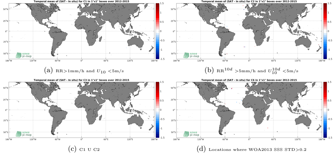
Figure 12: Temporal mean gridded over spatial boxes of size 1^\circ \times 1^\circ of \Delta SSS (Aquarius-L2-JPL-V5 - TSG-GOSUD-Sailing-ship) for 4 different subdatasets corresponding to: RR > 1\text{mm/h} and U_{10} < 5\text{m/s} (a), RR^{10d} > 5\text{mm/h} and U_{10}^{10d} < 5\text{m/s} (b), C1 U C2 (c), Locations where WOA2013 SSS STD > 0.2 (d).
