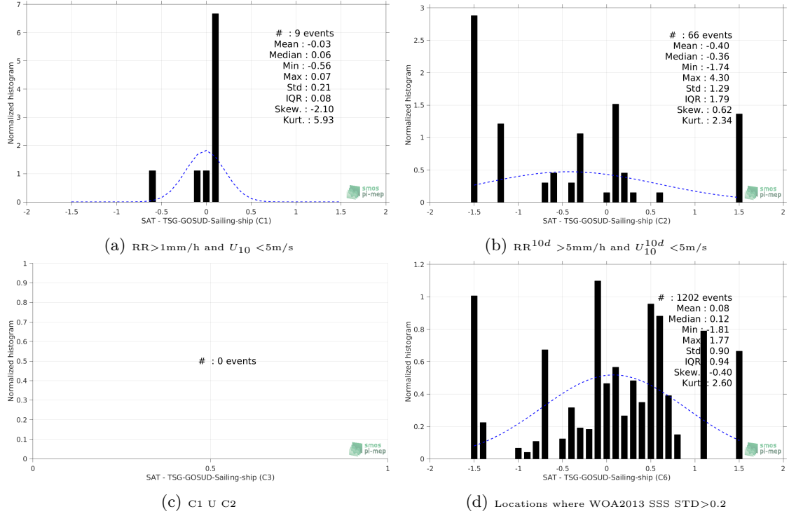
Figure 13: Normalized histogram of \Delta SSS (Aquarius-L2-JPL-V5 - TSG-GOSUD-Sailing-ship) for 6 different subdatasets corresponding to: RR > 1\text{mm/h} and U_{10} < 5\text{m/s} (a), RR^{10d} > 5\text{mm/h} and U_{10}^{10d} < 5\text{m/s} (b), C1 U C2 (c), Locations where WOA2013 SSS STD > 0.2 (d).
