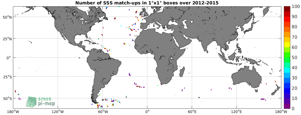
Figure 4: Number of SSS match-ups between TSG-GOSUD-Sailing-ship SSS and the Aquarius-L2-JPL-V5 SSS product for the SMOS coastal zone ( \leq 800\text{km} ) 60N-60S Pi-MEP region over 1^\circ \times 1^\circ boxes and for the full satellite product period.
