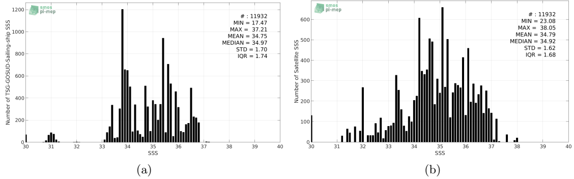
Figure 2: Histograms of SSS from TSG-GOSUD-Sailing-ship (a) and Aquarius-L2-JPL-V5 (b) considering all match-up pairs per bins of 0.1 over the SMOS coastal zone ( \geq 800\text{km} ) 60^\circ\text{N} - 60^\circ\text{S} Pi-MEP region and for the full satellite product period.
