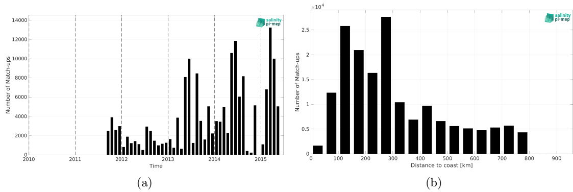
Figure 2: Number of match-ups between TSG (GOSUD-Research-vessel) and Aquarius SSS L2 CAP v5 (JPL) SSS as a function of time (a) and as function of the distance to coast (b) over the SMOS coastal zone (<800km) 60N-60S Pi-MEP region and for the full satellite product period.
