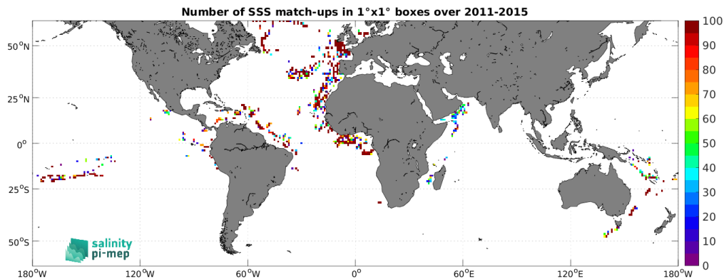
Figure 5: Number of SSS match-ups between TSG (GOSUD-Research-vessel) SSS and the Aquarius SSS L2 CAP v5 (JPL) SSS product for the SMOS coastal zone (<800km) 60N-60S Pi-MEP region over 1^\circ \times 1^\circ boxes and for the full satellite product period.
