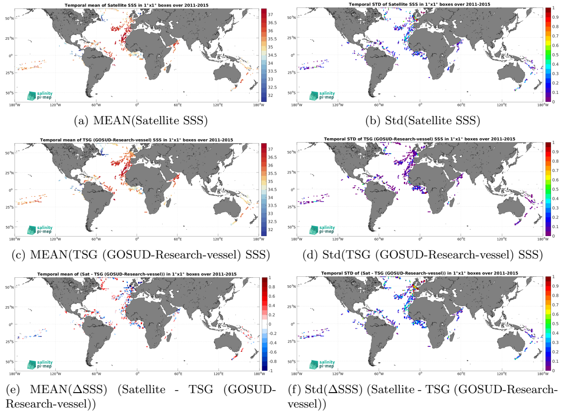
Figure 7: Temporal mean (left) and Std (right) of SSS from Aquarius SSS L2 CAP v5 (JPL) (top), TSG (GOSUD-Research-vessel) (middle), and of \Delta SSS (Satellite - TSG (GOSUD-Research-vessel)). Only match-up pairs are used to generate these maps.
