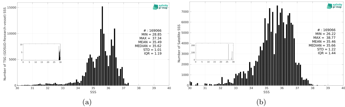
Figure 3: Histograms of SSS from TSG (GOSUD-Research-vessel) (a) and Aquarius SSS L2 CAP v5 (JPL) (b) considering all match-up pairs per bins of 0.1 over the SMOS coastal zone (<800km) 60N-60S Pi-MEP region and for the full satellite product period.
