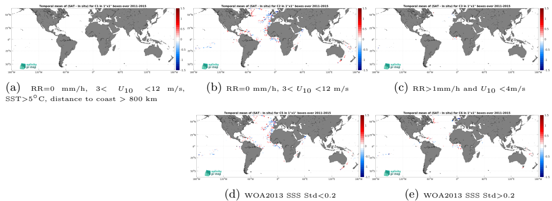
Figure 14: Temporal mean gridded over spatial boxes of size 1^\circ \times 1^\circ of \Delta SSS (Aquarius SSS L2 CAP v5 (JPL) - TSG (GOSUD-Research-vessel)) for 5 different subdatasets corresponding to: RR=0 mm/h, 3 < U_{10} < 12 m/s, SST > 5^\circ\text{C} , distance to coast > 800 km (a), RR=0 mm/h, 3 < U_{10} < 12 m/s (b), RR > 1 mm/h and U_{10} < 4 m/s (c), WOA2013 SSS Std < 0.2 (d), WOA2013 SSS Std > 0.2 (e).
