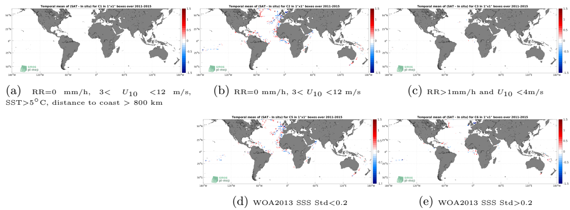
Figure 12: Temporal mean gridded over spatial boxes of size 1^\circ \times 1^\circ of \Delta\text{SSS} (Aquarius SSS L2 CAP v5 (JPL) - TSG (GOSUD-Research-vessel)) for 5 different subdatasets corresponding to:RR=0 mm/h, 3 < U_{10} < 12 m/s, SST >5^\circ\text{C} , distance to coast > 800 km (a), RR=0 mm/h, 3 < U_{10} < 12 m/s (b), RR >1 mm/h and U_{10} < 4 m/s (c), WOA2013 SSS Std <0.2 (d), WOA2013 SSS Std >0.2 (e).
