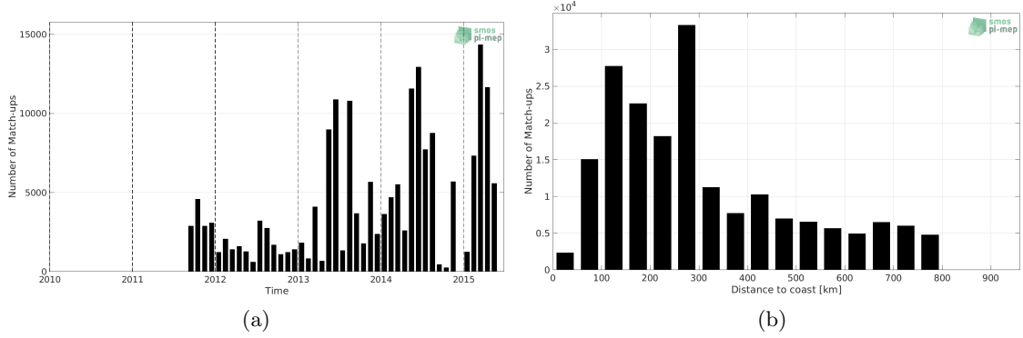
Figure 1: Number of match-ups between TSG (GOSUD-Research-vessel) and Aquarius SSS L2 CAP v5 (JPL) SSS as a function of time (a) and as function of the distance to coast (b) over the SMOS coastal zone (<800km) 60N-60S Pi-MEP region and for the full satellite product period.
