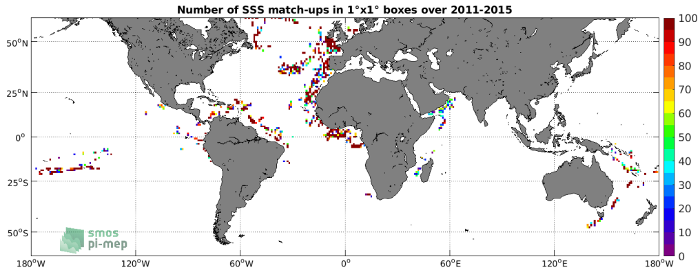
Figure 4: Number of SSS match-ups between TSG (GOSUD-Research-vessel) SSS and the Aquarius SSS L2 CAP v5 (JPL) SSS product for the SMOS coastal zone (<800km) 60N-60S Pi-MEP region over 1^\circ \times 1^\circ boxes and for the full satellite product period.
