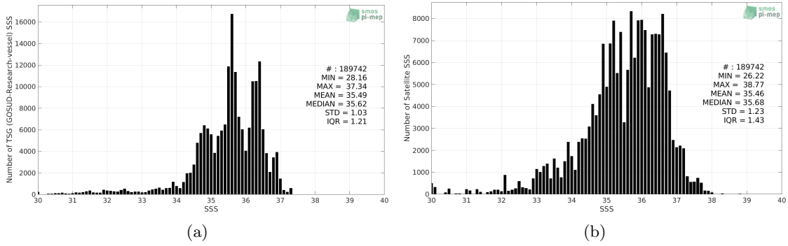
Figure 2: Histograms of SSS from TSG (GOSUD-Research-vessel) (a) and Aquarius SSS L2 CAP v5 (JPL) (b) considering all match-up pairs per bins of 0.1 over the SMOS coastal zone (<800km) 60N-60S Pi-MEP region and for the full satellite product period.
