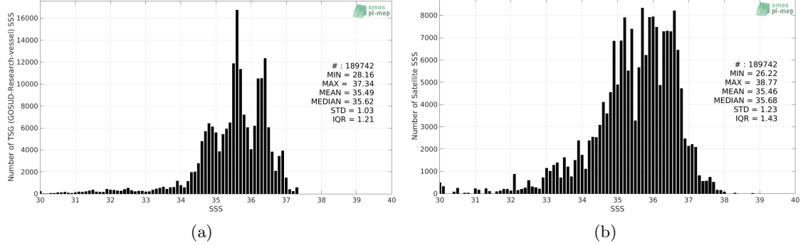
Figure 2: Histograms of SSS from TSG (GOSUD-Research-vessel) (a) and Aquarius SSS L2 CAP v5 (JPL) (b) considering all match-up pairs per bins of 0.1 over the SMOS coastal zone (<800km) 60N-60S Pi-MEP region and for the full satellite product period.
