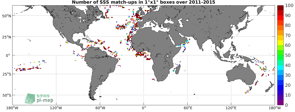
Figure 4: Number of SSS match-ups between TSG (GOSUD-Research-vessel) SSS and the Aquarius SSS L2 CAP v5 (JPL) SSS product for the SMOS coastal zone (<800km) 60N-60S Pi-MEP region over 1°x1° boxes and for the full satellite product period.
