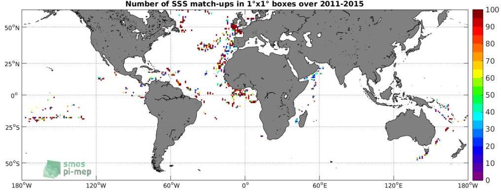
Figure 4: Number of SSS match-ups between TSG-GOSUD-Research-vessel SSS and the Aquarius-L2-JPL-V5 SSS product for the SMOS coastal zone ( \pm 800\text{km} ) 60N-60S Pi-MEP region over 1^\circ \times 1^\circ boxes and for the full satellite product period.
