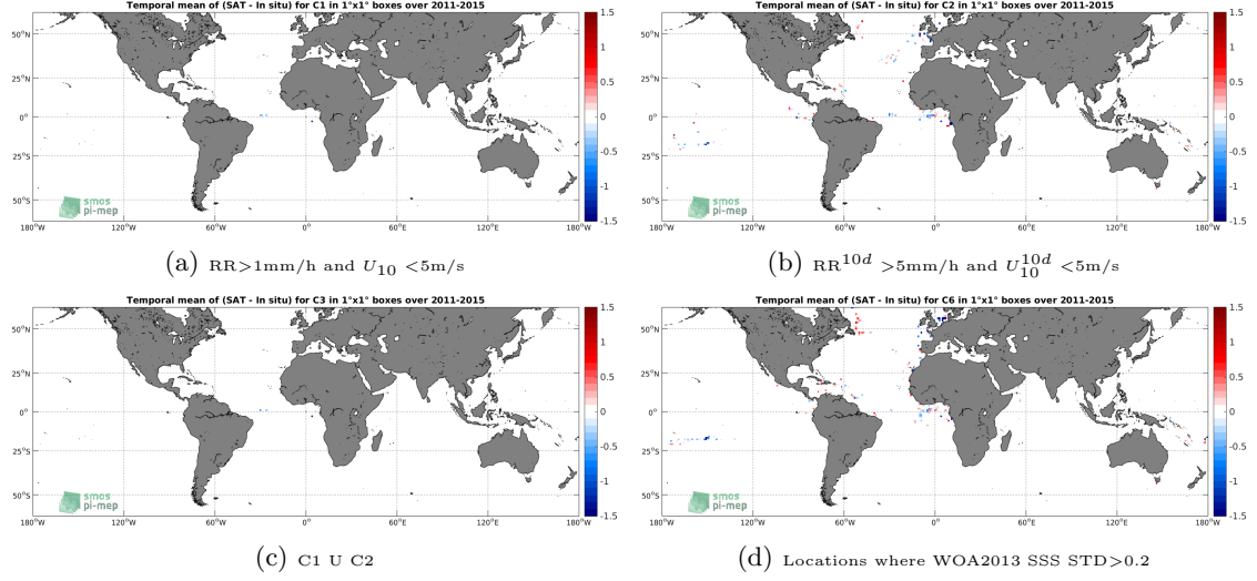
Figure 12: Temporal mean gridded over spatial boxes of size 1^\circ \times 1^\circ of \Delta SSS (Aquarius-L2-JPL-V5 - TSG-GOSUD-Research-vessel) for 4 different subdatasets corresponding to: RR > 1\text{mm/h} and U_{10} < 5\text{m/s} (a), RR^{10d} > 5\text{mm/h} and U_{10}^{10d} < 5\text{m/s} (b), C1 U C2 (c), Locations where WOA2013 SSS STD > 0.2 (d).
