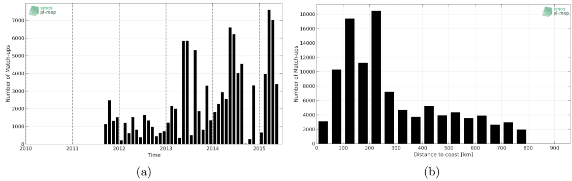
Figure 1: Number of match-ups between TSG-GOSUD-Research-vessel and Aquarius-L2-JPL-V5 SSS as a function of time (a) and as function of the distance to coast (b) over the SMOS coastal zone ( \pm 800 km) 60N-60S Pi-MEP region and for the full satellite product period.
