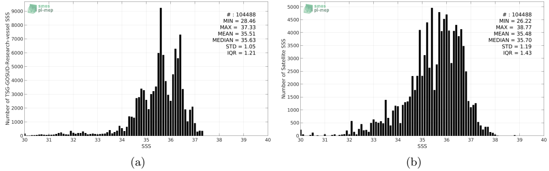
Figure 2: Histograms of SSS from TSG-GOSUD-Research-vessel (a) and Aquarius-L2-JPL-V5 (b) considering all match-up pairs per bins of 0.1 over the SMOS coastal zone ( \geq 800\text{km} ) 60N-60S Pi-MEP region and for the full satellite product period.
