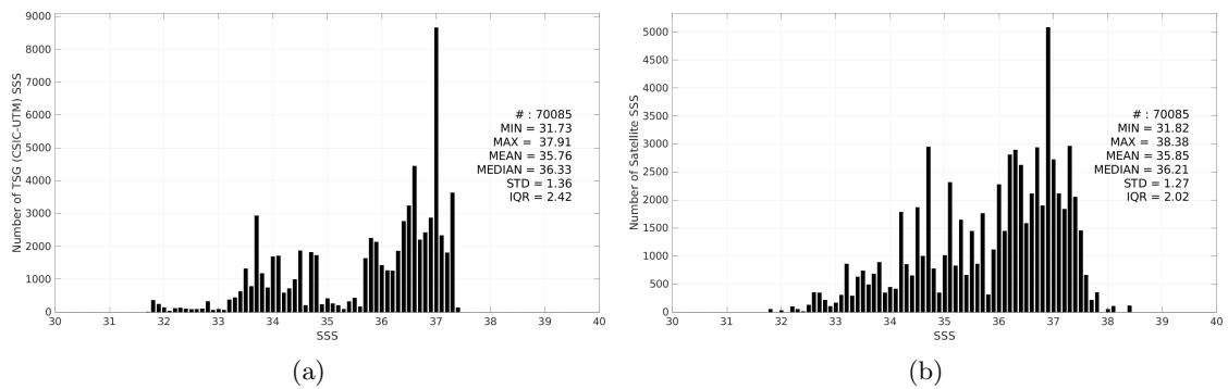
Figure 3: Histograms of SSS from TSG (CSIC-UTM) (a) and Aquarius SSS L2 CAP v5 (JPL) (b) considering all match-up pairs per bins of 0.1 over the SMOS coastal zone (<800km) 60N-60S Pi-MEP region and for the full satellite product period.
