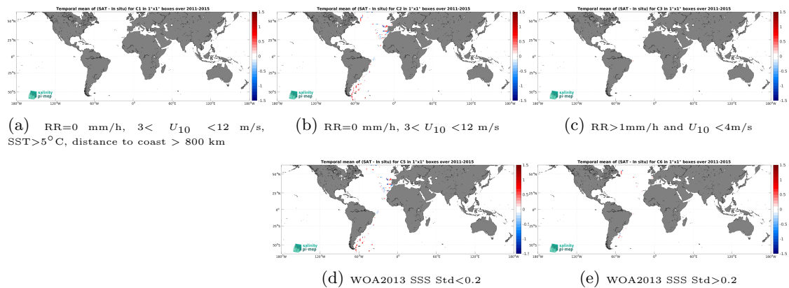
Figure 14: Temporal mean gridded over spatial boxes of size 1^\circ \times 1^\circ of \Delta SSS (Aquarius SSS L2 CAP v5 (JPL) - TSG (CSIC-UTM)) for 5 different subdatasets corresponding to:RR=0 mm/h, 3 < U_{10} < 12 m/s, SST > 5°C, distance to coast > 800 km (a), RR=0 mm/h, 3 < U_{10} < 12 m/s (b), RR > 1mm/h and U_{10} < 4 m/s (c), WOA2013 SSS Std < 0.2 (d), WOA2013 SSS Std > 0.2 (e).
