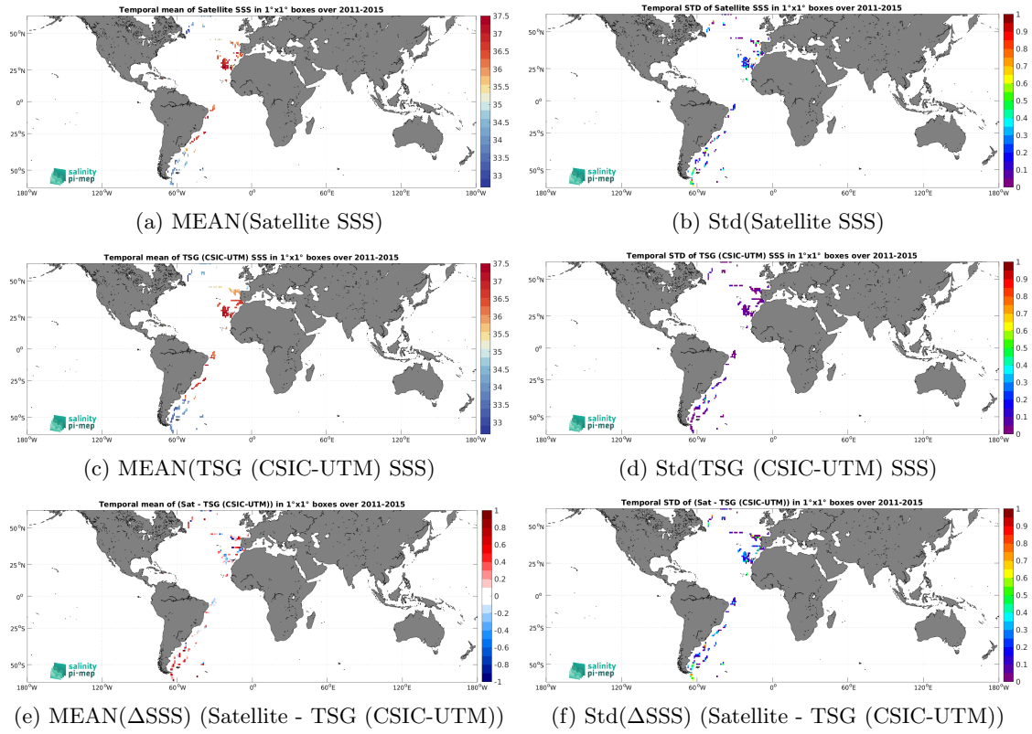
Figure 7: Temporal mean (left) and Std (right) of SSS from Aquarius SSS L2 CAP v5 (JPL) (top), TSG (CSIC-UTM) (middle), and of \Delta SSS (Satellite - TSG (CSIC-UTM)). Only match-up pairs are used to generate these maps.
