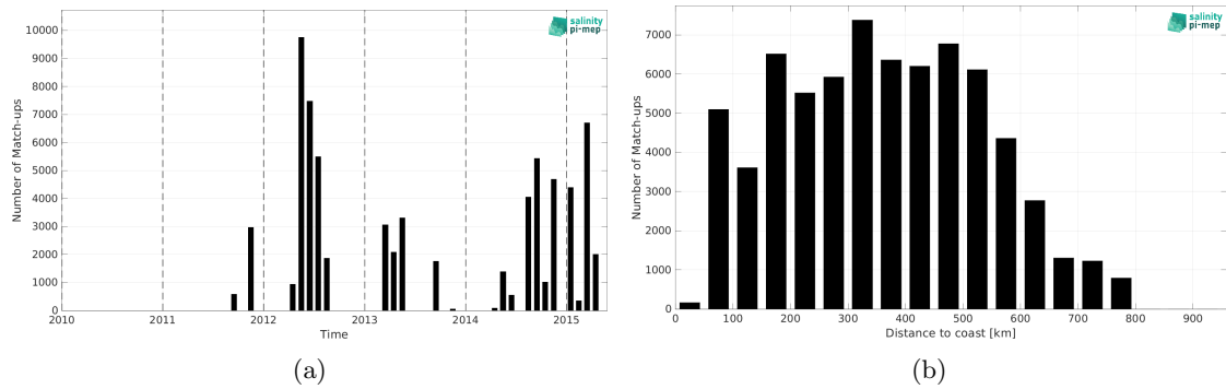
Figure 2: Number of match-ups between TSG (CSIC-UTM) and Aquarius SSS L2 CAP v5 (JPL) SSS as a function of time (a) and as function of the distance to coast (b) over the SMOS coastal zone (<800km) 60N-60S Pi-MEP region and for the full satellite product period.
