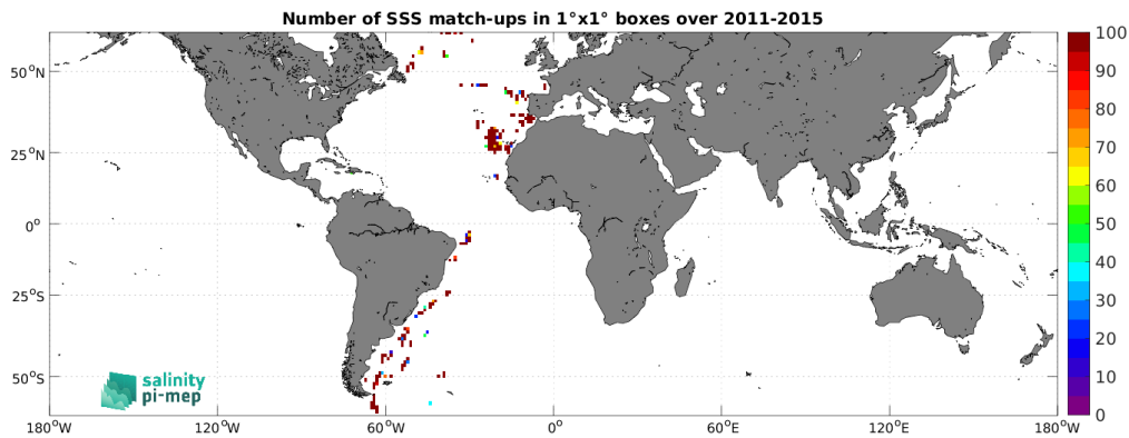
Figure 5: Number of SSS match-ups between TSG (CSIC-UTM) SSS and the Aquarius SSS L2 CAP v5 (JPL) SSS product for the SMOS coastal zone (<800km) 60N-60S Pi-MEP region over 1^\circ \times 1^\circ boxes and for the full satellite product period.
