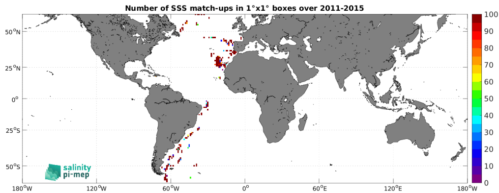
Figure 4: Number of SSS match-ups between TSG (CSIC-UTM) SSS and the Aquarius SSS L2 CAP v5 (JPL) SSS product for the SMOS coastal zone (<800km) 60N-60S Pi-MEP region over 1^\circ \times 1^\circ boxes and for the full satellite product period.
