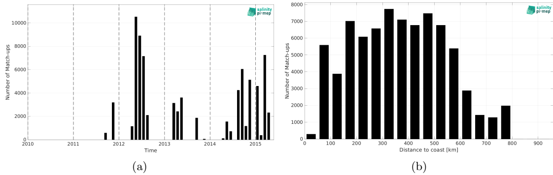
Figure 1: Number of match-ups between TSG (CSIC-UTM) and Aquarius SSS L2 CAP v5 (JPL) SSS as a function of time (a) and as function of the distance to coast (b) over the SMOS coastal zone (<800km) 60N-60S Pi-MEP region and for the full satellite product period.
