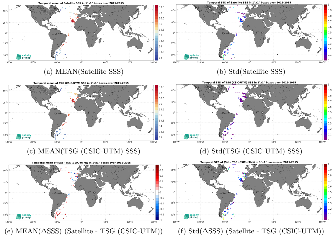
Figure 6: Temporal mean (left) and Std (right) of SSS from Aquarius SSS L2 CAP v5 (JPL) (top), TSG (CSIC-UTM) (middle), and of \Delta SSS (Satellite - TSG (CSIC-UTM)). Only match-up pairs are used to generate these maps.
