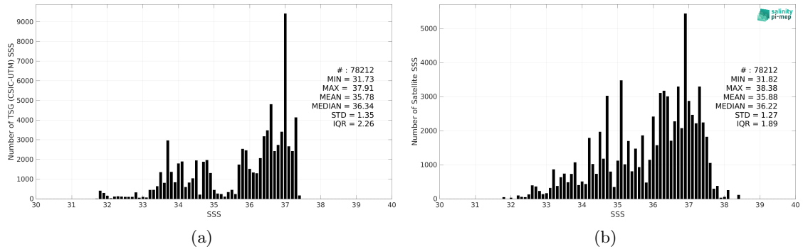
Figure 2: Histograms of SSS from TSG (CSIC-UTM) (a) and Aquarius SSS L2 CAP v5 (JPL) (b) considering all match-up pairs per bins of 0.1 over the SMOS coastal zone (<800km) 60N-60S Pi-MEP region and for the full satellite product period.
