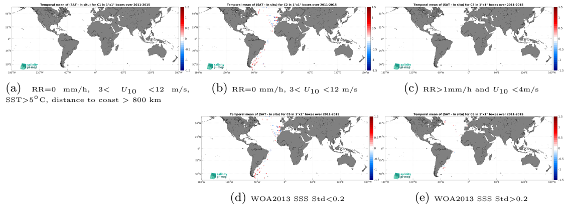
Figure 12: Temporal mean gridded over spatial boxes of size 1^\circ \times 1^\circ of \Delta SSS (Aquarius SSS L2 CAP v5 (JPL) - TSG (CSIC-UTM)) for 5 different subdatasets corresponding to:RR=0 mm/h, 3 < U_{10} < 12 m/s, SST >5^\circ\text{C} , distance to coast > 800 km (a), RR=0 mm/h, 3 < U_{10} < 12 m/s (b), RR >1 mm/h and U_{10} < 4 m/s (c), WOA2013 SSS Std <0.2 (d), WOA2013 SSS Std >0.2 (e).
