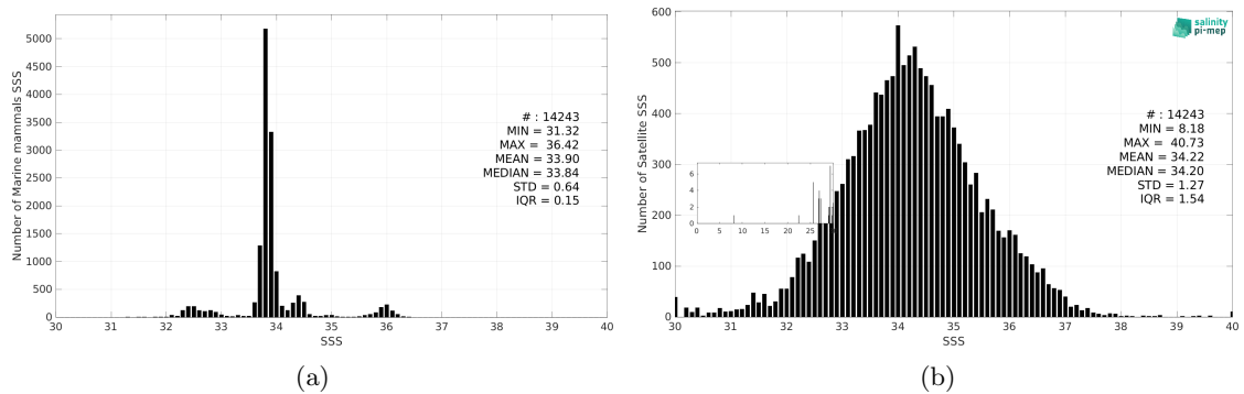
Figure 3: Histograms of SSS from Marine mammals (a) and Aquarius SSS L2 CAP v5 (JPL) (b) considering all match-up pairs per bins of 0.1 over the SMOS coastal zone (<800km) 60N-60S Pi-MEP region and for the full satellite product period.
