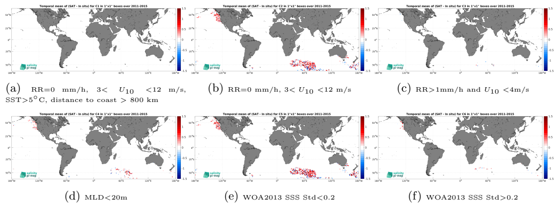
Figure 14: Temporal mean gridded over spatial boxes of size 1^\circ \times 1^\circ of \Delta SSS (Aquarius SSS L2 CAP v5 (JPL) - Marine mammals) for 6 different subdatasets corresponding to:RR=0 mm/h, 3 < U_{10} < 12 m/s, SST >5^\circ\text{C} , distance to coast > 800 km (a), RR=0 mm/h, 3 < U_{10} < 12 m/s (b), RR >1 mm/h and U_{10} < 4 m/s (c),MLD <20 m (d),WOA2013 SSS Std <0.2 (e),WOA2013 SSS Std >0.2 (f).
