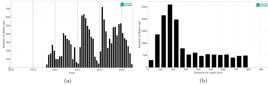
Figure 2: Number of match-ups between Marine mammals and Aquarius SSS L2 CAP v5 (JPL) SSS as a function of time (a) and as function of the distance to coast (b) over the SMOS coastal zone (<800km) 60N-60S Pi-MEP region and for the full satellite product period.
