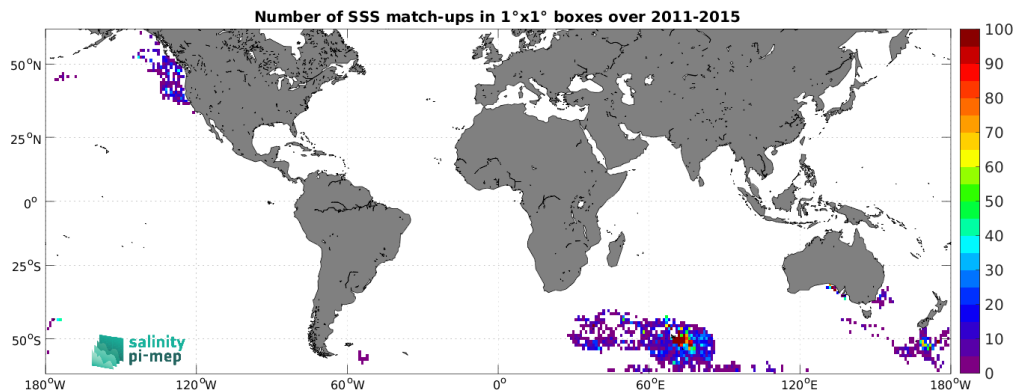
Figure 5: Number of SSS match-ups between Marine mammals SSS and the Aquarius SSS L2 CAP v5 (JPL) SSS product for the SMOS coastal zone (<800km) 60N-60S Pi-MEP region over 1°x1° boxes and for the full satellite product period.
