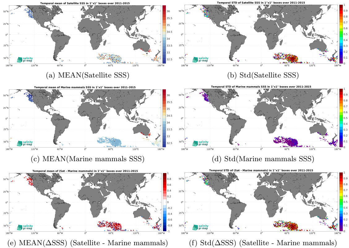
Figure 7: Temporal mean (left) and Std (right) of SSS from Aquarius SSS L2 CAP v5 (JPL) (top), Marine mammals (middle), and of \Delta SSS (Satellite - Marine mammals). Only match-up pairs are used to generate these maps.
