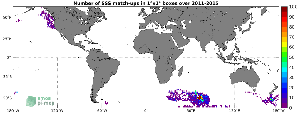
Figure 4: Number of SSS match-ups between Sea mammals SSS and the Aquarius SSS L2 CAP v5 (JPL) SSS product for the SMOS coastal zone (<800km) 60N-60S Pi-MEP region over 1°x1° boxes and for the full satellite product period.
