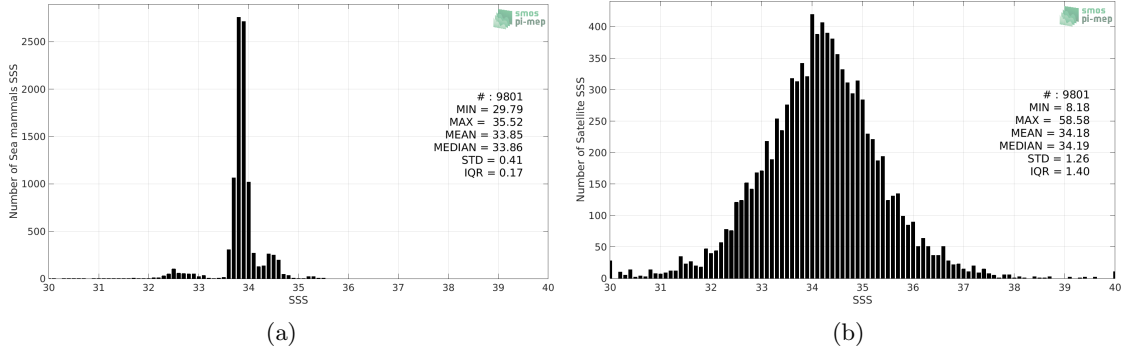
Figure 2: Histograms of SSS from Sea mammals (a) and Aquarius SSS L2 CAP v5 (JPL) (b) considering all match-up pairs per bins of 0.1 over the SMOS coastal zone (<800km) 60N-60S Pi-MEP region and for the full satellite product period.
