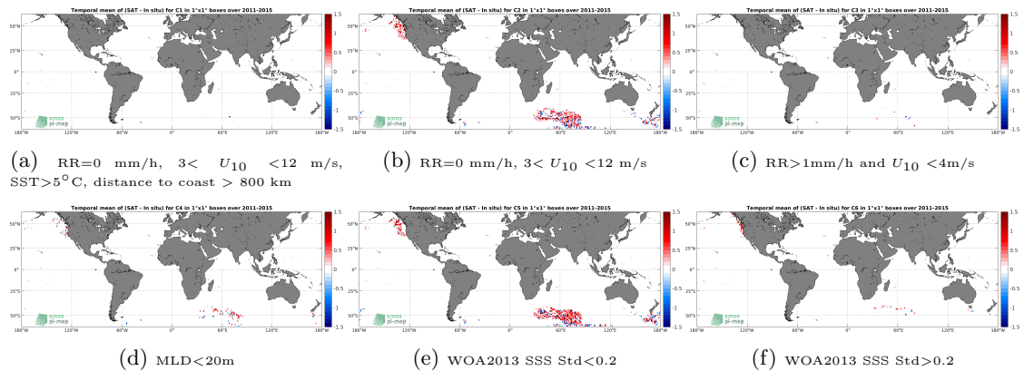
Figure 12: Temporal mean gridded over spatial boxes of size 1^\circ \times 1^\circ of \Delta SSS (Aquarius SSS L2 CAP v5 (JPL) - Sea mammals) for 6 different subdatasets corresponding to:RR=0 mm/h, 3 < U_{10} < 12 m/s, SST > 5^\circ\text{C} , distance to coast > 800 km (a), RR=0 mm/h, 3 < U_{10} < 12 m/s (b), RR > 1 mm/h and U_{10} < 4 m/s (c),MLD < 20 m (d),WOA2013 SSS Std < 0.2 (e),WOA2013 SSS Std > 0.2 (f).
