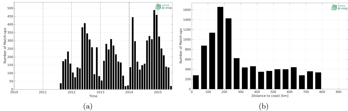
Figure 1: Number of match-ups between Sea mammals and Aquarius SSS L2 CAP v5 (JPL) SSS as a function of time (a) and as function of the distance to coast (b) over the SMOS coastal zone (<800km) 60N-60S Pi-MEP region and for the full satellite product period.
