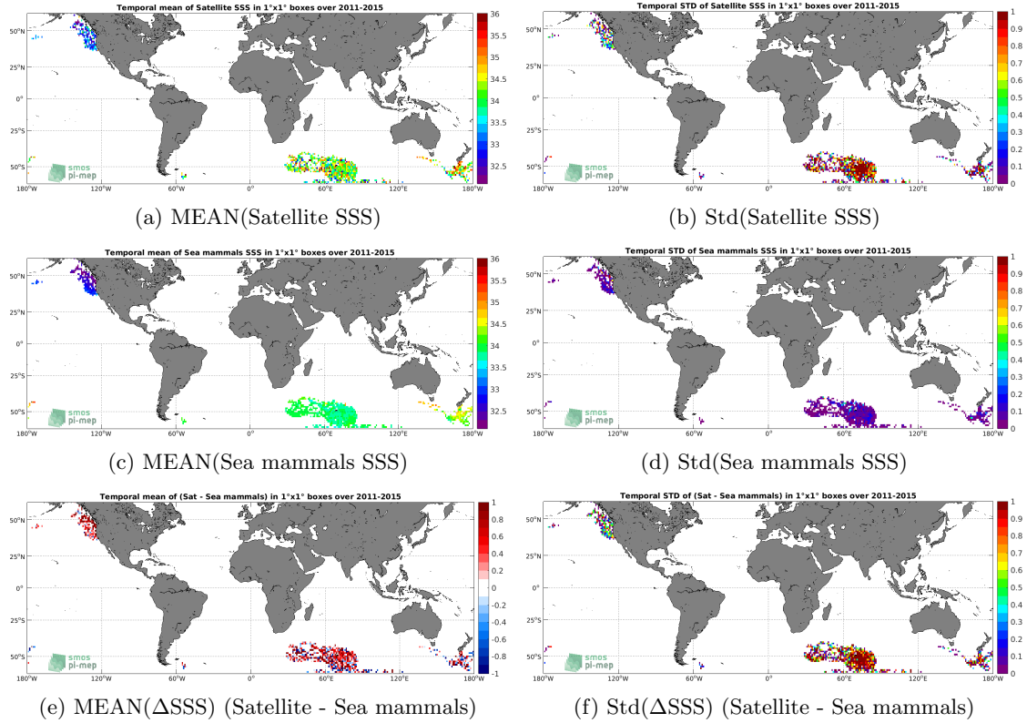
Figure 6: Temporal mean (left) and Std (right) of SSS from Aquarius SSS L2 CAP v5 (JPL) (top), Sea mammals (middle), and of \Delta SSS (Satellite - Sea mammals). Only match-up pairs are used to generate these maps.
